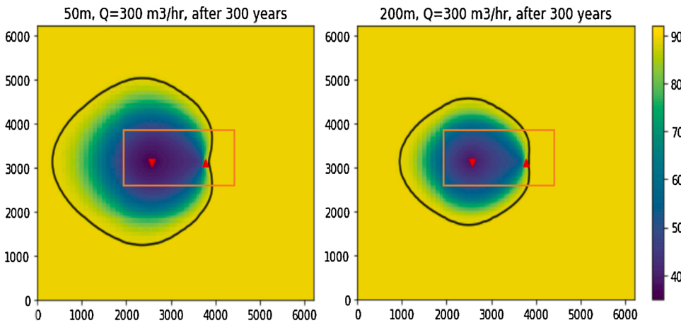
Fig. 4. The temperature distribution at the bottom of the top confining layer after 300 years of production, with on the left a reservoir of 50 m thick, on the right a reservoir of 200 m thick. The black contour line indicates the 89 °C boundary. The red triangle pointing down and up represent the injection and production well, respectively. The orange box indicates the representative volume boundary. (For interpretation of the references to colour in this figure legend, the reader is referred to the web version of this article.)
