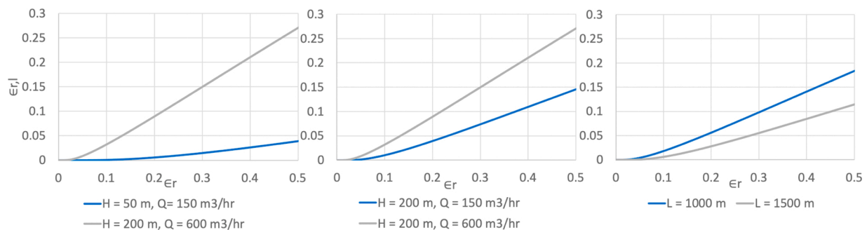
Fig. 9. Laterally recharged heat \epsilon_{rl} against the total recharged heat \epsilon_r . The figures show from left to right the effect of reservoir thickness, production rate and well spacing.
