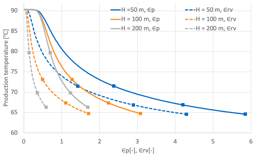
Fig. 3. The effect of reservoir thickness on recharge. The produced and vertically recharged energy content against the production temperature. Measured for a reservoir of H = 50, 100 & 200 m during 300 years of production with a constant production rate of 300 \text{ m}^3/\text{h} for all cases. Each marker on the line represents 100 years of production.
