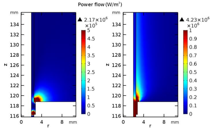
Fig. 4. Time average power flow (0 to 0.02 s) in the positive radial direction (left) and positive z direction (right). Argon model at the same conditions given in Figure 1.
