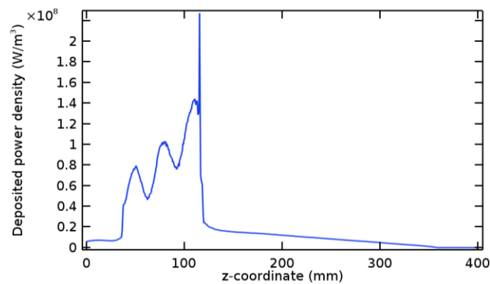
Fig. 3. Deposited power density profile at steady state (0.006 s). Argon model at the same conditions given in Figure 1. The power density peak seen at 116 mm is related to the intense electric field formed at this point due to the Surfatron design (see small protrusion at the bottom of Figure 4).
