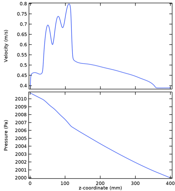
Fig. 2. Velocity (top) and pressure (bottom) profiles at steady state (0.016 s). Argon model at the same conditions given in Figure 1.
