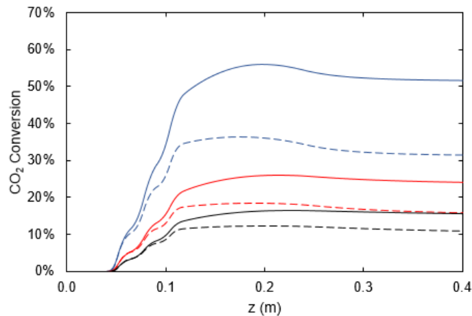
Fig. 9. CO 2 conversion as a function of the axial position in the reactor for 100 (blue), 200 (red) and 300 sccm (black). Results ignoring the vibrationally enhanced CO 2 dissociation are shown in dashed lines. The solid lines correspond to the full model, including the fictitious species CO 2 * and its reactions. In all cases, the CO 2 recombination from x = 0.4 m until the measuring device located at x = 2.9 m is estimated to be less than 1%.
