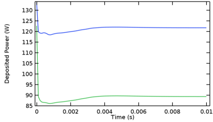
Fig. 5. Deposited microwave power over time. Blue: total deposited power, green: deposited power inside the Surfatron body (at high power densities). Argon model at the same conditions given in Figure 1.
