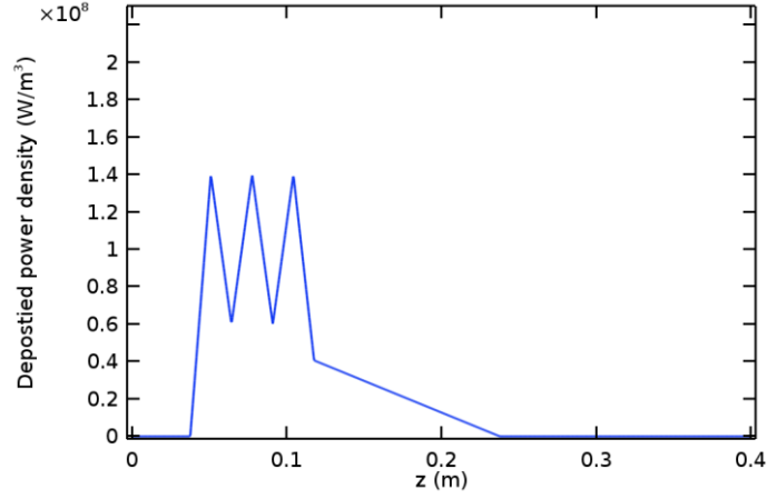
Fig. 8. Deposited power density profile for the CO 2 model. Refer to Figure 3 for the power density profile obtained with the Argon model.
