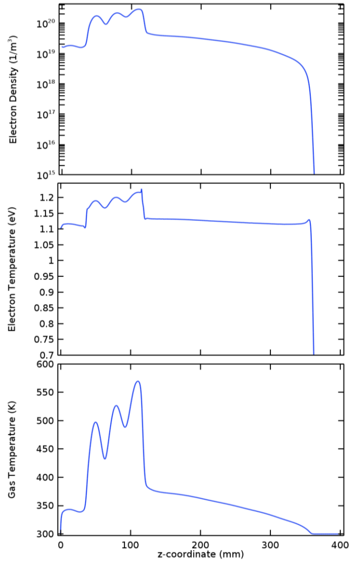
Fig. 1. Electron density (top), electron temperature (middle) and gas temperature (bottom) profiles at steady state (0.006 s). These profiles were obtained using the Argon model 13 for a flowrate of 300 sccm, inlet temperature of 300 K, inner wall temperature of 300 K, outlet pressure of 20 mbar and a microwave power input of 150 W. (1 eV \approx 11600 K)
