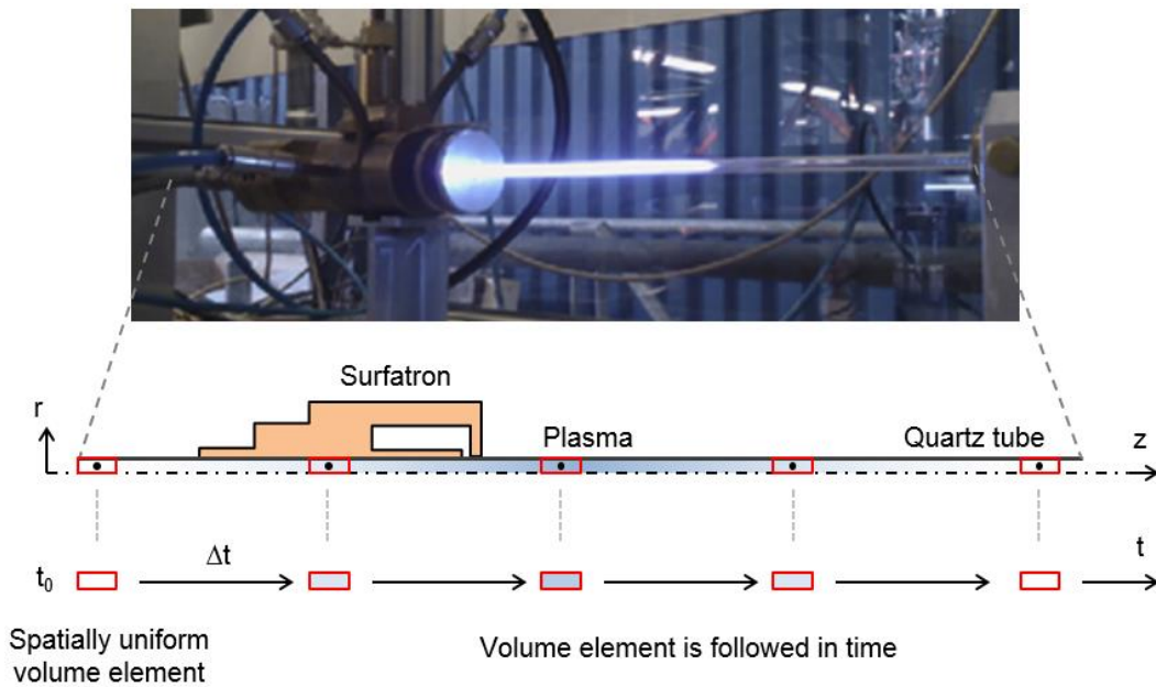
Fig. 6. Approach for modelling \text{CO}_2 dissociation in a microwave plasma reactor. Top: Experimental setup used in 12 , middle: Two-dimensional axisymmetric sketch of the reactor 13 , bottom: Approach used in this work.
