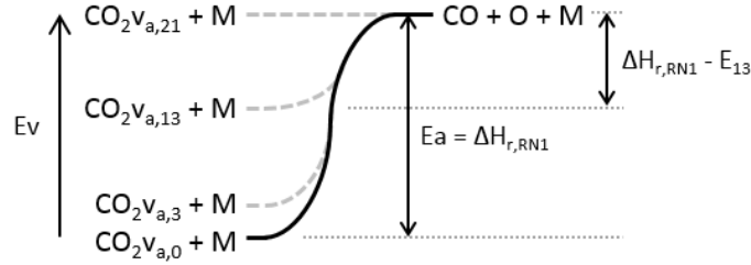
Fig. 7. Enthalpy change of the \text{CO}_2 dissociation reaction RN1 for selected asymmetric vibrational levels. The energy barrier of the reaction decreases as the vibrational energy increases up to the dissociation limit of 5.5 eV.
