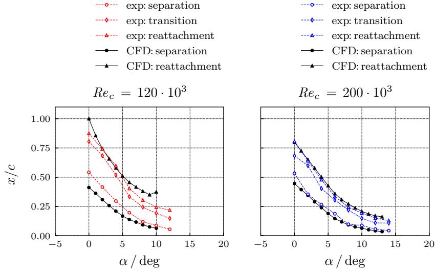
Figure 6: Experimental and computational separation behavior at different Reynolds numbers on the suction side of a NACA0018.
