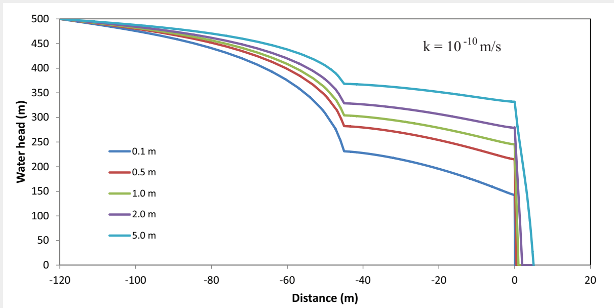
Figure 3.5: Pore pressure head distribution along the tunnel for different sealing lengths, top: k=10^{-9} m/s for the backfill hydraulic conductivity; bottom: k=10^{-10} m/s for the backfill hydraulic conductivity.
