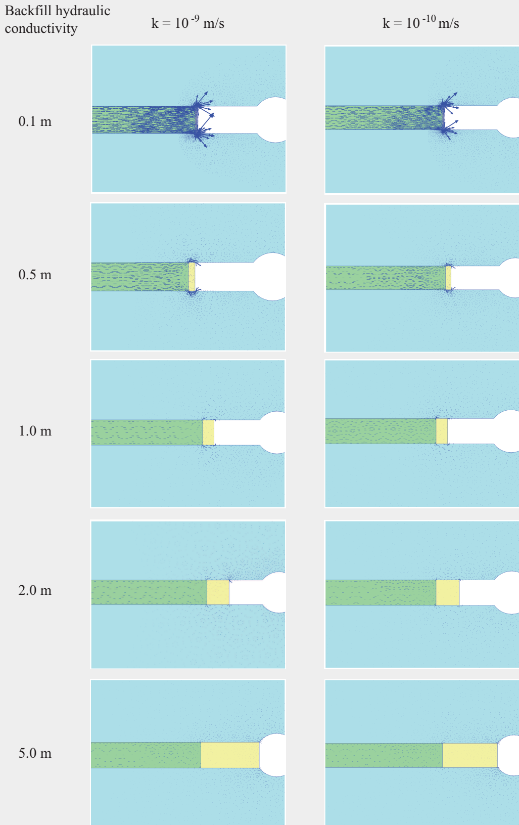
Figure 3.8: Velocity distribution near the plug for different sealing lengths, left: k=10^{-9} m/s for the backfill hydraulic conductivity; right: k=10^{-10} m/s for the backfill hydraulic conductivity.
