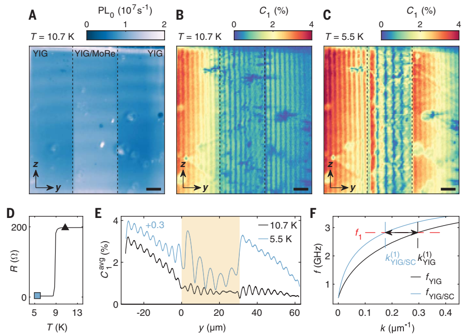
Fig. 2. Magnetic resonance imaging of spin waves above and below the superconducting transition temperature. (A) Spatial map of the NV photoluminescence \text{PL}_0 in the absence of microwaves, showing the MoRe strip (between the vertical dashes). Scale bar, 10 \mu\text{m} . (B and C) Spatial maps of the NV electron spin resonance contrast C_1 above (B) and below (C) the superconducting transition temperature of T_c = 8.7 \text{ K} at T = 10.7 and 5.5 \text{ K} , respectively. The Au, which excites spin waves, is located just outside the left edge of the imaged area. Above T_c , the wavelength is unaffected by the MoRe strip; below T_c , it is lengthened. (D) DC resistance R of the MoRe strip as a function of temperature T , with markers indicating the resistance of the film during the measurements of (B) triangle and (C) square. (E) Data from (B) and (C) averaged over the z direction, with the MoRe strip indicated by yellow shading. (F) Calculated spin-wave dispersion f_{\text{YIG}}(k) for bare YIG, and f_{\text{YIG/SC}}(k, \lambda_L) for YIG, covered by a superconducting film with London penetration depth \lambda_L = 400 \text{ nm} . The superconductor shifts the dispersion upwards by f_{\text{SC}}(k, \lambda_L) , which manifests as a reduction in the wave number at NV frequency f_1 from k_{\text{YIG}}^{(1)} to k_{\text{YIG/SC}}^{(1)} , indicated by the dashed lines.
