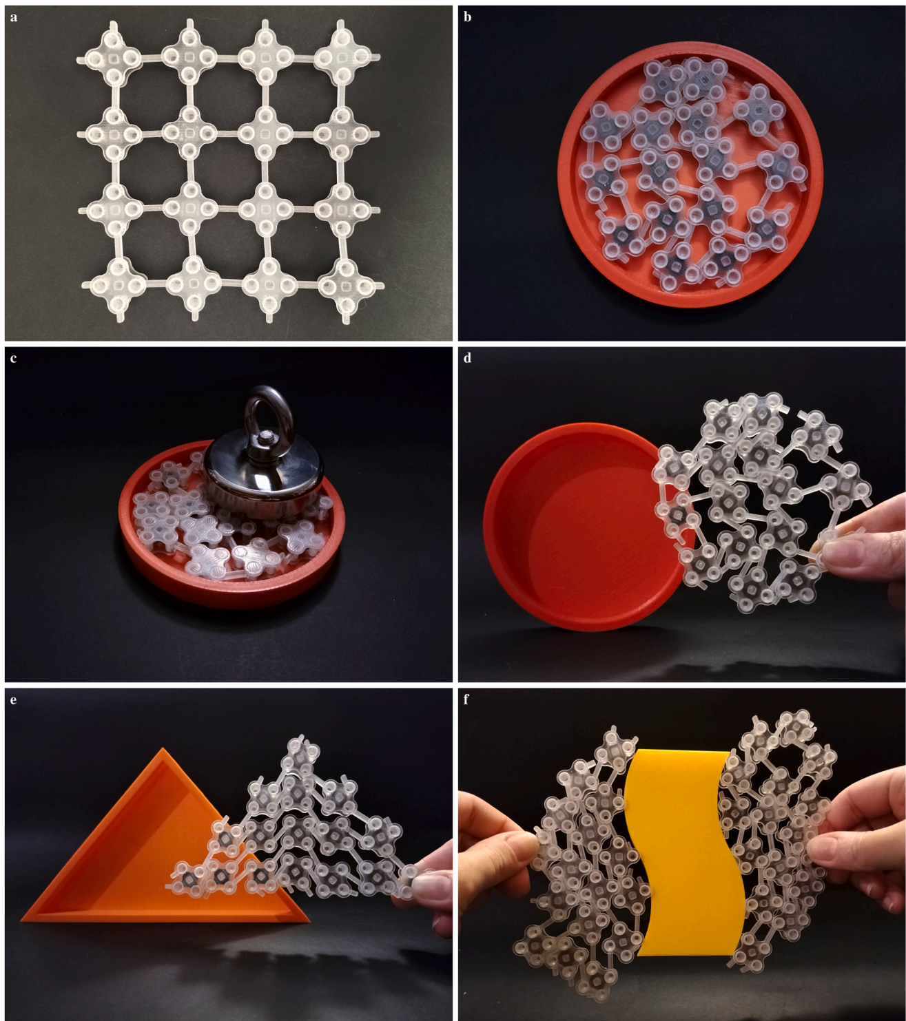
Fig. 6. The final design of the in-plane shape morphing magnetic locking structures. The structure included ferromagnetic locking rings (MEX-TRB/P [40]) that are depicted in grey and transparent elements (MJT-UV/P [40]). a) The assembled structure prior to morphing. b) The structure after morphing into a circular shape. c) Shape locking was achieved by a magnetic field. d) The locked structure maintains its acquired shape. e) Different target shapes, such as a triangle, can also be attained. f) A potential application is the grasping of objects.
