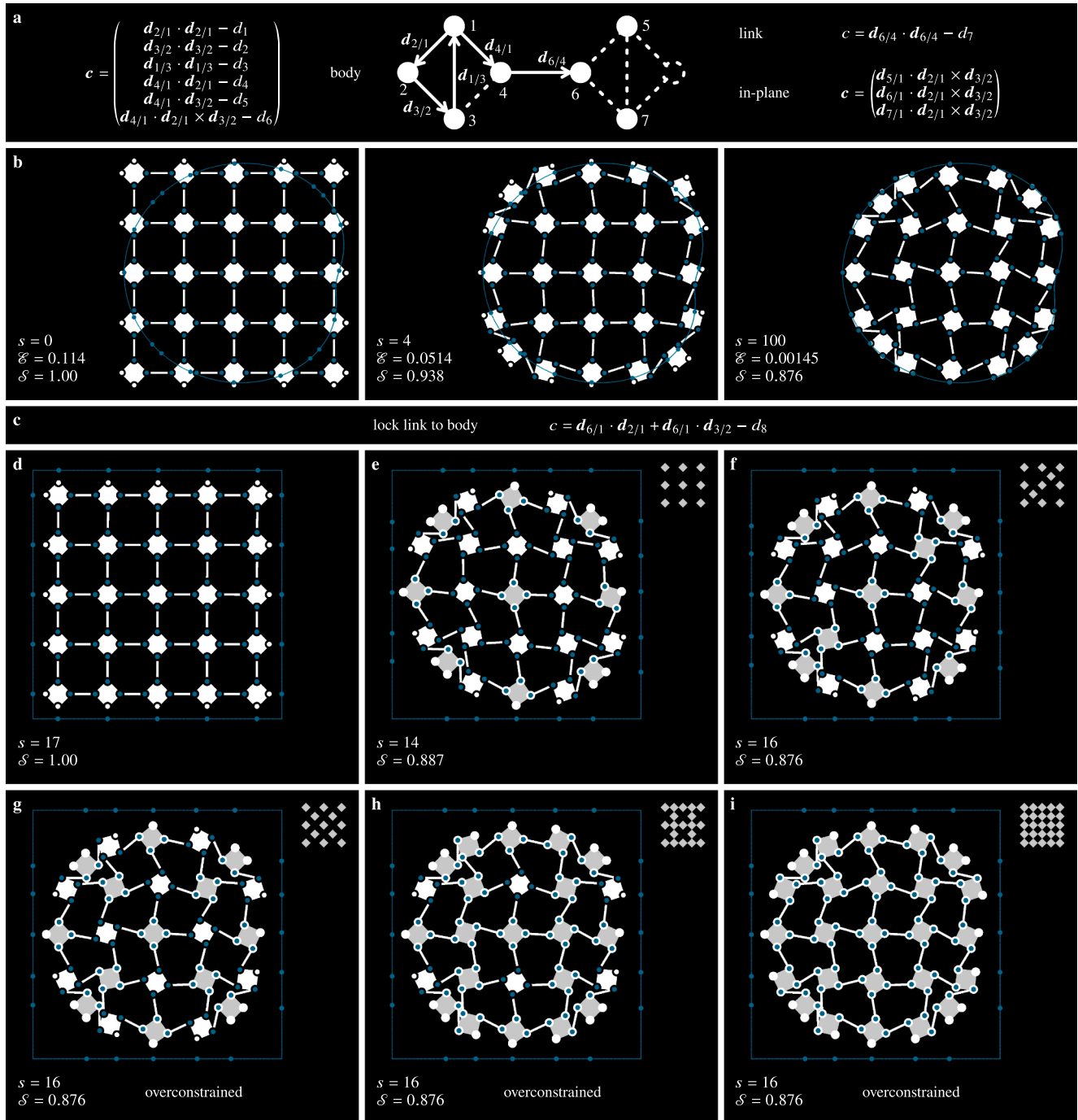
Fig. 4. Simulation of shape-morphing and shape-locking using a multibody kinematic system approach and different distributions of actively locked elements. a) Nodes (white circles) and constraints \mathbf{c} , comprised of vectors \mathbf{d} and constants d , define the structure. b) Combining a sufficient number of these nodes and constraints results in a network of rigid bodies (white squares) and rigid links (white lines) connected via hinges. Each simulation proceeds through multiple steps, s , during which the peripheral nodes move toward the desired shape (green line), minimizing the distance error \mathcal{E} between the node and the nearest point (green dot) on the target shape. A shape factor \mathcal{S} was introduced to quantify the current shape relative to its initial shape. The position of nodes at various steps in this process are depicted. c) After the deformation, DoF were removed by applying additional constraints at specific locations. d)–i) Final states in an effort to return the structure to its original state, using a square target shape and altering the distribution of the locked bodies (grey squares). A locked body restricted all its attached links from rotating relative to that specific body which, in certain instances, may result in an over-constrained system. (For interpretation of the references to colour in this figure legend, the reader is referred to the web version of this article.)
