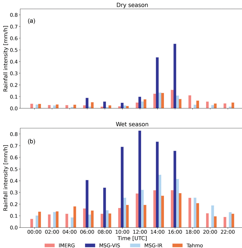
Figure 2. Spatially and temporally averaged daily cycle of precipitation according to TAHMO, IMERG, MSG-IR and MSG-VIS. The spatial average is based on all MSG pixels and TAHMO stations that fall within an IMERG pixel. (a) Dry season; (b) wet season. All observations, i.e. both wet and dry moments, are included. The x-axis ticks indicate the beginning of each time interval.
