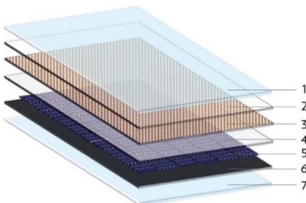
Figure 5: Panel composition: 1-Front Glass; 2-Clear interlayer; 3-Colour and texture filter; 4-Clear interlayer; 5-Monocrystalline PV cell matrix; 6-Back interlayer; 7-Back glass (Source CSEM).
