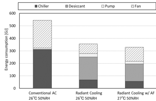
Figure 18: Comparison of estimated energy consumption between different type of air-conditioning system for the cooling in Tokyo
