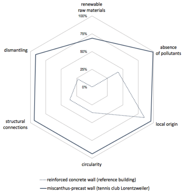
Figure 5: The “spider network diagram” compares a miscanthus-precast wall with a concrete wall
