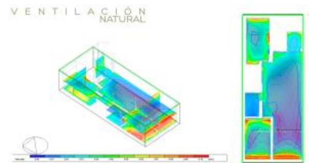
Figure 7: Natural ventilation: indoor air speed (source: Archiwizard Analysis)
