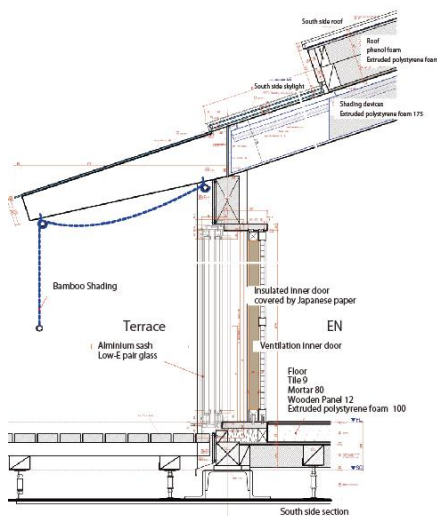
Figure 8: Detail of the top light windows and other devices.
