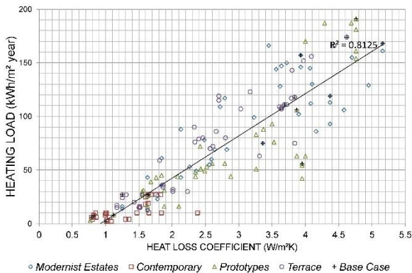
Figure 7: Scatter plot showing the relationship between HLC and Heating Load for all case studies.
