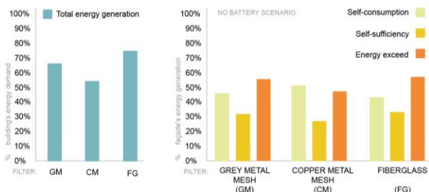
Figure 8: Building energy simulation results from different BIPV panels (Source : LAST).
