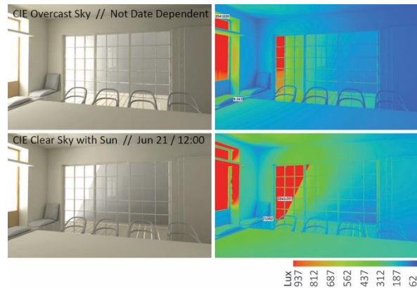
Figure 3. Illuminance image-based and false color visualizations for the Dining-Study space. Source [1].
