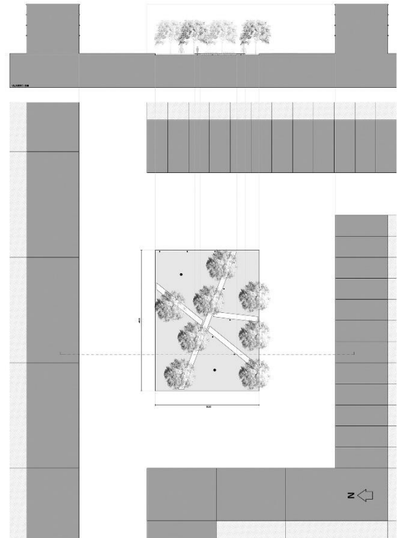
Figure 7: REALCOOL prototype POND EW.
