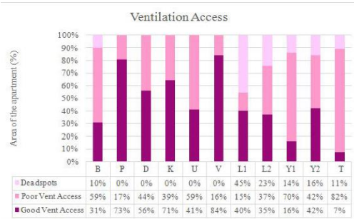
Figure 12: Ventilation access- SW Baseline
