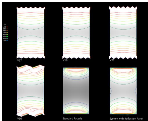
Figure 6: Showing the result of the fourth test of variants V17, V19 and V21 (above three). V56, Standard Façade and the façade with system of reflection plate on the lower three.
