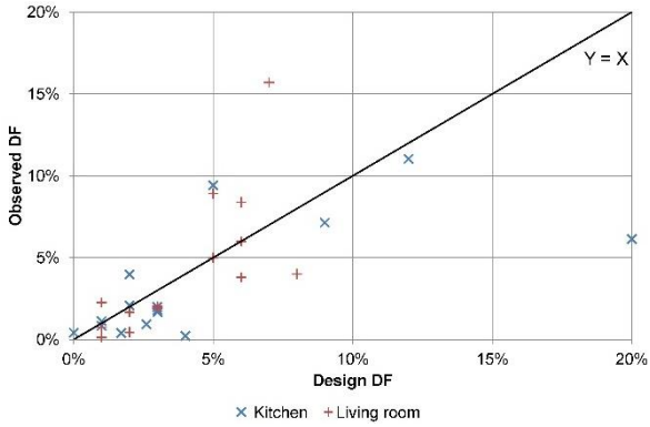
Figure 2: Scatter plot showing Design Values DF vs. Observed DF in kitchens and living rooms of the sixteen case studies
