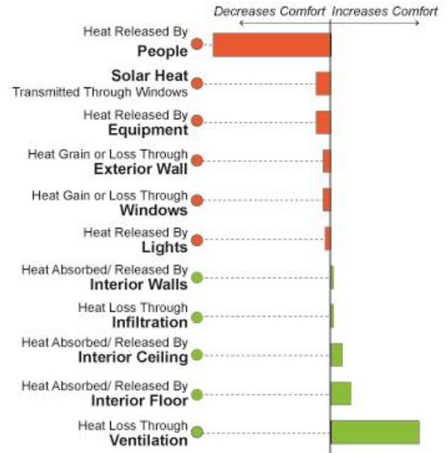
Figure 3: Comfort Load Factors (Degree To Which A Particular Load Is Pushing The Temperature Of A Space Towards The Middle Of The Comfort Zone Or Away From It ) For Bottom Floor Classroom with Suite of Improvements
