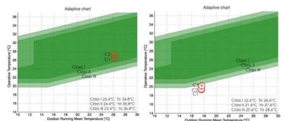
Figures 7 and 8: Adaptive Chart of Santiago and Constanza School Classrooms from Left to Right.
