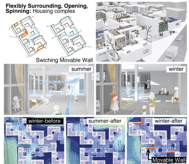
Figure 9b: Simulation of Wind Environment Control by Partitions
