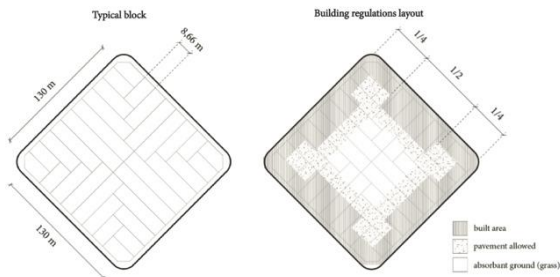
Figure 2: Typical block and plot layout, and building block formation according to building and planning regulations [6]
