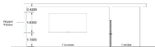
Figure 13: Schools Classroom Original Design Section Detail
