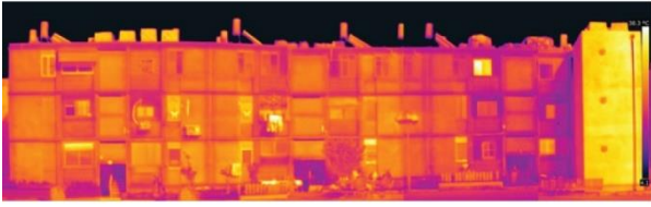
Figure 6: Thermal photo of the Sderot building at 15:00 on a winter day before renovation (photo: Wolfgang Motzafi-Haller)
