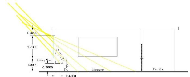
Figure 15: Schools Classroom Section Detail with Additional Wall Zone.
