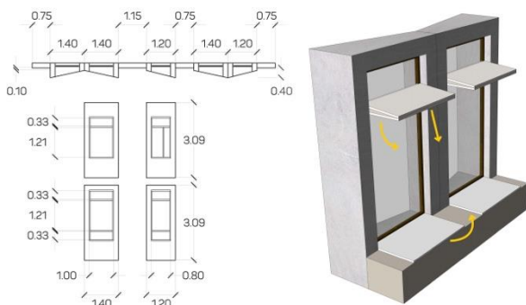
Figure 5: (left) shows the modular insulated timber panel system and window layout; (right) shows the adjustable lightshelf and nightshutter design. Source [1]
