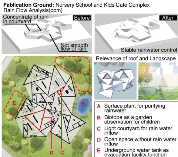
Figure 8: Simulation of Rainflow for Roof Design and Landscape
