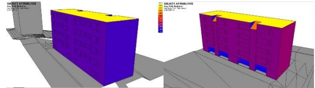
Figure 4: Solar radiation during a summer day on the north-west façade of the Migdal Hahemek building (right) and on the south-east façade (left)
