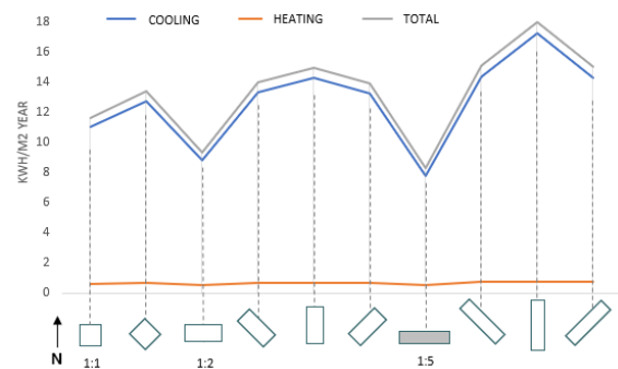
Figure 2: Energy demands for volumes with different shapes and orientations (Source: Author)
