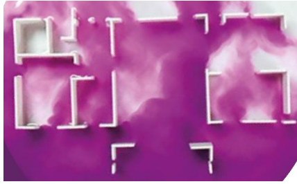
Figure 10: Removal of north wall - SW WIA
