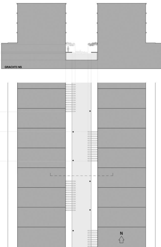
Figure 4: REALCOOL prototype CANAL3 NS.
