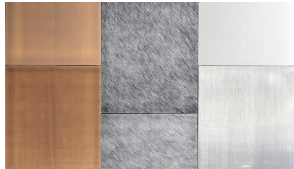
Figure 6: CSEM's BIPV panels. They integrate different filters and different glass treatments. From left to right: Copper metal mesh (can generate 110 W/m 2 ), Fibreglass (can generate 155 W/m 2 ) and Grey metal mesh (can generate up to 120 W/m 2 ) (Source: LAST).
