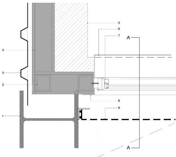
Figure 13: Wall detail drawing.
