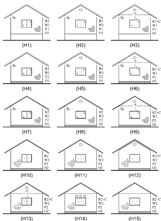
Figure 3: Model of ventilation scenarios in the study
