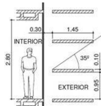
Figure 6: Schematic section of COPAN through north and south orientations.
