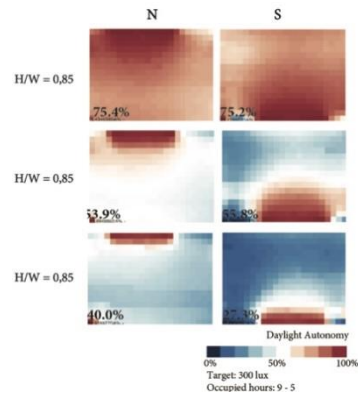
Figure 6: Daylight Autonomy according to H/W ratios (Source: DIVA for Rhino)
