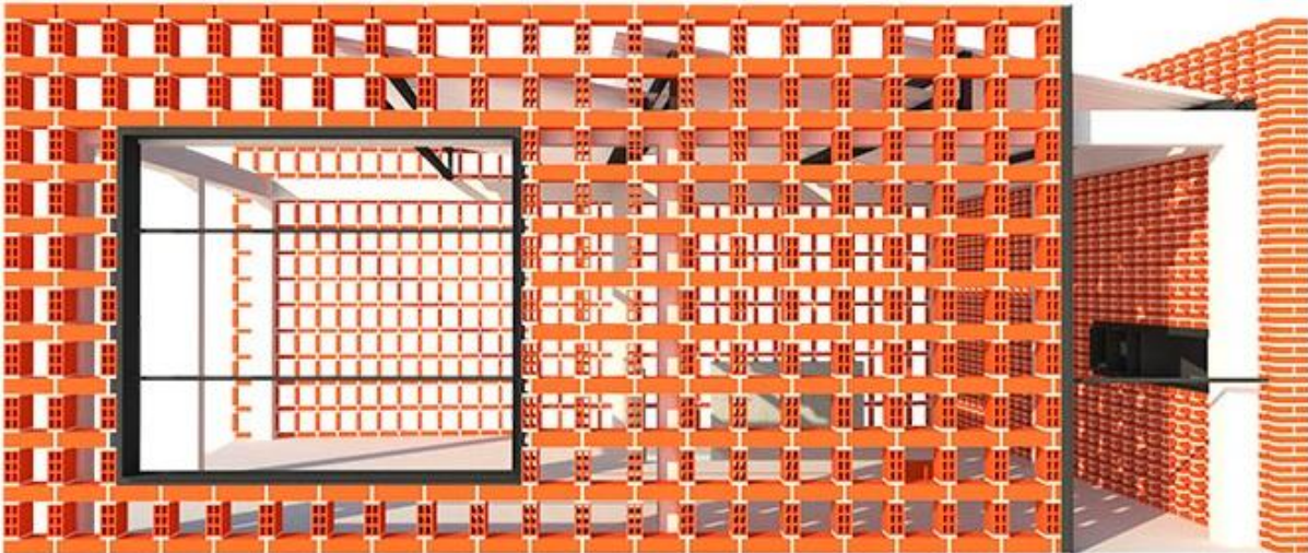
Figure 10: (Third outcome) Digital model of the 1:1 prototype, featuring the Northern façade.
