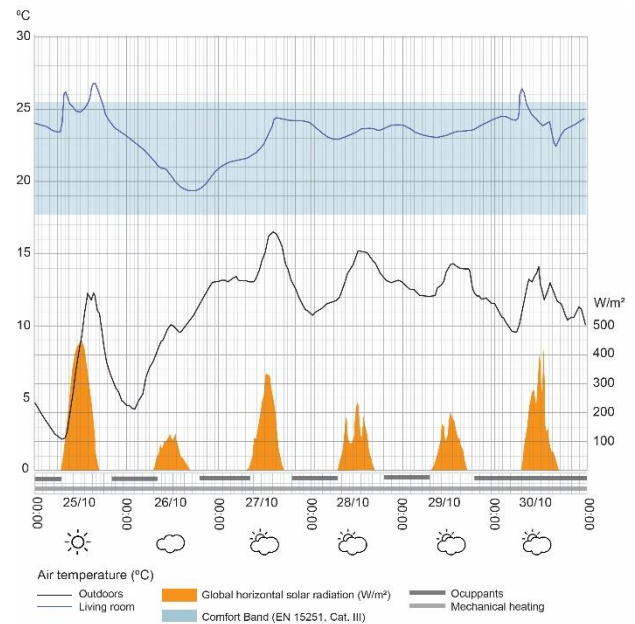
Figure 4: Datalogger results from Highpoint I. The dwelling was monitored during October 2010. The heating system was in intermittent operation (after 5).
