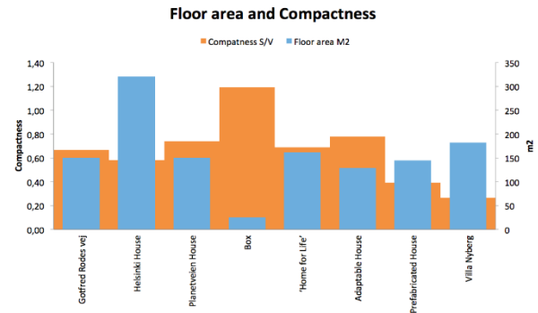
Figure 4: Floor area and Compactness (expressed as Surface to Volume ratio; lower value = more compact).
