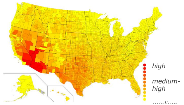
Figure 7: Passive evaporative cooling applicability (I). Determined from CH x [DBT-WBT].
