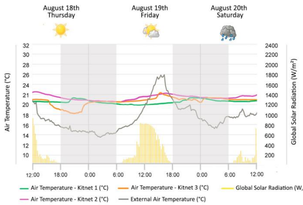
Figure 9: Measurements of dry bulb air temperature during cool days (August 2016) in the case studies with external temperatures and global solar radiation on the horizontal surface.
