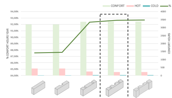
Figure 3: Evaluation of building's shape optimization during thermal comfort times (source: Author)
