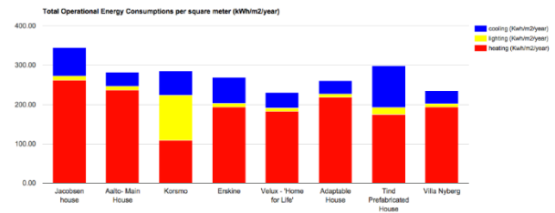
Figure 14: Simulated Operational Energy Use Intensity.
