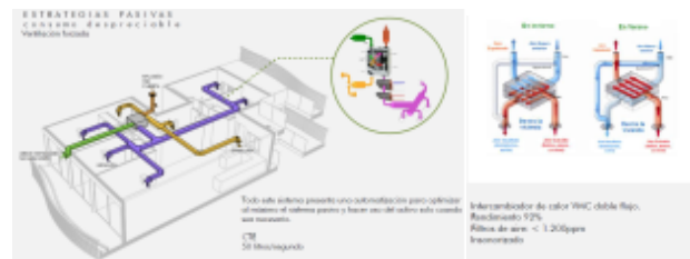
Figure 9: System for recovering heat energy through ventilation with a VCM Heat Exchanger, with a dual flow system and an efficiency level of 92%.
