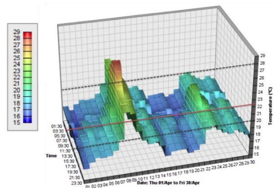
Figure 10: Constanza Dry Resultant Temperatures During the Month of April.
