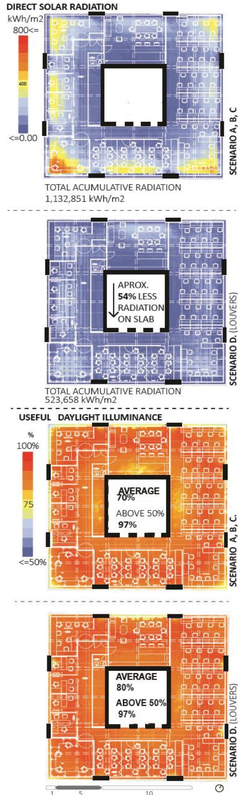
Figure 13. Comparative diagrams of 6 th floor showing the effects of external solar control "louvers" on the transmitted direct solar radiation hitting the slab (thermal mass), upper diagrams, and on the UDI, lower diagrams. (after grasshopper, ladybug and radiance)
