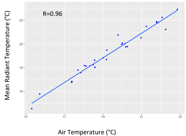
Figure 3: Correlation between air temperature and mean radiant temperature, measured by the industry standard Swema thermal comfort equipment. With trend line and 95% confidence interval (blue shaded area).
