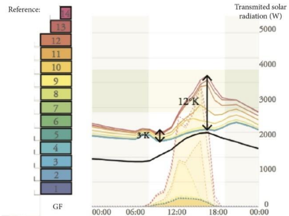
Figure 3: Performance of North oriented apartments on a typical winter day in Buenos Aires (Source: Collo, 2016). [3]
