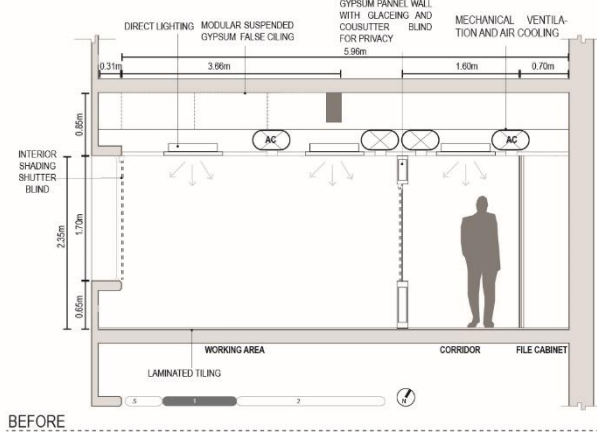
Figure 2: Typical section of studied floor - general construction details before the refurbishment.
