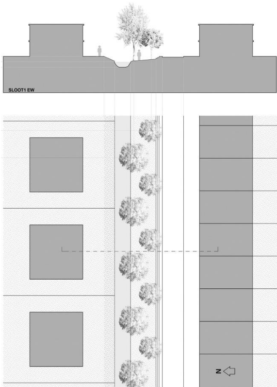
Figure 6: REALCOOL prototype DITCH1 EW.
