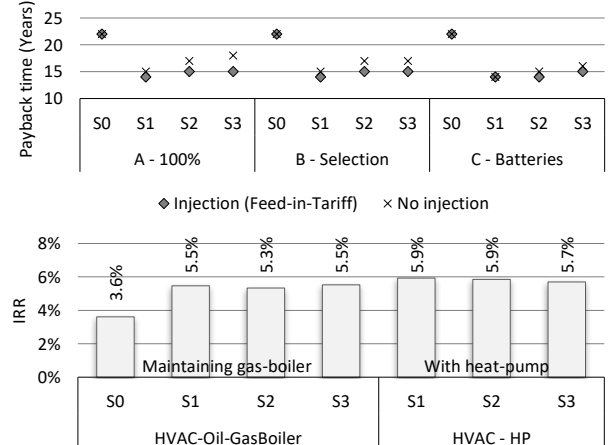
Figure 8: Life-Cycle Cost analysis (LCC) results in terms of payback time (top) and internal rate of return (IRR) (bottom).
