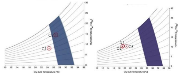
Figures 5 and 6: Psychrometric Chart of Santiago and Constanza School Classrooms from Left to Right
