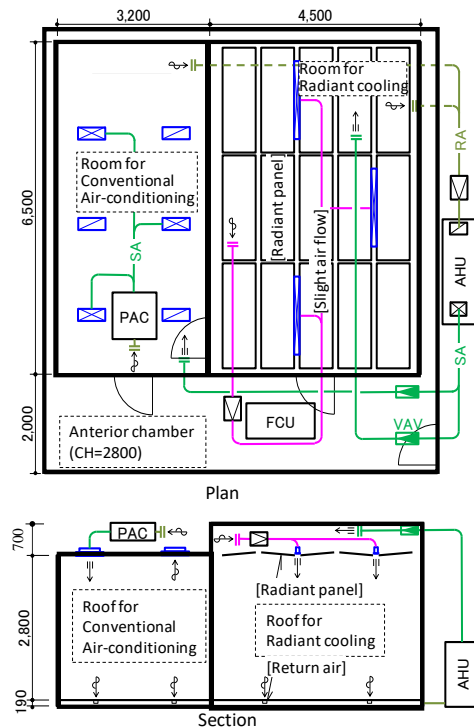
Figure 3: Diagram of mock-up experimental room
