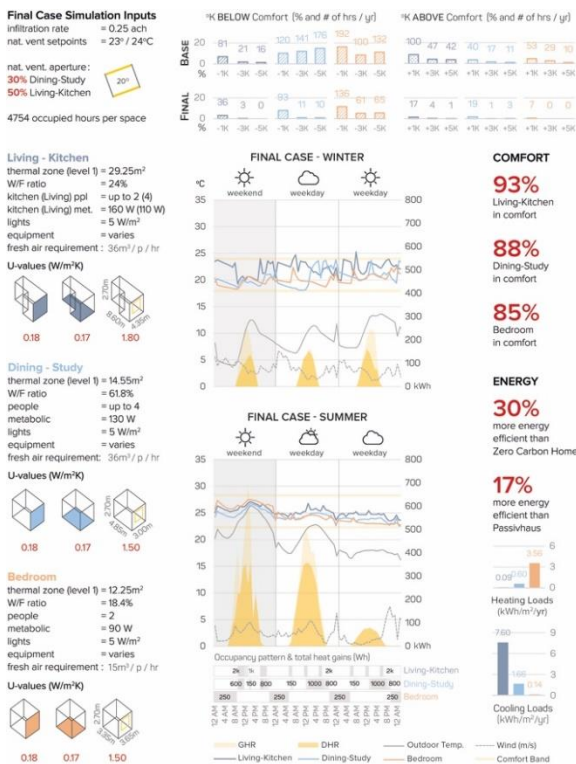
Figure 8: Final case thermal analysis results and energy loads from the infill prototype. Source [1].
