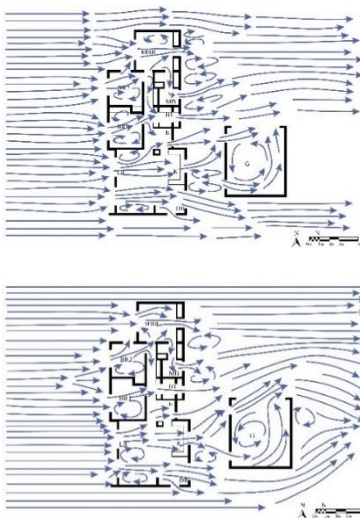
Figure 3: Top: Flow diagram from smoke chamber test from Boutet (1987). Bottom: Flow diagram from water table experiment
