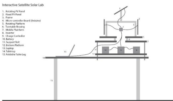
Figure 1: Diagram of the Interactive Satellite Solar Lab.
