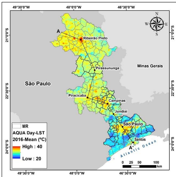
Figure 6: Mean Land Surface Temperature (°C) - Metropolitan Regions, Urban Agglomerations and Connections of the State of São Paulo.
