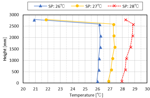
Figure 8: Vertical temperature distribution at the different set point temperatures before occupation.
