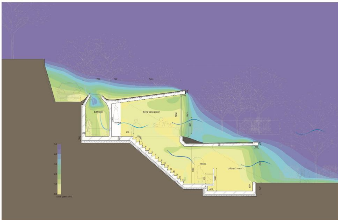
Figure 7: Section (wind simulation).
