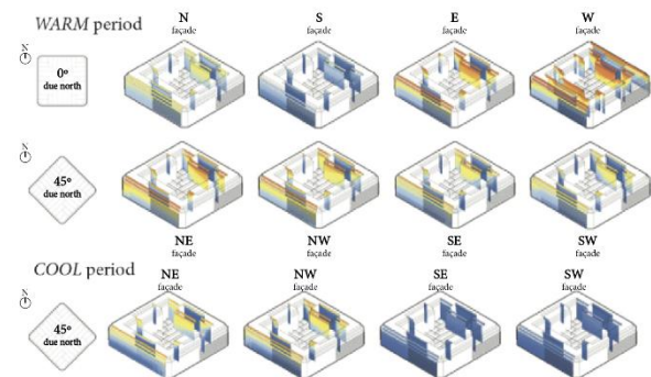
Figure 4: Extract from an extensive solar radiation analysis through different block orientations, densities and configurations (both regulated and irregular), for Buenos Aires, during warm and cool periods (Source: HoneyBee). [1]
