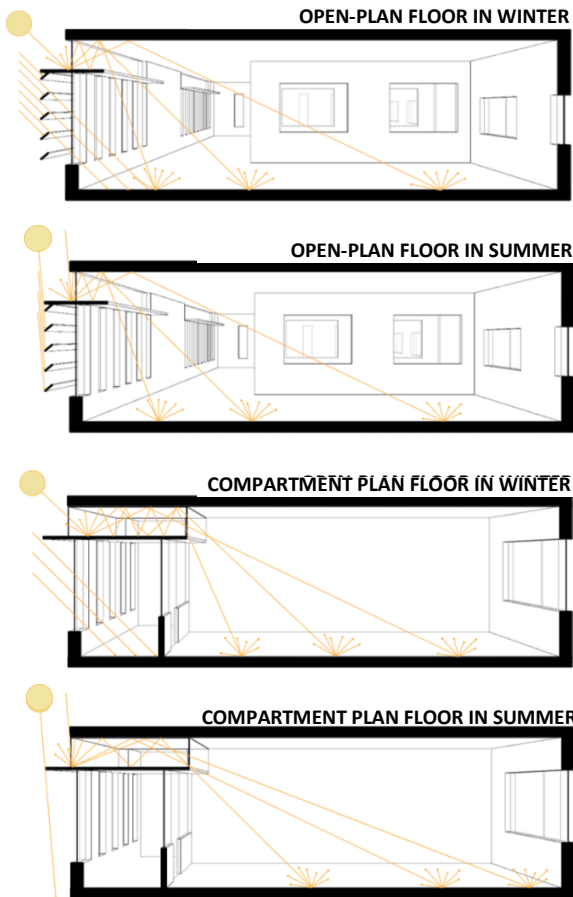
Figure 6: strategies for natural lighting and solar control (Source: Author)
