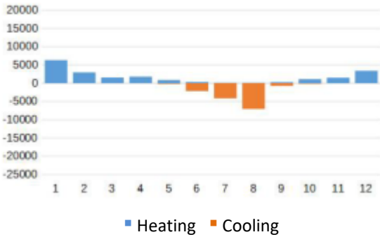
Figure 10: Monthly energy demand expressed in kWh. Heating demand: 12,47kWh/m 2 year. Cooling demand: 10,34kWh/m 2 year.
