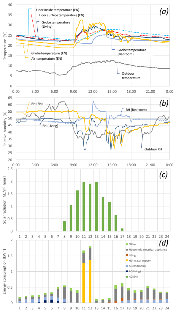
Figure 17: Results of environmental factors and electric consumption on 24 th November, a sunny day. (a) Globe, air and surface temperatures, (b) relative humidity, (c) solar radiation and (d) energy consumption.
