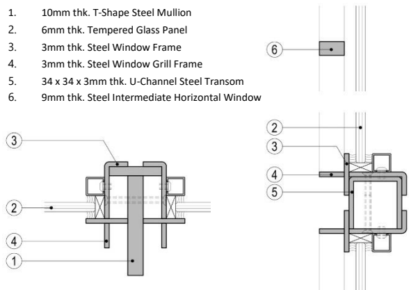
Figure 10: Reconstruction of featured steel window frame.
