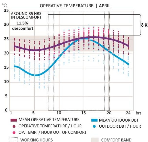
Figure 14. Monthly indoor operative temperature and outdoor DBT during 24-hour period for December (cooler month) and April (warmer month) and comfort hours with potential comfort band extension with adaptive opportunities.
