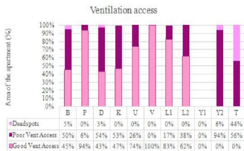
Figure 13: Ventilation Access –Removal of north wall – SW orientation
