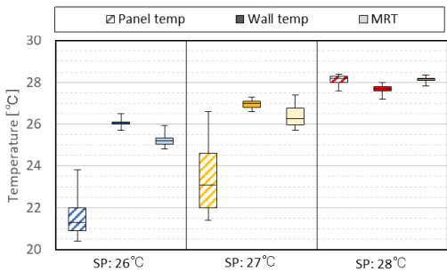
Figure 9: Surface temperature and MRT in the different set point temperature before occupied
