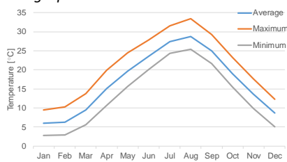
Figure 7: Monthly maximum, average, and minimum temperatures in Osaka 1) .
