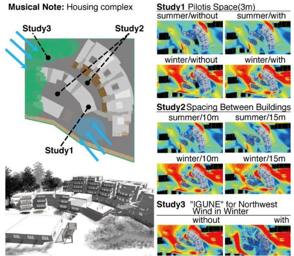
Figure 9a: Simulation of Wind Environment by Block Planning
