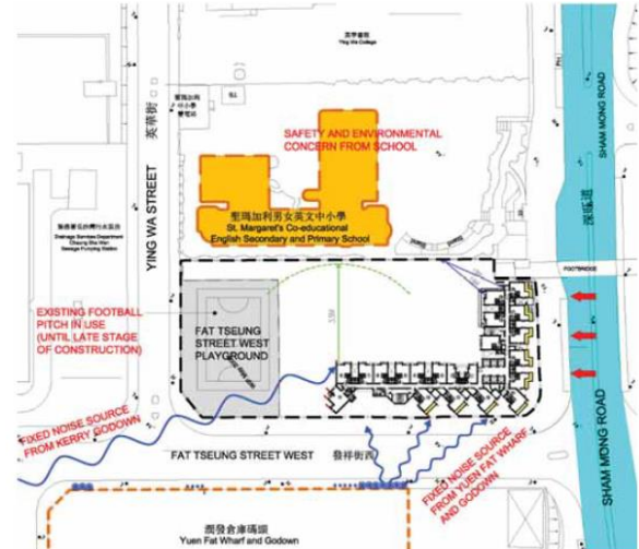
Figure 4: Site specific design of FTSW Development
