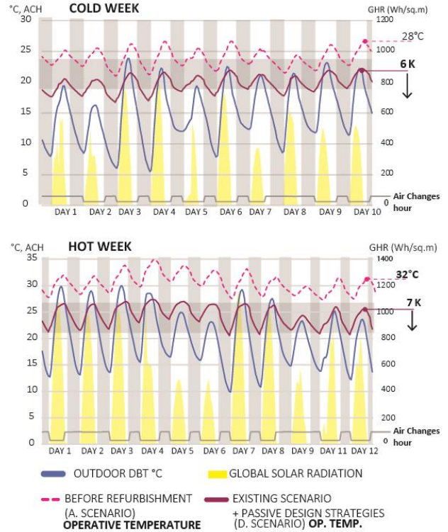
Figure 11. Comparison of thermal performance between scenario A (before the refurbishment) and D (after passive design strategies) under free running conditions for a typical hot and cold week. (After OpenStudio and Energy Plus)
