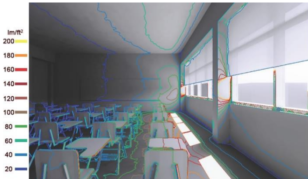
Figure 2: Illuminance levels shown as contour lines in perspective view of typical existing classroom on March 21st at 2pm, with shades lowered for sky brightness.
