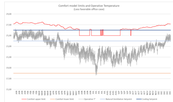
Figure 5: Graph of operating temperature and adaptive comfort limits in least favorable office (Source: Author)
