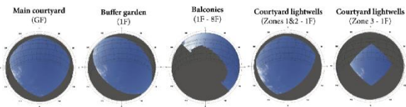
Figure 11: Shadow mask variation/sky framing for all proposed outdoor spaces (Source: Ladybug). [1]
