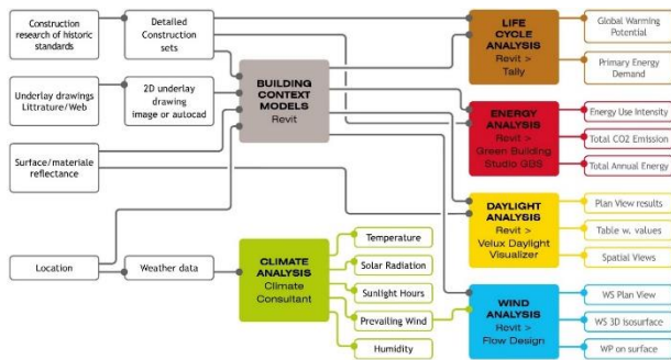
Figure 2: The workflow charts from construction research to building simulation (and related outputs)
