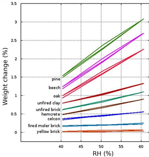
Figure 9: Humidity buffering for different materials [10]
