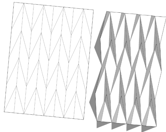
Figure 3: Diagram showing the folding pattern of the MIURA DDC geometry. The right side is a 3D illustration of its shape. This figure shows what this paper calls a vertical arrangement.
