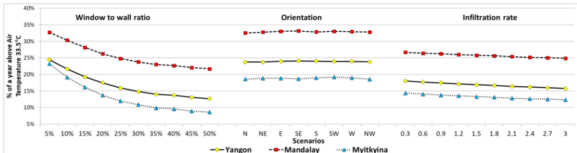
Figure 4: Comparison of overheating hours above 33.5°C for 5% to 50% WWR in the model (1), single-sided ventilated
