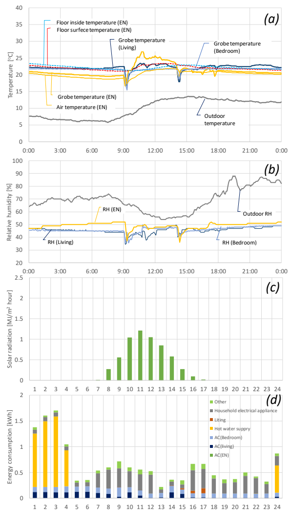
Figure 18: Results of environmental factors and electric consumption on 26 th November, a sunny day. (a) Globe, air and surface temperatures, (b) relative humidity, (c) solar radiation and (d) energy consumption.
