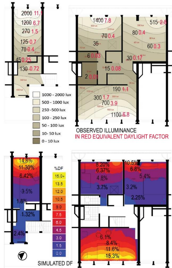
Figure 3: Robin Hood Gardens. Top: Indoor illuminance spot measurements taken on 16 th October 2010 at 12:00. Outdoor Illuminance: 18000Lux. Intermediate sky. Bottom: Daylight Factors from Radiance simulation (4)
