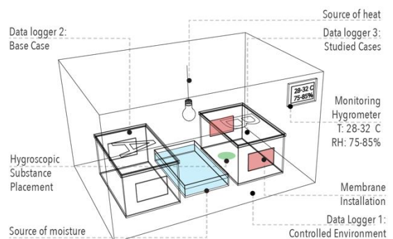
Figure 2: Experimentation set-up diagram [6]
