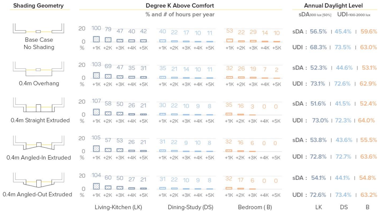
Figure 7: Comparing degree K above comfort and daylight level of the five shading geometries. Source [1]
