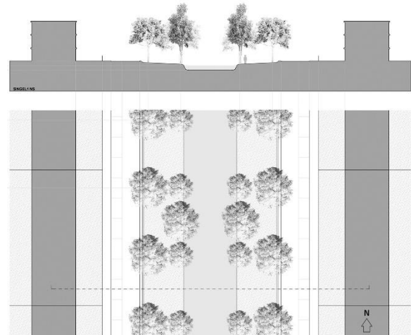
Figure 5: REALCOOL prototype WIDE CANAL1 NS.
