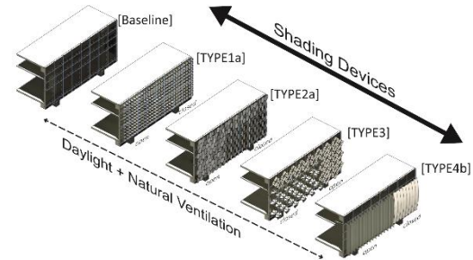
Figure 5: Four facade strategy types in pilot studies
