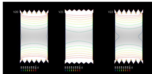
Figure 7: Showing the result of the fourth test V20 on the left, V21 in the middle and V22 on the right. At 750mm folding depth the V21 is not a shallow façade. This test also tested the fold from 300 mm onwards. The deeper façade folding, as much as 1500, creates less penetration of daylight.
