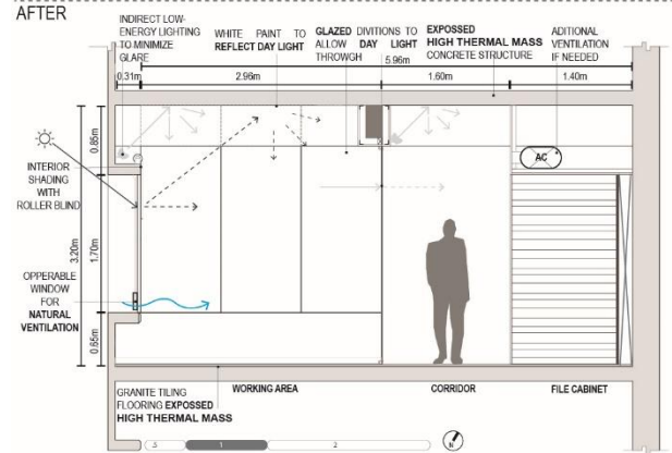
Figure 4: Typical section of studied floor - general construction details and passive strategies and design intentions after refurbishment (existing scenario). The section can be contrasted with the previous scenario show on figure 2.
