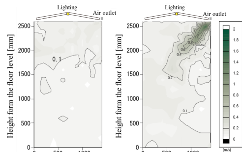
Figure 12: Sectional spatial distribution of air velocity in the interior space (Left: w/o airflow, Right: w/ airflow)
