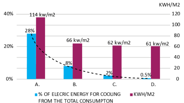
Figure 12. Annual electric energy consumption and cooling percentage for the various scenarios described above. The percentage of electric energy for cooling from the total consumption dropped up to 98% (scenario D.) - the total electric energy consumption was reduced up to 46% (Scenario D.). (After OpenStudio and Energy Plus)
