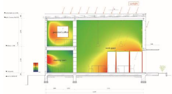
Figure 9: Section (light environment simulation).
