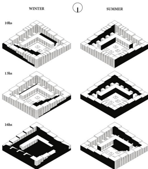
Figure 12: Sun access on façades (Source: Sketchup PRO) [1]
