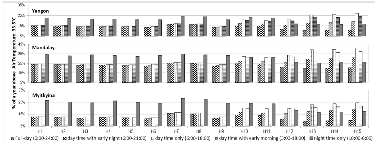
Figure 7: Comparison of overheating hours above 33.5°C for five window opening modes, Single-sided ventilation
