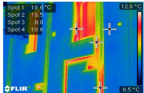
Figure 2: Thermographic images were used to highlight the gaps in external wall insulation due to poor detailing, leading to thermal bridges.
