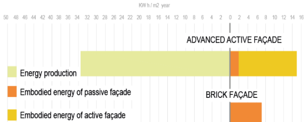
Figure 7: LCA results comparative. (Source : LAST).
