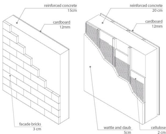
Figure 4: Left: Envelope for reference case ( U=2 ) / Right: improved case with cellulose insulation ( U=1.5 )
