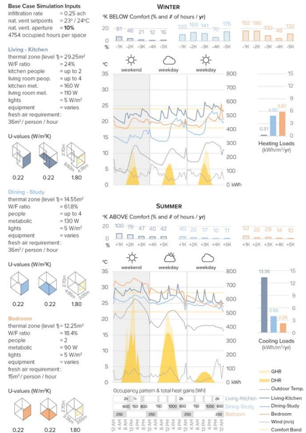
Figure 6: Base case thermal analysis results and energy loads from the infill prototype. Source [1].
