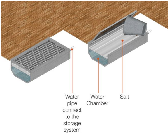
Figure 7: The Design of the Passive Salt Dehumidifier [6]
