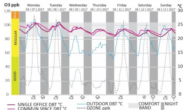
Figure 9: Air temperature data gathered at the 6th floor during one week (07/08/2017 to 13/08/2017), showing the interior DBT in relation to the outdoor DBT and the O3ppb levels. The chart also shows graphic representation of the relevant meteorological events.
