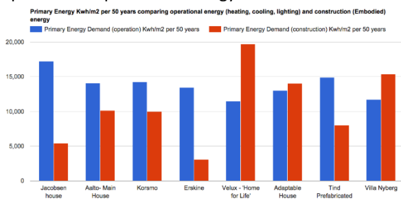
Figure 15: Used materials Primary Energy Demand (PED) in operation and for construction.
