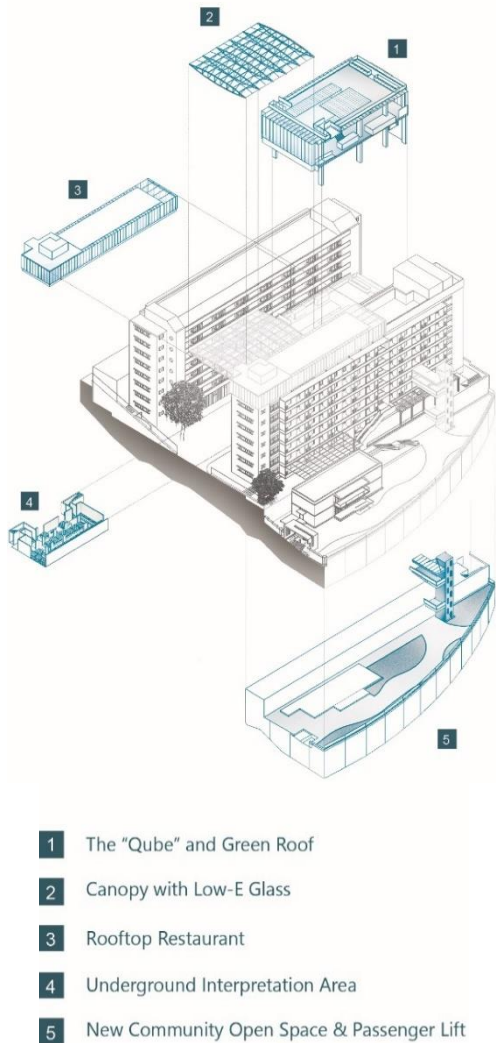
Figure 4: Isometric diagram showing the location of new elements in the site.
