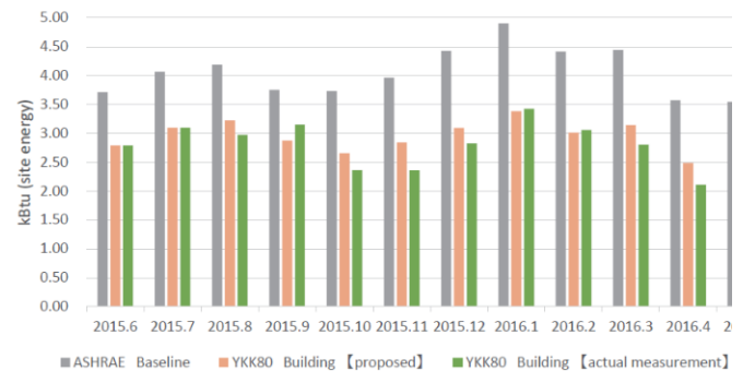
Figure 19: Monthly energy consumption for office space of baseline, proposed and actual measurement
