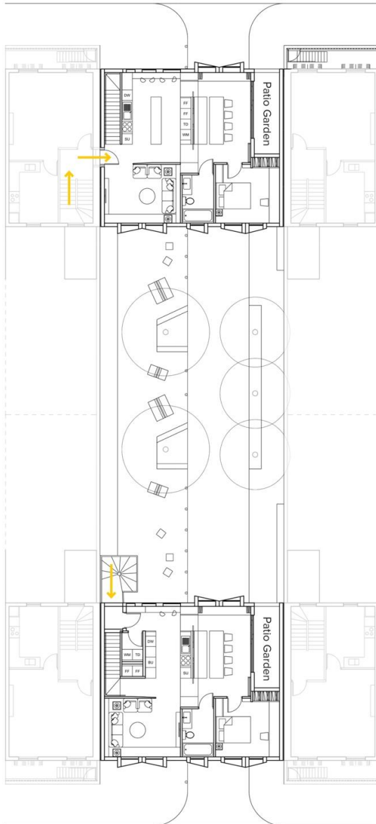
Figure 4: Spatial layout of two units (10.5m wide by 9.0m deep) with two options for accessing (illustrated with arrows) at the prototype site, with a pedestrianized connector road as community space. Source [1].
