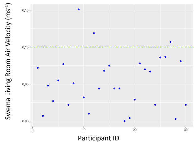
Figure 4: Air Velocity in each participating home ( N=30 ) measured using the industry standard Swema equipment and the value of 0.1\text{ms}^{-1} (blue dashed line) typically used as an assumed value in PMV-PPD calculations.
