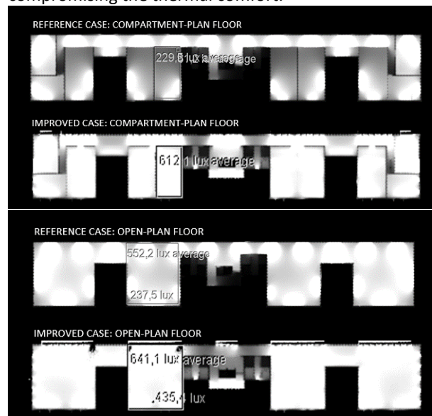
Figure 7: Illuminance Levels for improved and reference case (Source: Author)
