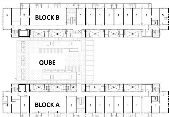
Figure 6: Plan showing the two Quarter Blocks and the QUBE bridging between them.
