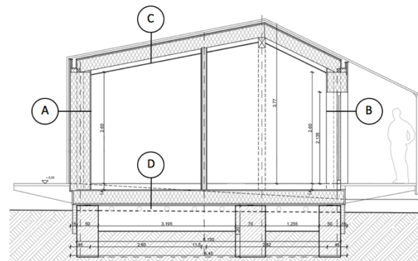
Figure 3: Building section of the Tennis club Lorentzweiler in Luxembourg
