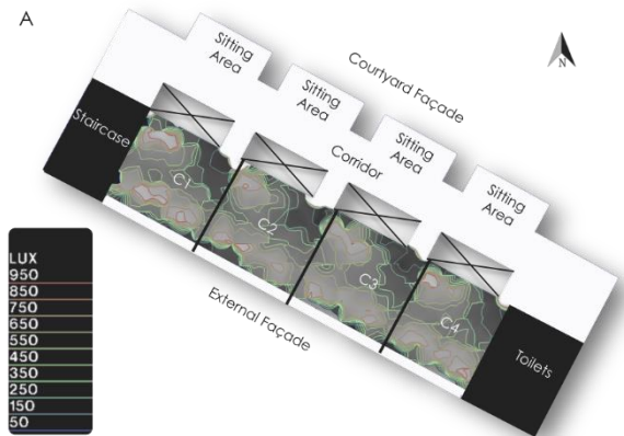
Figure 16: (A) Classroom Daylight Illuminance Performance Implementing 2mts Separation from the Corridor. Simulated the 21st of April at 3:pm, 1.2mts height.
