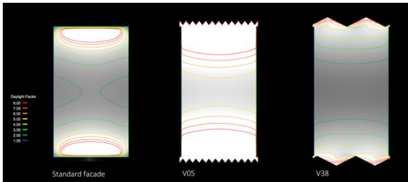
Figure 5: the result of the second test of Standard façade, V05 (passed the test) and V38 (failed the test).
