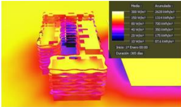
Figure 5: Solar Radiation at the Summer Solstice (source: Archiwizard Analysis)
