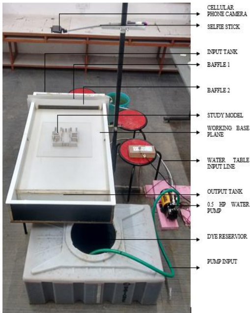
Figure 1: Water table apparatus experimental set-up at CEPT University (Royan & Vaidya, 2017)
