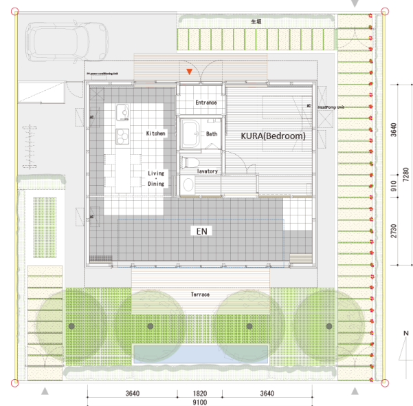
Figure 2: Plan of Kisekae House.
