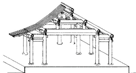
Figure 5: Typical Ancient Timber Architecture
