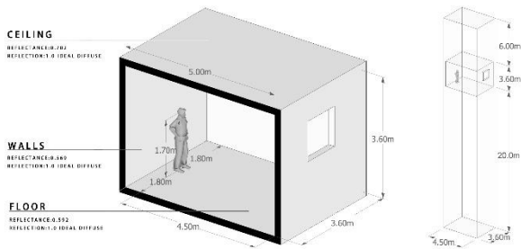
Figure 8: The model of test room
