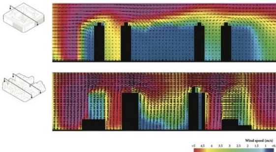
Figure 8: Air movement for the regulated and irregular blocks on a typical summer day (Source: ENVI-met 4.0) [1]
