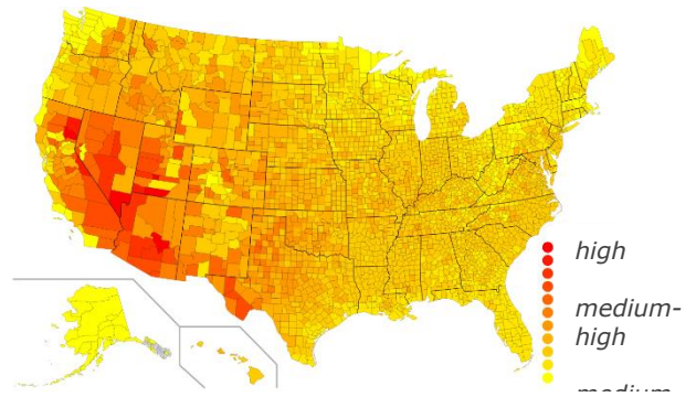
Figure 9: Passive evaporative cooling applicability (III). Determined from CH x [26°C-WBT].
