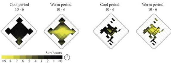
Figure 5: Solar access in regulated and irregular blocks (Source: Ladybug) [1]
