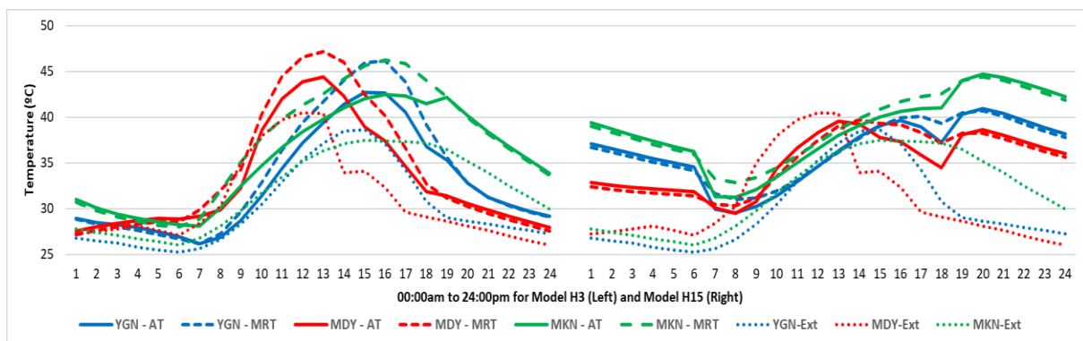
Figure 6: Comparison of AT and MRT in different cities for the hottest day, Single-sided ventilation
