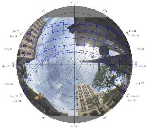
Figure 4: Solar access analysis by overlay of a fisheye image and a sun path diagram.
