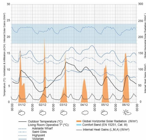
Figure 5: Thermal simulation results comparing living room operative temperatures under free-running conditions for four of the selected schemes over a typical winter week.
