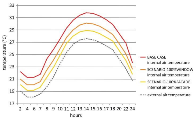
Figure 5: Air Temperature in a sunny summer day, comparing different scenarios: base case internal temperature; proposed scenario 01 (replacing window) internal temperature; scenario 02 (room with new facade) internal temperature; and external temperature.
