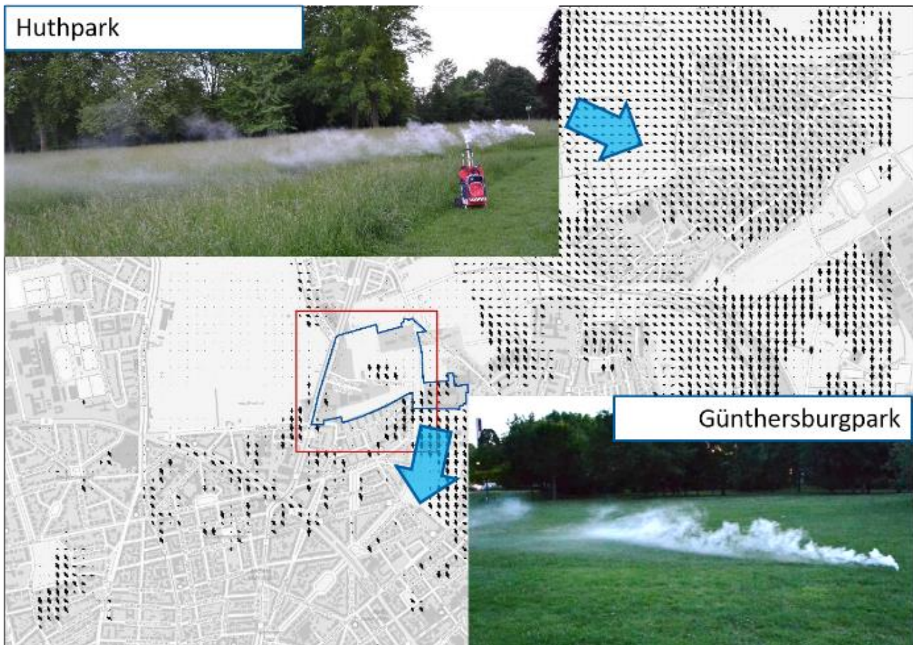
Figure 3: Cold air calculation, combined with near surface measurements and cold air evidence by smoke experiment.
