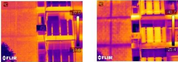
Figure 7: Thermal photo of the Sderot building at 13:00 on a winter day (right) and 19:00(left) before renovation (photo: Wolfgang Motzafi-Haller)
