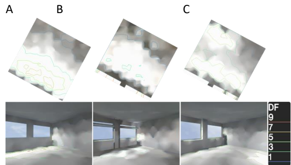
Figure 12: Classroom Daylight Factor Performance Plans and South Façade Perspectives of (A) Base Case (B) After the Implementation of Light Shelves (C) After the Addition of a Wall Zone. Simulated the 21st of April at 3:pm, 1.2mts height.
