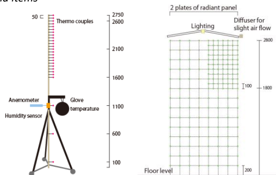
Figure 6: Methodology of manual measurements for spatial distribution in the office
