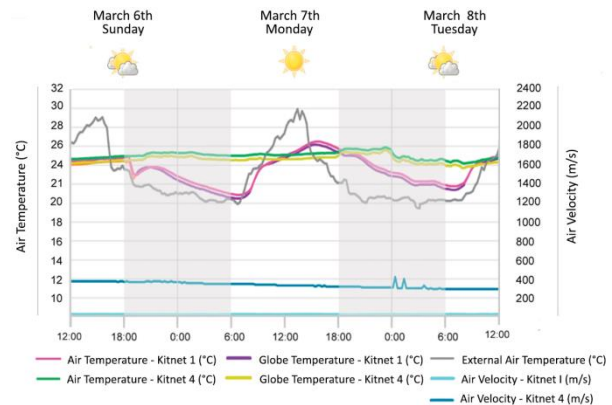
Figure 8: Measurements of dry bulb air temperature, globe temperature and air velocity in kitnets 1 and 4 during the warm period (March 2016).
