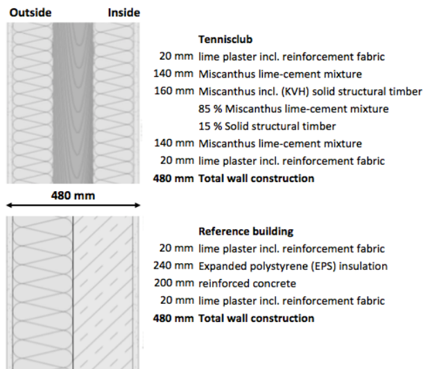
Figure 4: Wall construction of the Tennis Club and the reference building
