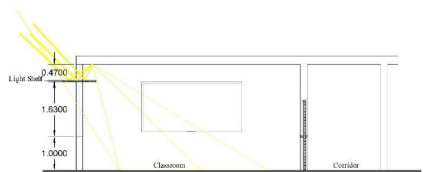
Figure 14: Schools Classroom Light Shelf Section Detail
