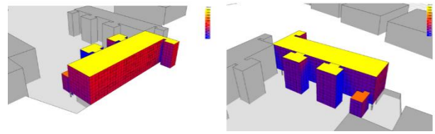
Figure 3: Solar radiation during a summer day on the north-east façade of the Sderot building (right) and on the south-west façade (left)
