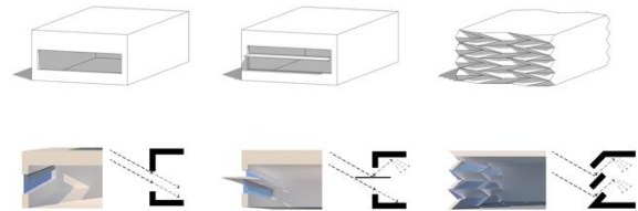
Figure 1: Diagram showing the three models that this paper tests. From left to right: Standard model, System with Reflection inspired by BARTENBACH, MIURA DDC. The paper develops variations of MIURA DDC geometry by changing dimensions and direction.
