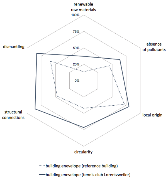
Figure 6: The “spider network diagram” compares the whole building envelope of the tennis club with the reference building envelope
