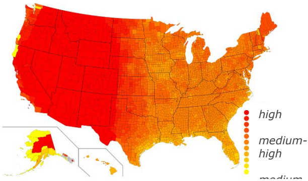
Figure 5: Passive evaporative cooling opportunity (II). Determined from DBT-WBT when DBT>26°C.
