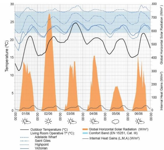
Figure 6: Thermal simulation results comparing living room operative temperatures under free-running conditions for four of the selected schemes over a typical summer week.
