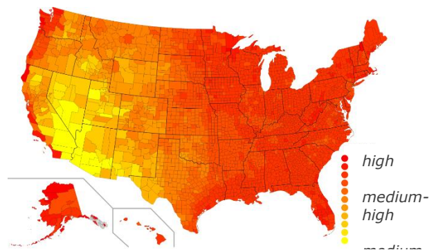
Figure 12: Active draught cooling opportunity (II). Determined from DBT-\text{WBT} .
