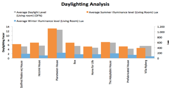
Figure 12: Simulated daylighting factors (above) and illuminance levels for living spaces at 12 o'clock the 21 of June and 21 of December and Lighting Loads.
