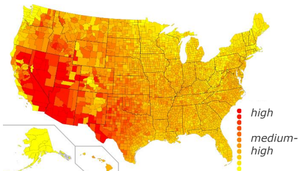
Figure 13: Active draught cooling applicability (I). Defined from CH \times [26^{\circ}\text{C}-\text{DPT}] .
