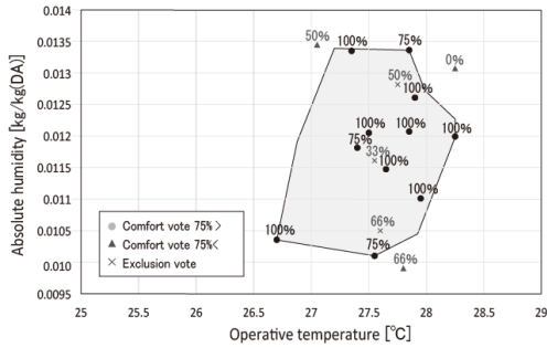
Figure 7: Expanded comfort areas based on 75% of the subjects
