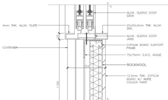
Figure 8: Sectional details of the thermal insulation of the building envelope.
