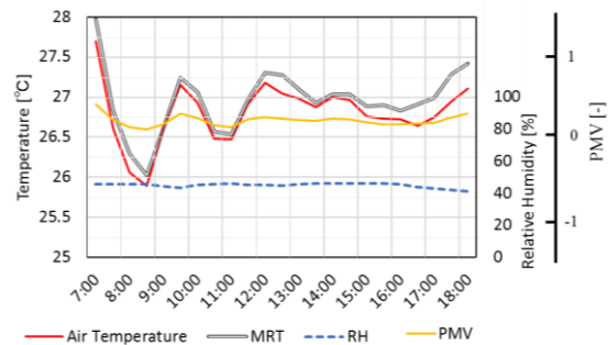
Figure 11: Fluctuation of the thermal environment in the interior space on a typical summer day ( Clo = 0.5 , Met = 1.1 )
