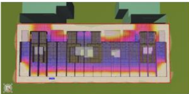
Figure 6: Natural lighting simulation: day.light factor (source: Archiwizard Analysis)
