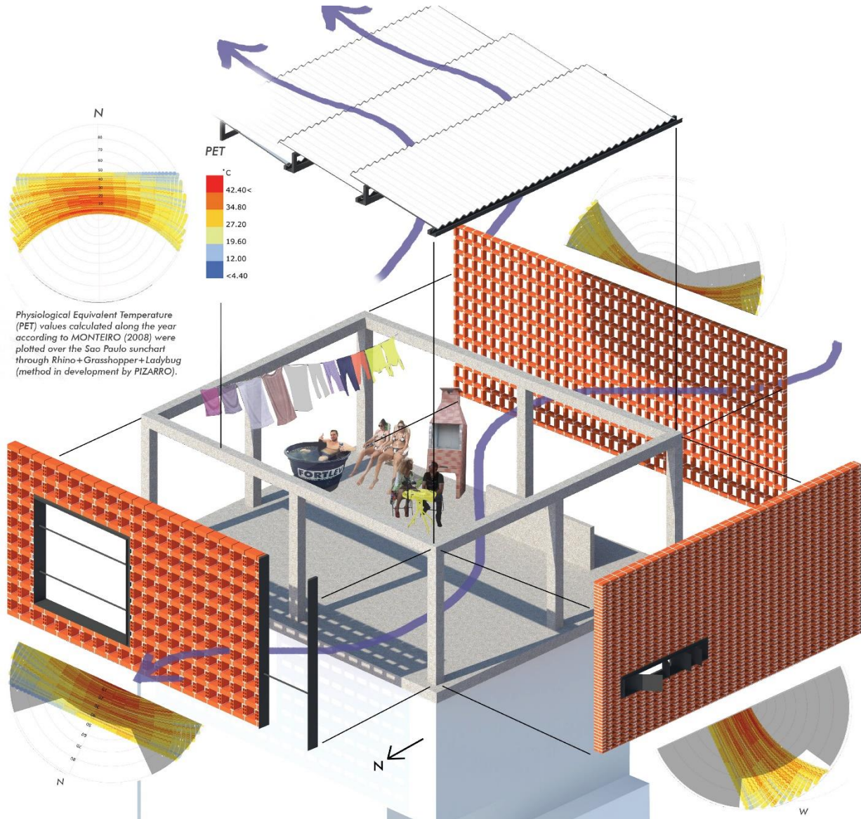
Figure 9: (Third outcome) Exploded Axonometric Perspective of the 1:1 Prototype, highlighting sun masks of different orientations.
