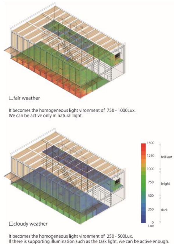
Figure 10: light environment simulation - illuminance distribution (June.21tt pm0:00) -
