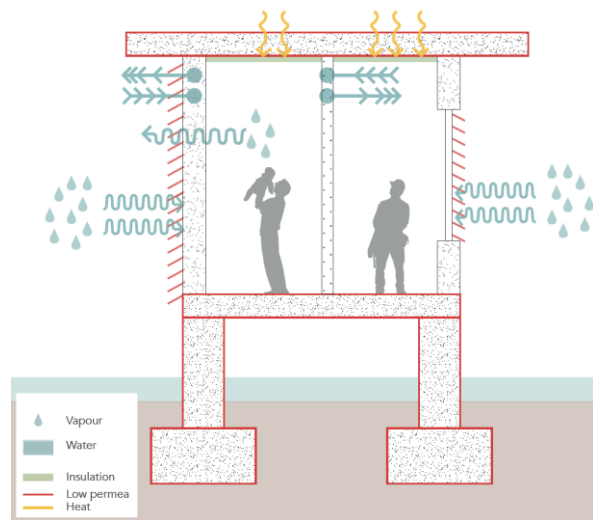
Figure 8: Breathable Material Diagram [6]
