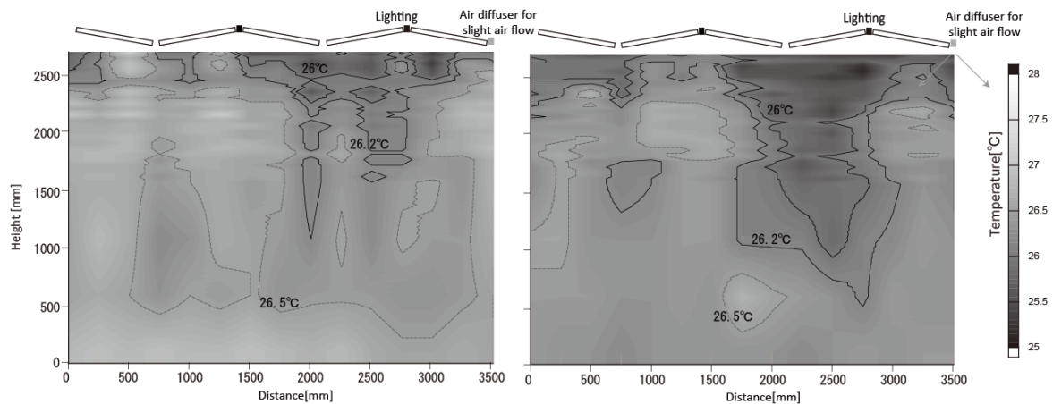
Figure 13: Sectional spatial distribution of air temperature in the interior space (Left: w/o airflow, Right: w/ airflow)
