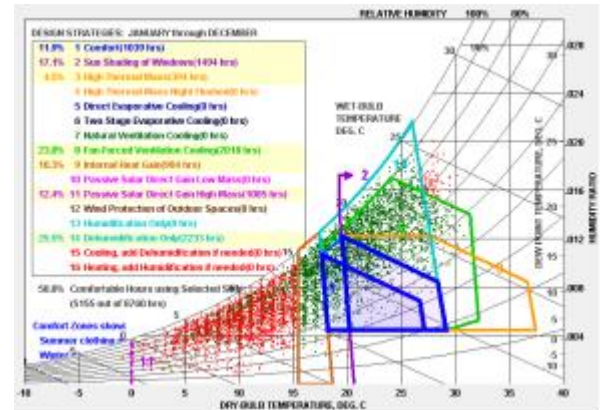
Figure 4: Psychometric chart analysis (Source: Climate Consultant, Meteonorm and Autodesk Weather Tool 2011 Analysis)
