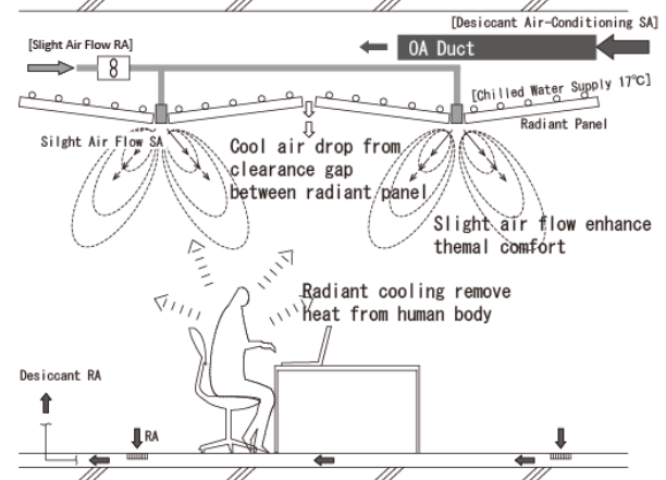
Figure 2: Diagram of slight airflow assisted radiant cooling
