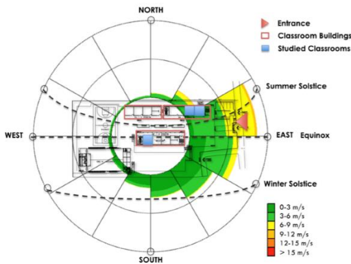
Figure 3: Context Analysis and Evaluated Classrooms in Constanza School. (Oceanic Climate Type (Cfb)). IESVE 2015.
