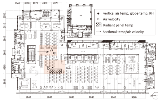
Figure 5: Plan for typical office floor with measurement points and items
