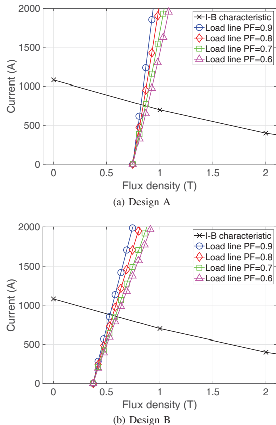
Fig. 3: Critical characteristic and load lines of the MgB_2 wire and determination of the critical currents.
