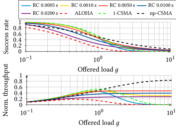
Fig. 21. Success rate (top) and normalized throughput (bottom) of nine nodes in a grid layout of 1\text{m} \times 1\text{m} for different RC values.
