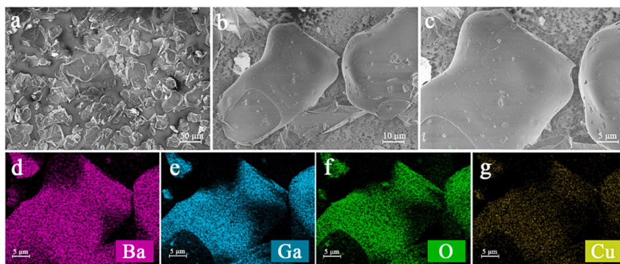
Fig. 2. (a - c) SEM morphologies of Ba_{0.95}Ga_2O_4:0.05Cu sample. The element mapping images of Ba (d), Ga (e), O (f) and Cu (g) in the sample.
