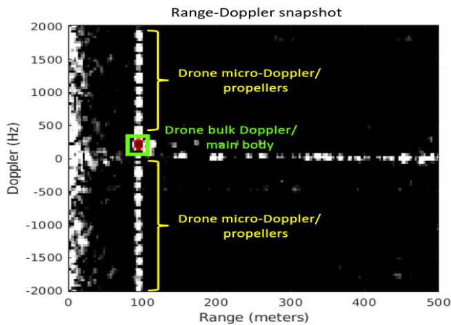
Fig. 2. Example of filtered range-Doppler containing a drone used as input for YOLO for detection and classification. The bulk Doppler and the micro-Doppler of the drone's propellers are both highlighted.
