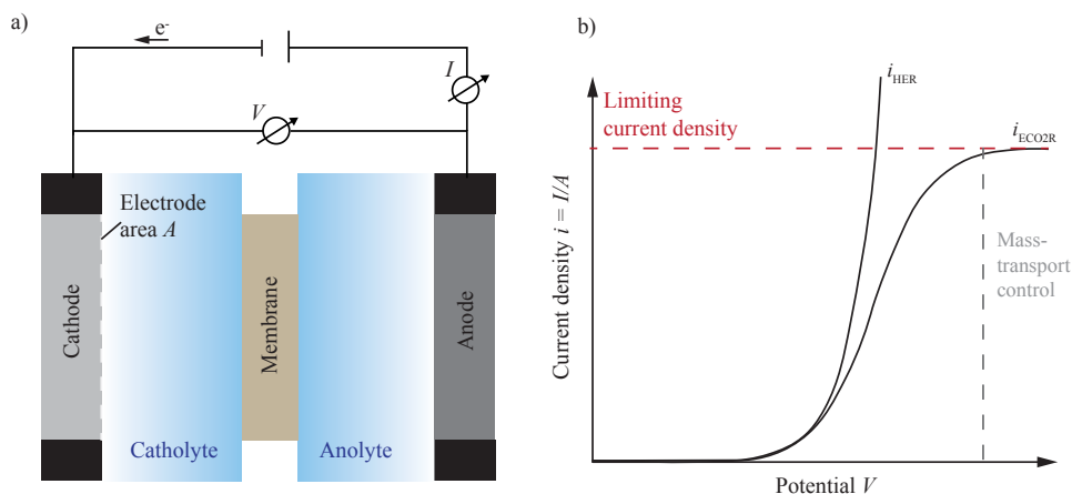
Figure 1.2: Schematic of a \text{CO}_2 electrolyser with planar electrodes shown in a). The relation between current density ( i = I/A ) and applied potential ( V ) is sketched in b), with the partial current density towards hydrogen ( i_{\text{HER}} ) and \text{CO}_2 reduction ( i_{\text{ECO2R}} ).
