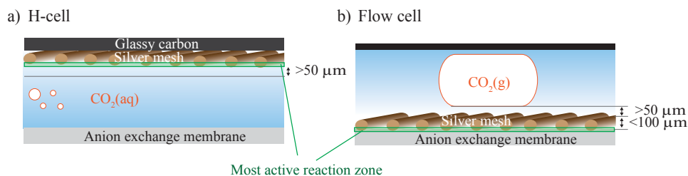
Figure 3.7: Representation of a) the cathode chamber in the H-cell configuration including the expected thickness of the diffusion layer close to the electrode and b) a unit cell with a gaseous \text{CO}_2 Taylor bubble flowing past the silver gauze with the expected liquid film and mesh thickness as the diffusion distance for the \text{CO}_2 to reach the most reactive zone in the electrolyser.
