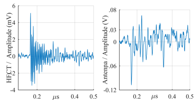
Fig. 15. Corona signal. Left: test cell HFCT; right: magnetic antenna.
