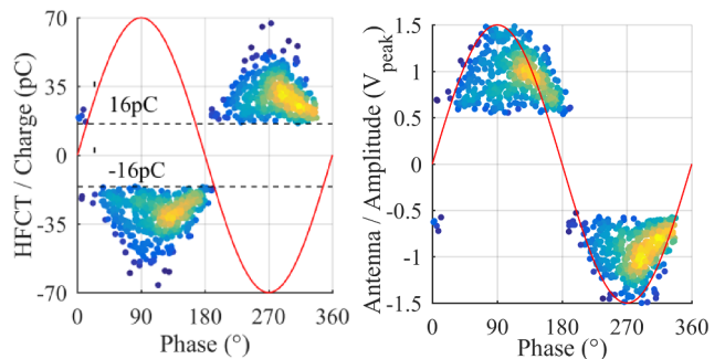
Fig. 11. PRPD pattern of free moving particle. Left: test cell HFCT; right: top loop.
