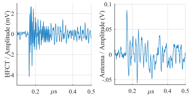
Fig. 16. Surface discharge signal. Left: test cell HFCT; right: magnetic antenna.
