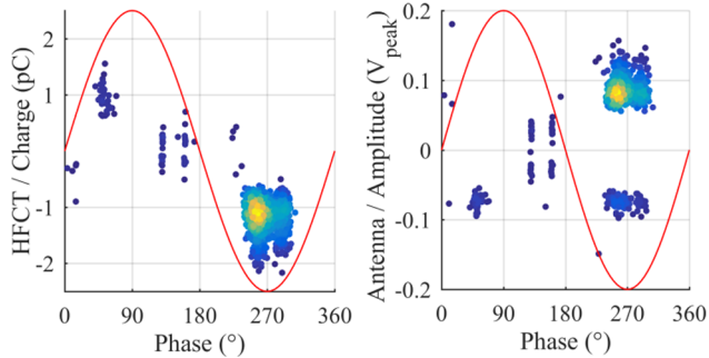
Fig. 13. PRPD pattern of surface discharges. Left: test cell HFCT; right: top loop.
