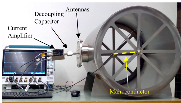
Fig. 5. Calibration rig workbench.
