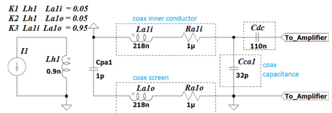
Fig. 3. Equivalent electric circuit of the magnetic antenna.
