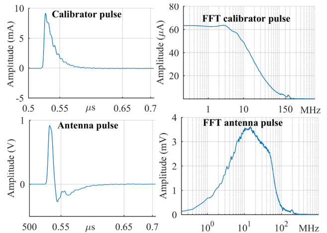
Fig. 6. Magnetic antenna response to a calibrator pulse.
