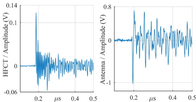
Fig. 14. Free moving particle signal. Left: test cell HFCT; right: magnetic antenna.
