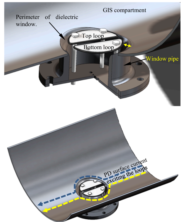
Fig. 2. Intersection of the GIS compartment and the dielectric pipe that results in a window in the GIS compartment. (a) Cutaway view of the position of the magnetic antenna relative to the compartment window; (b) perspective view of the PD current around the magnetic antenna.
