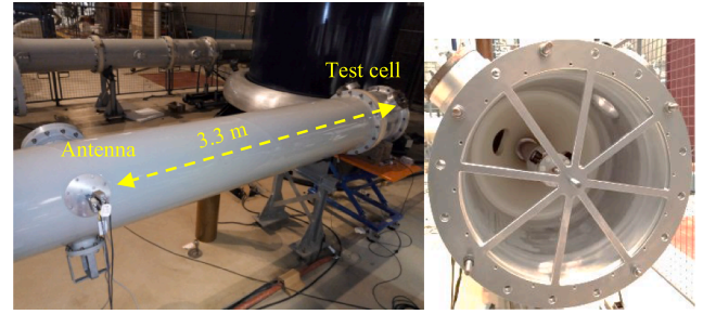
Fig. 10. Localization of the magnetic antenna and test cell in the GIS.
