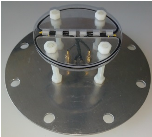
Fig. 1. Construction of the magnetic antenna showing both 1-turn loops assembled on the mounting plate.
