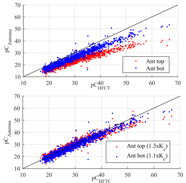
Fig. 18. Top: correlation between the charge values from the test cell HFCT and the antennas; bottom: compensation of the calibration factor.
