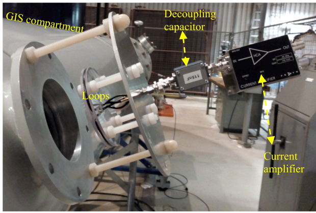
Fig. 4. Connection arrangement of the magnetic antenna, decoupling capacitor and transimpedance amplifier.
