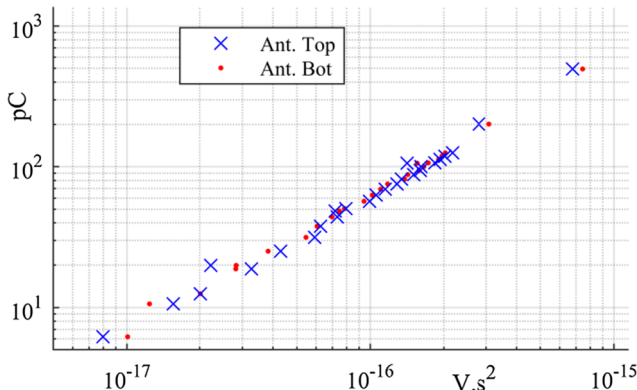
Fig. 9. Relation between the injected charge and the integral response from the antennas tested in the test bench.
