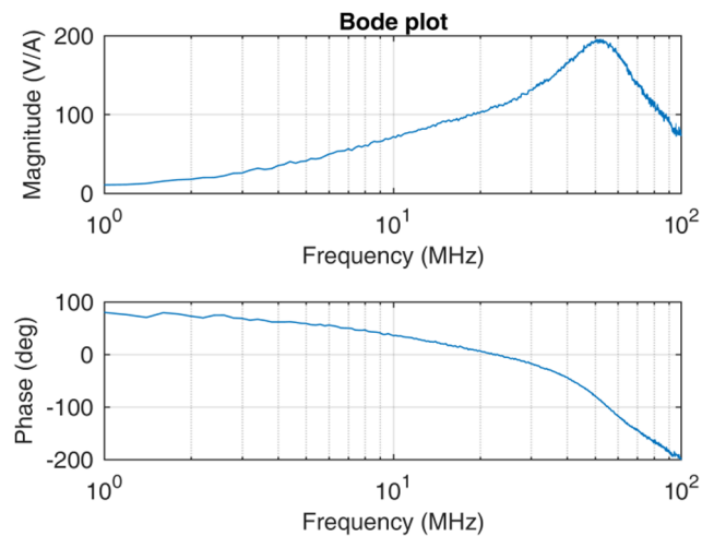
Fig. 7. Bode diagram of the magnetic loop antenna.
