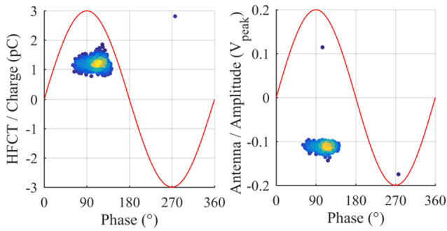
Fig. 12. PRPD pattern of corona. Left: test cell HFCT; right: top loop.
