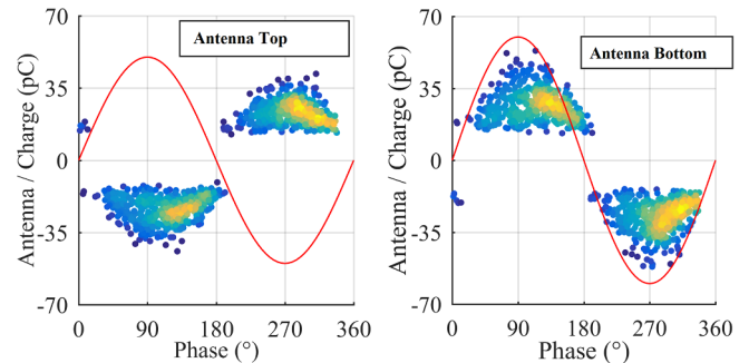
Fig. 17. PRPD of free moving particle test measured by left: top antenna, right: bottom antenna.
