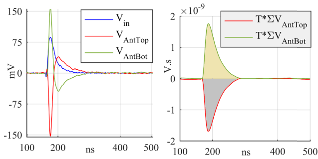
Fig. 8. Left: example of injection of a 50 pC pulse and response from the antennas; right: integration of the antenna’s output.
