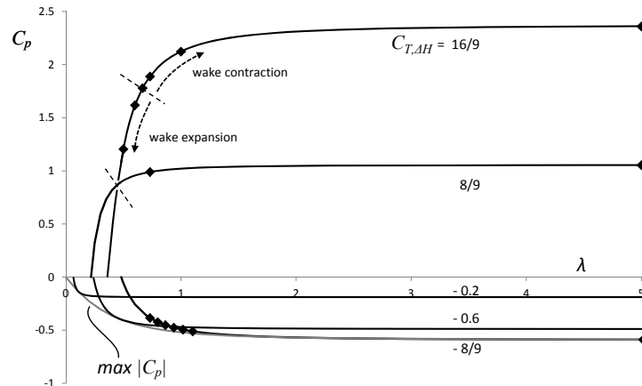
Figure 3. The Joukowsky momentum theory results (black lines), the maximum wind turbine |C_p| (grey line) and the potential flow calculated results ( \blacklozenge )
