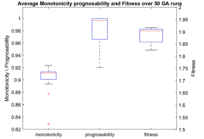
Fig. 7. Average monotonicity, prognosability and fitness with variance over 50 Genetic algorithm runs.
