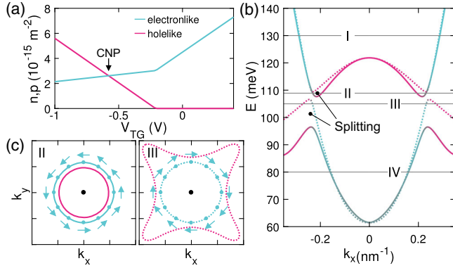
FIG. 1. (a) Expected electron and hole densities dependence on V_{TG} . (b) Numerical band structure calculation for V_{TG} = -0.4 V. The color indicates the wave function main character, solid and dotted lines distinguish two spin-orbit split subbands. (c) Fermi contours and spin texture of electronlike states for the Fermi energies II and III indicated in (b). The axis divisions are 0.2 \text{ nm}^{-1} , with the black dot indicating the origin. Fermi pockets at large k vector are ignored, but discussed further in the Supplemental Material [23].
