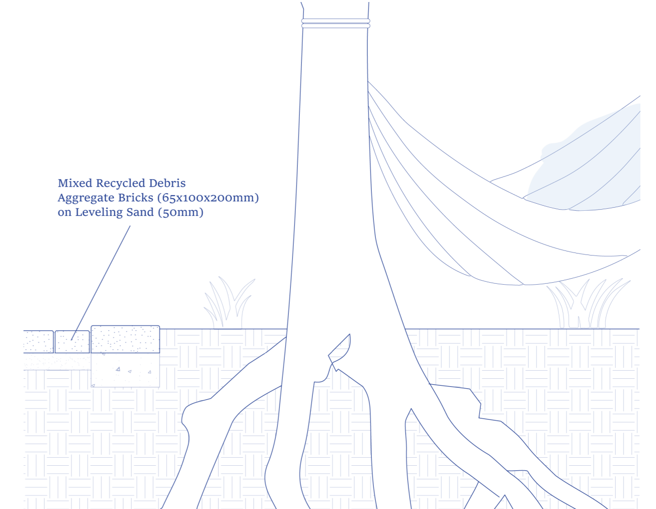
Relaxation Area - Hammock and Tree Detail - Vertical 1:10
