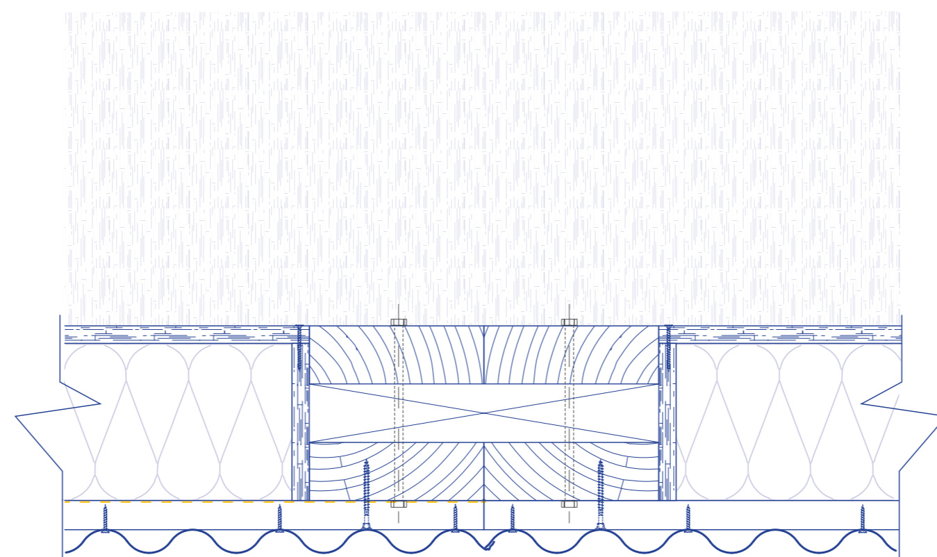
Module to Module Connection Detail - Horizontal 1:5
