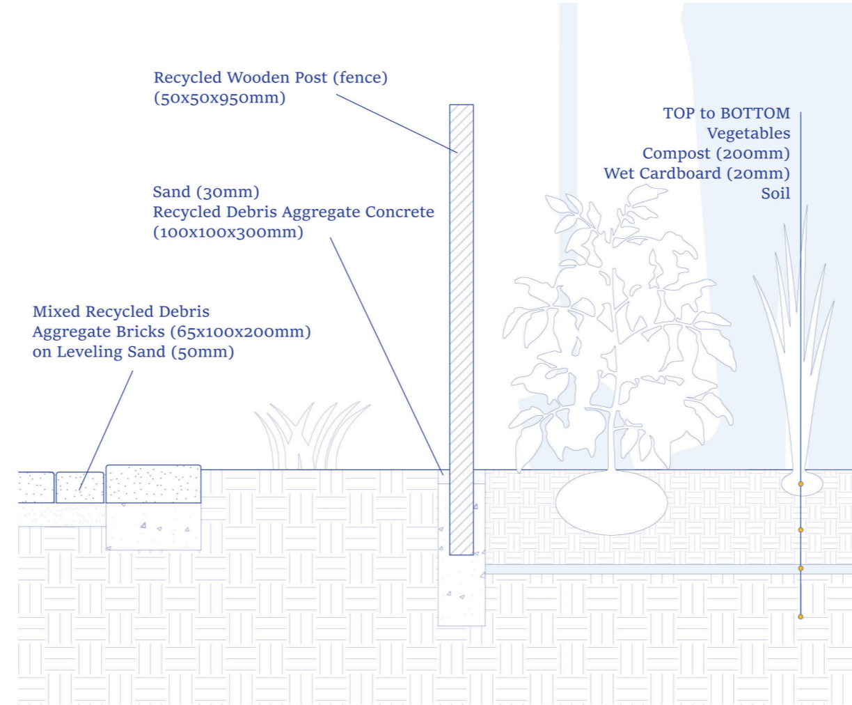
Vegetable Garden Detail - Vertical 1:10
