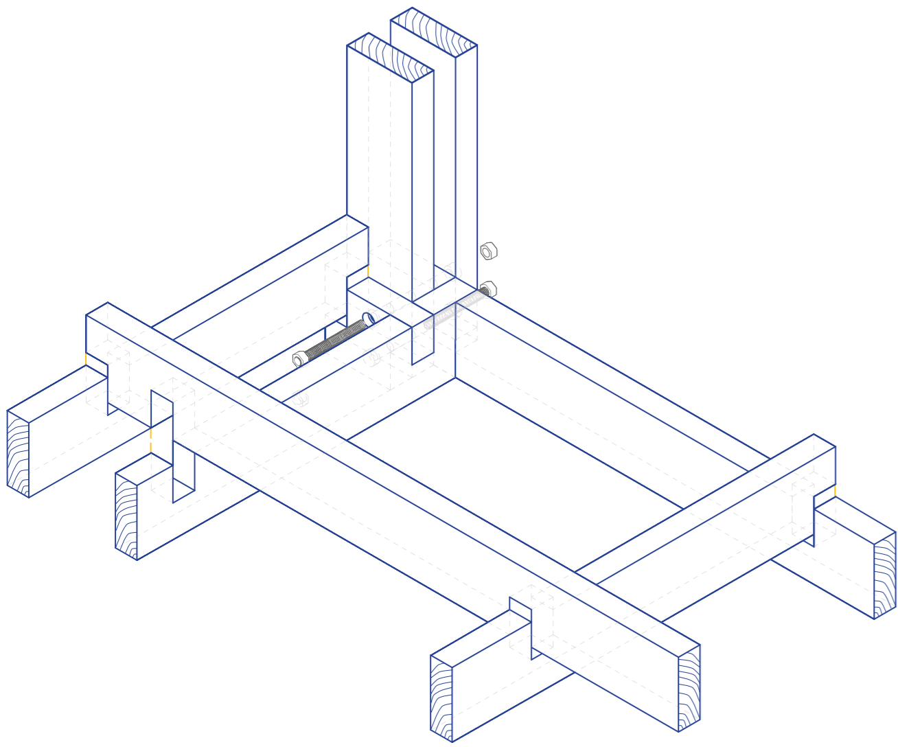
Bottom Corner Structure Detail 1:10
