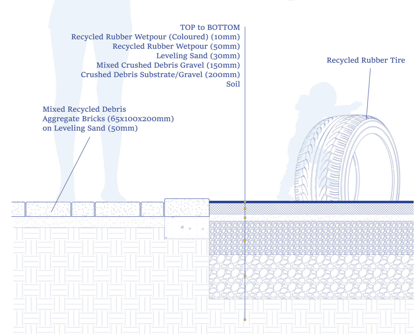
Children (After-)School Area - Playground Detail - Vertical 1:10
