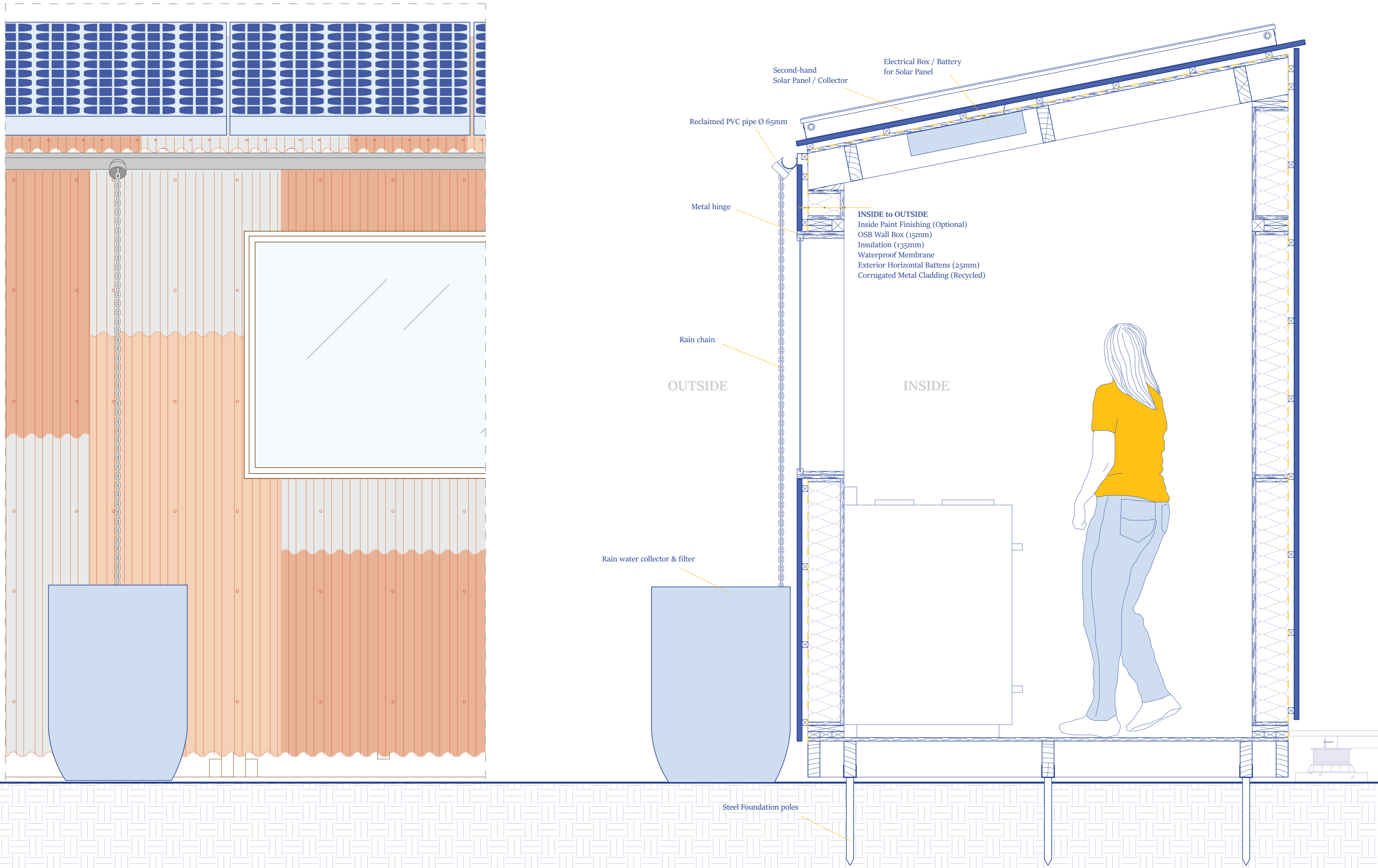
Combination Drawing Detail - Elevation - Section - Floorplan - Small Module - Shared Kitchen 1:10
