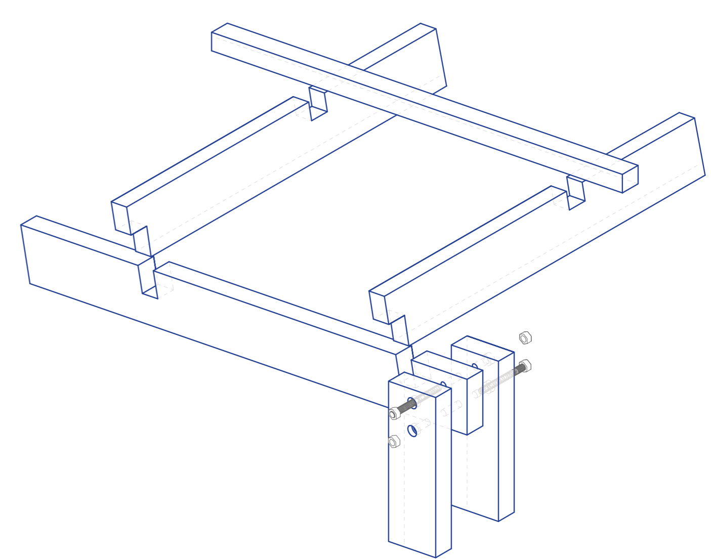
Top Corner Structure Detail 1:10
