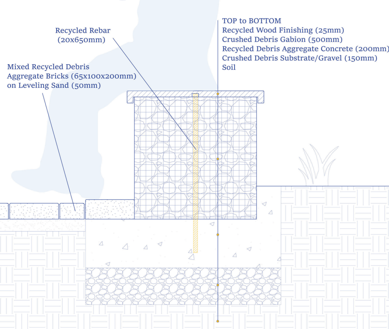
Gabion Bench - Walking Path Detail - Vertical 1:10
