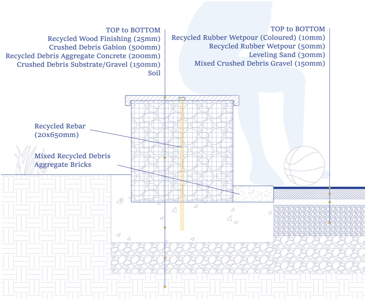
Gabion Bench - Basketball Court Detail - Vertical 1:10
