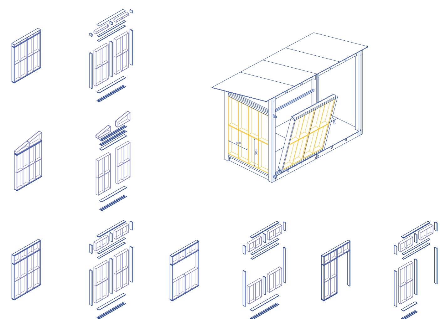
Wall Composition and Structural Breakdown
