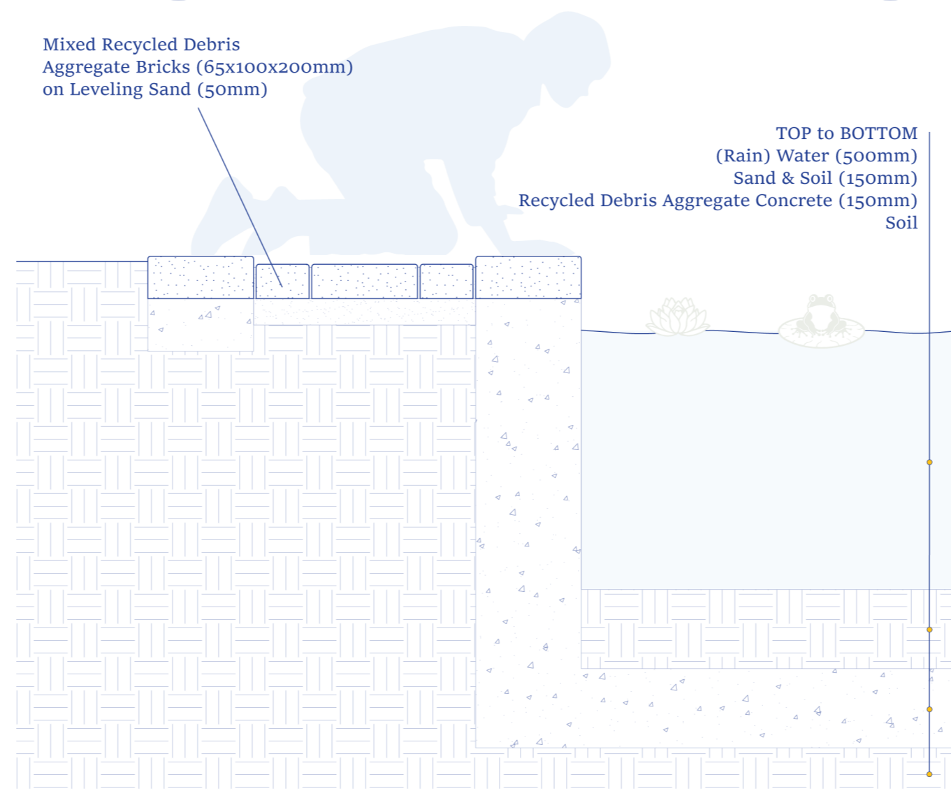
(Rain Water) Pond Detail - Vertical 1:10
