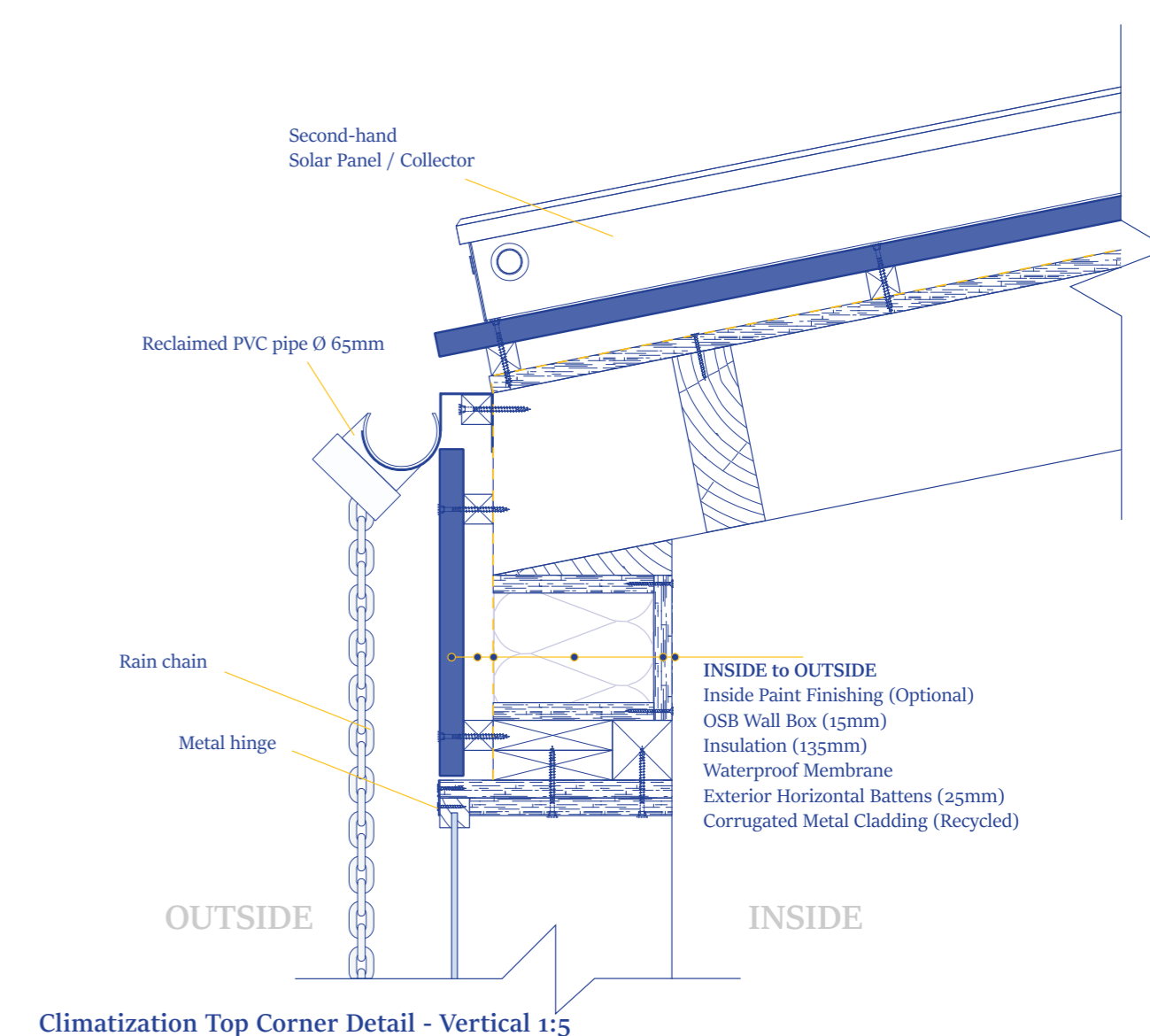
Climatization Top Corner Detail - Vertical 1:5
