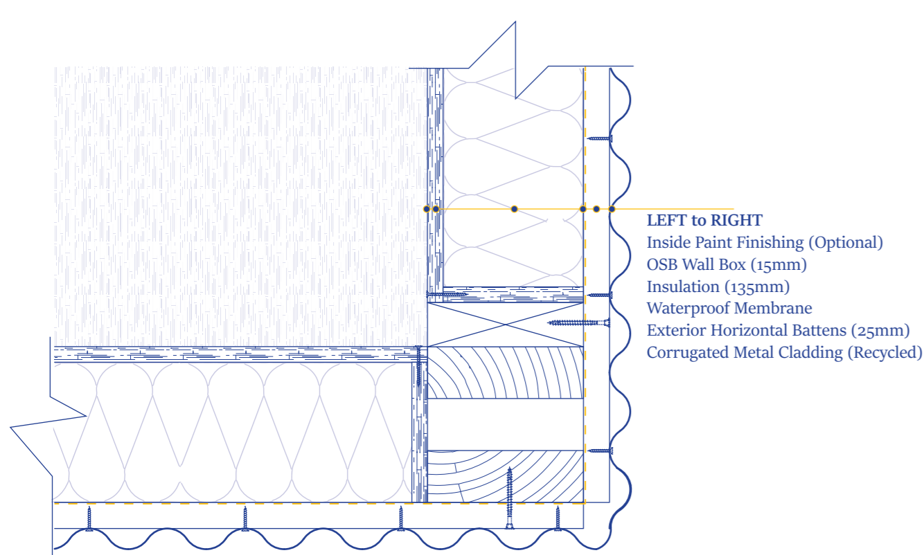
Corner Detail - Horizontal 1:5
