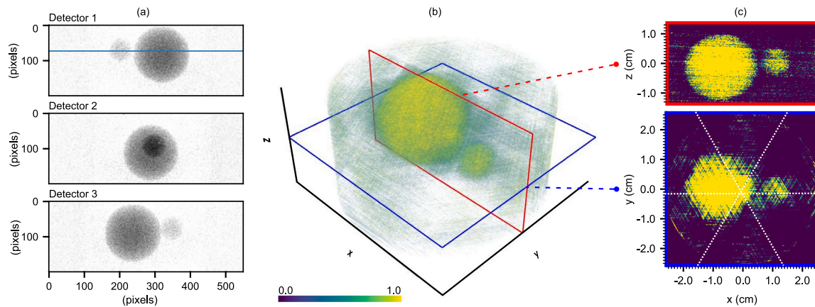
Fig. 9. Reconstruction of two polystyrene phantoms, with diameters D_1 = 23 mm and D_2 = 10 mm, that overlap on the second detector. The reconstruction, panel (b), has been rotated to match Fig. 7. The detector row marked in blue is used to compute noise statistics in Fig. 11. The visualization format is explained in Section 4.3.
