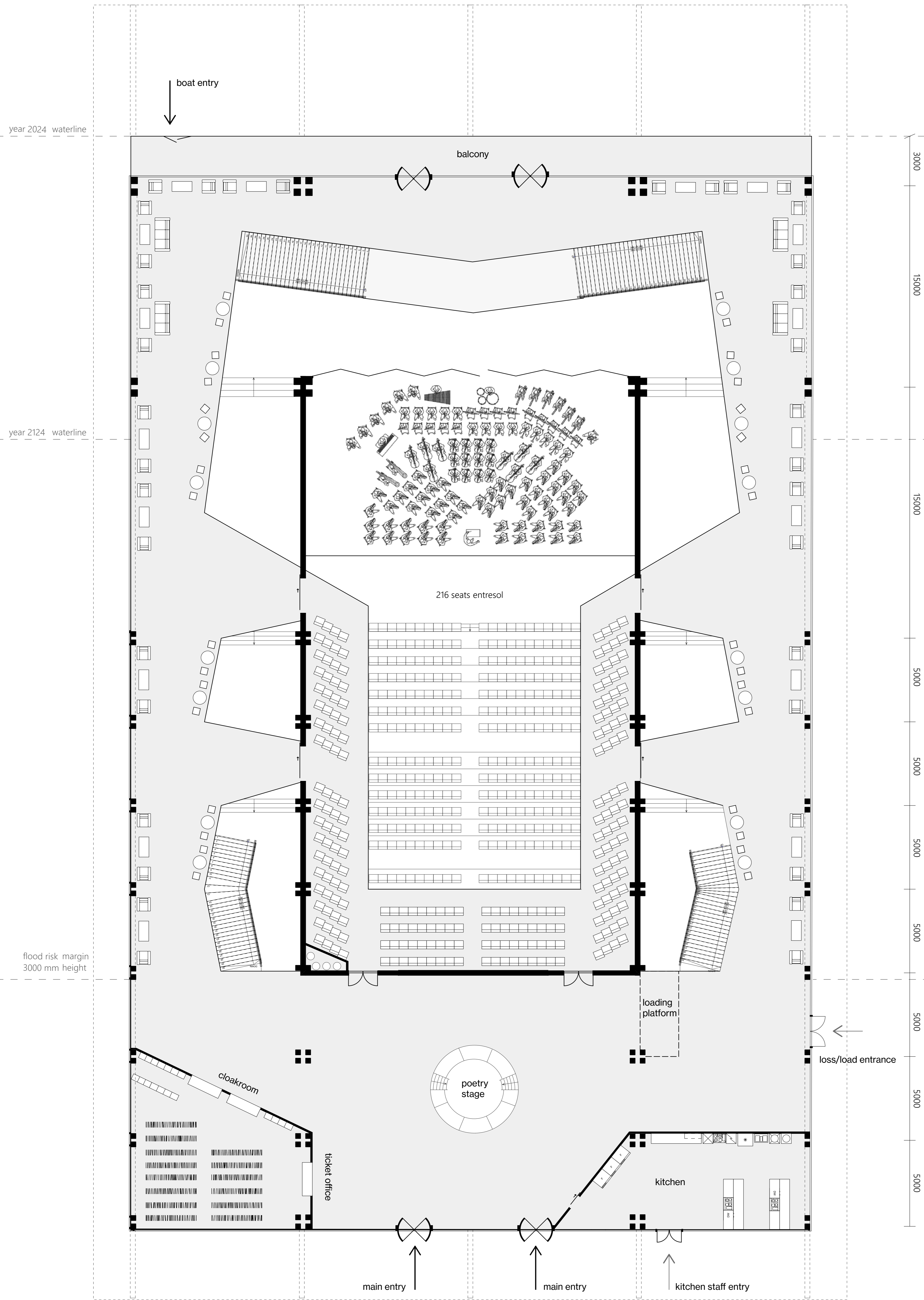
FLOOR PLAN GROUND LEVEL 1 : 100
