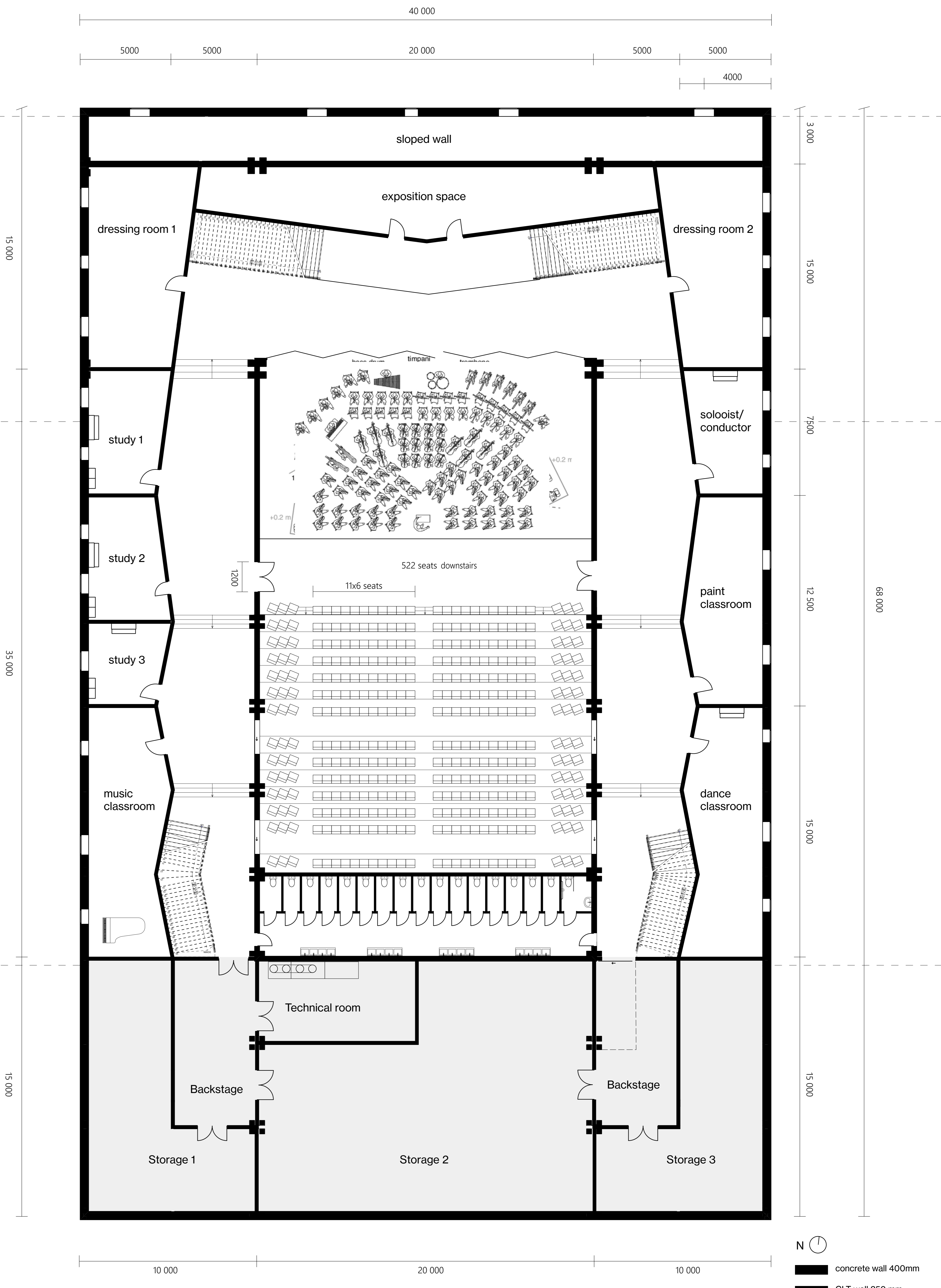
FLOOR PLAN UNDERGROUND LEVEL 1 : 100
