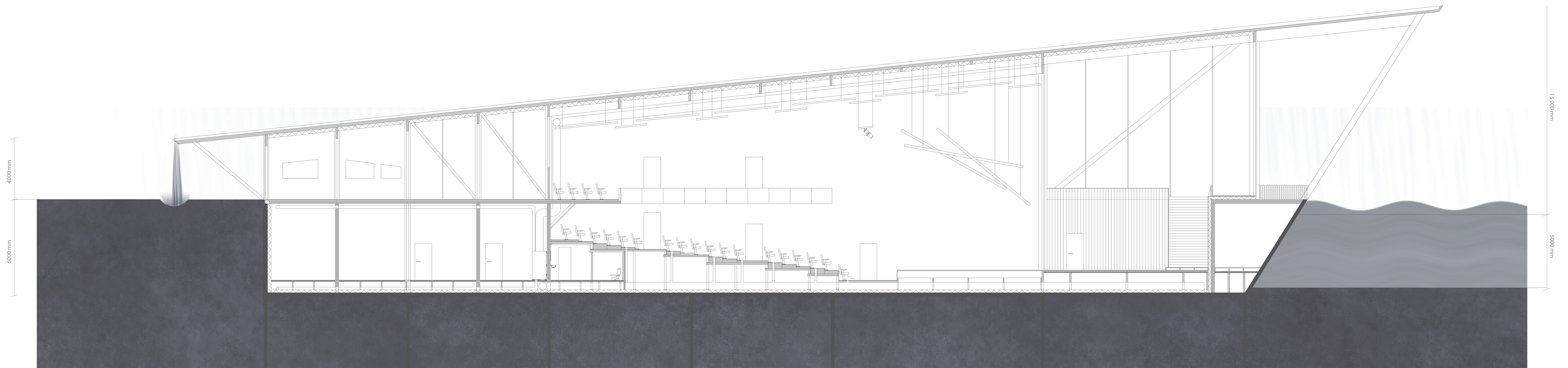
SECTION VIEW LENGTH 1 : 100
