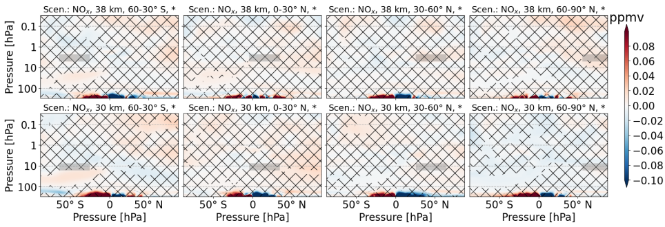
Figure A.25: Zonal mean of H_2O perturbation (volume mixing ratio, ppmv) for scenarios where NO_x is emitted. The first and second row refer to 38 km and 30 km altitudes of emission, respectively. Columns represent the latitude region of emission. The emission regions are shaded in gray. Lines indicate statistically insignificant results and the probability level is written in the title of each subplot.
