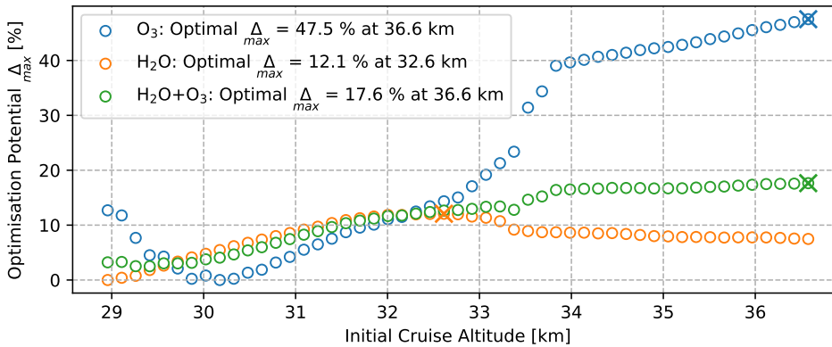
Figure 8.6: Relative optimisation potential \Delta_{max} based on ozone and water vapor net radiative forcing calculations for the individual net radiative forcings and the total net radiative forcing.
