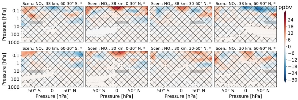
Figure A.26: Zonal mean of H_2 perturbation (volume mixing ratio, ppbv) for scenarios where NO_x is emitted. The first and second row refer to 38 km and 30 km altitudes of emission, respectively. Columns represent the latitude region of emission. The emission regions are shaded in gray. Lines indicate statistically insignificant results and the probability level is written in the title of each subplot.
