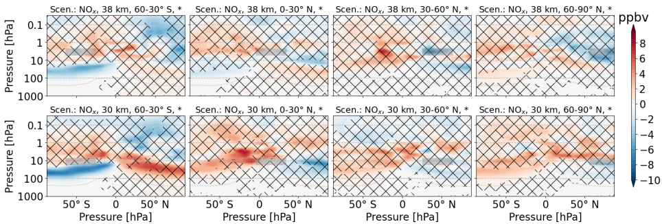
Figure A.27: Zonal mean of CH_4 perturbation (volume mixing ratio, ppbv) for scenarios where NO_x is emitted. The first and second row refer to 38 km and 30 km altitudes of emission, respectively. Columns represent the latitude region of emission. The emission regions are shaded in gray. Lines indicate statistically insignificant results and the probability level is written in the title of each subplot.
