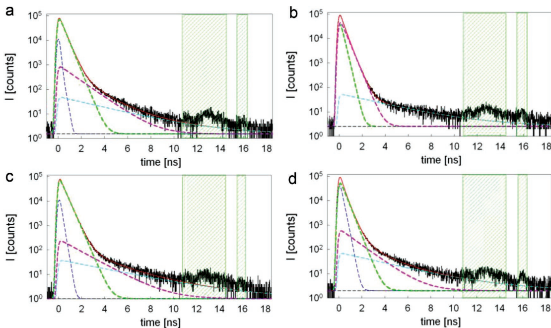
Figure 8. PALS spectra at 1 keV and fits obtained using POSWIN of a) papain/titania nonlayer, b) annealed (450 °C, 4 h) papain/titania nonlayer, c) TiO 2 reference sample fabricated using EBPVD, and d) ITO layer on glass substrate. The regions between 10.8 and 14.5 ns as well as 15.6–16.2 ns have been excluded from fitting, due to the presence of spurious peaks of annihilation by backscattered positrons.
