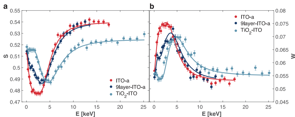
Figure 6. Comparison of DB-PAS depth profiles of papain/titania nonalayer on ITO-coated glass and the EBPVD-TiO 2 and annealed ITO reference samples. Dashed lines are best-fits from VEPFIT analysis (see Table 2). The reference sample is made with electron-beam physical vapor deposition and has a thicker ITO coating of \approx 100 nm, and a different type of glass substrate. Annealing of the nonalayer and of the ITO reference sample is done at 400 °C for 4 h.
