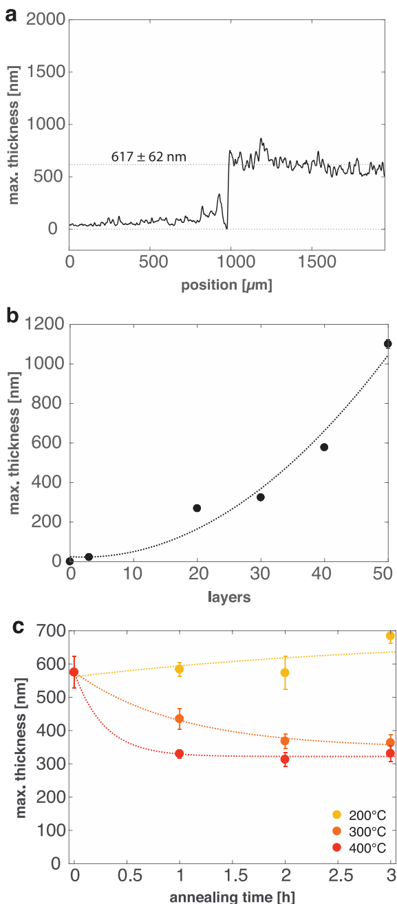
Figure 2. a) Profilmetry thickness measurement of as-deposited papain/titania nonalayer. b) Thickness of papain/titania layers as a function of number of deposited layers using 10 \times 10^{-6} M papain in 20 \times 10^{-3} M MOPS pH 7.0, determined from profilmetry. c) Thickness of papain/titania nonalayers deduced from profilmetry as a function of annealing time for three different annealing temperatures, 200, 300, and 400 °C.
