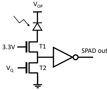
Figure 5.1. nanoSPAD pixel schematic with cascode transistors to allow for high VOP.
