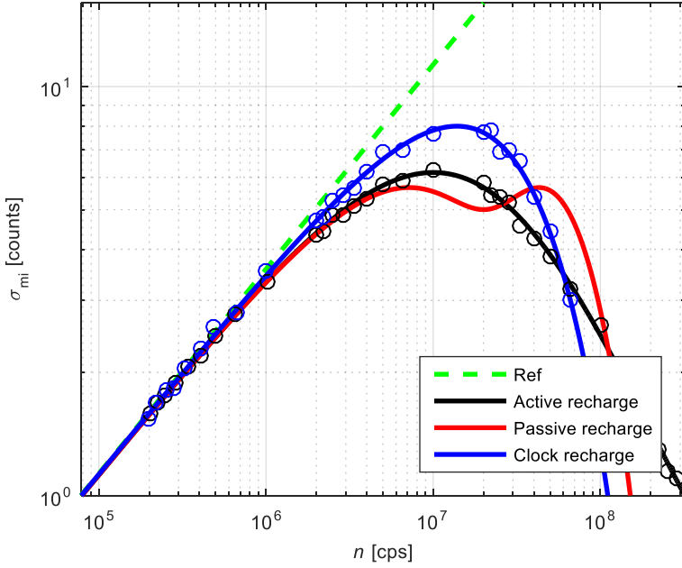
Figure 2.5. Modeled standard deviation of the measured count number \sigma_{mi} due to shot noise and count suppression, T_{dead}=50 ns and t=12.8 \mu s. Green shows the reference, i.e. standard deviation due to shot noise. Circles indicate simulated data.
