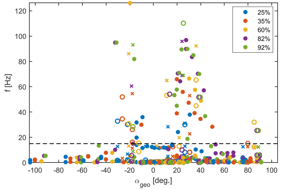
FIGURE 11 Scatter plot showing dominant frequencies observed in all standstill cases versus the corresponding geometric angle of attack (AoA) ( \alpha_{geo} ) at a particular test condition and spanwise location. The cross markers (x) denote presence of spanwise flow from tip to root, hollow circle markers (o) denotes presence of spanwise flow from root to tip, and filled circle markers (•) represent no spanwise flow. The dashed black line denotes the 15-Hz frequency level [Colour figure can be viewed at wileyonlinelibrary.com]
