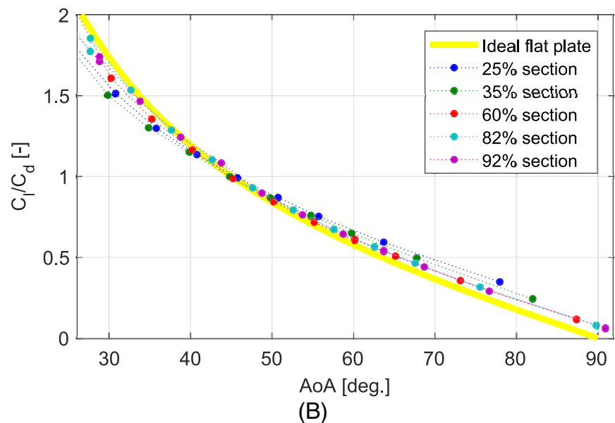
FIGURE 8 Lift to drag ratio versus angle of attack (AoA) for the new model rotor experiments under controlled conditions (New MEXICO) blade sections. A, A comparison of lift to drag ratio of 3D polars from five different sections of New MEXICO blade with the ideal flat plate theory and 2D airfoil polars. B, A close-up of Figure 8A in the deep stall regime [Colour figure can be viewed at wileyonlinelibrary.com ]
