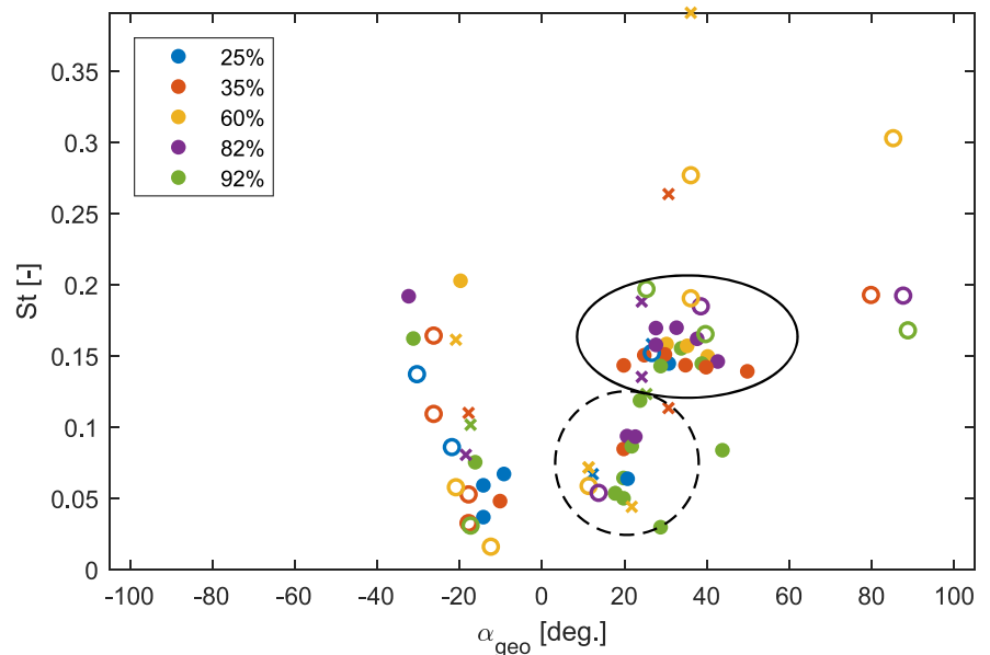
FIGURE 12 Scatter plot showing Strouhal numbers observed in all standstill cases versus the corresponding geometric angle of attack (AoA) ( \alpha_{geo} ) at a particular test condition and spanwise location. The cross markers (x) denote presence of spanwise flow from tip to root, hollow circle markers (o) denotes presence of spanwise flow from root to tip, and filled circle markers (•) represent no spanwise flow [Colour figure can be viewed at wileyonlinelibrary.com]
