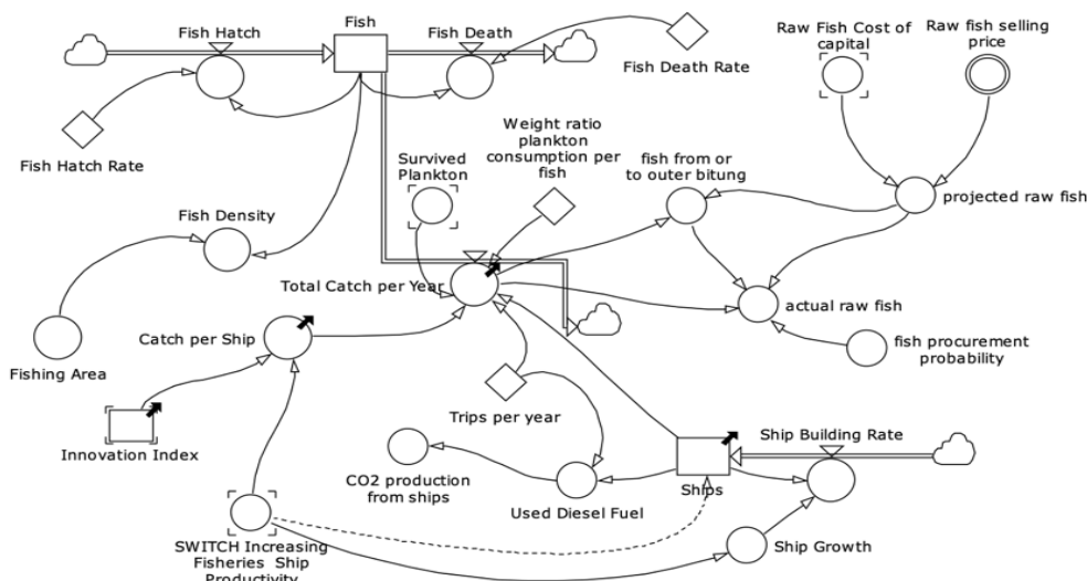
Figure 7 Stock and flow diagram of the fisheries submodule
