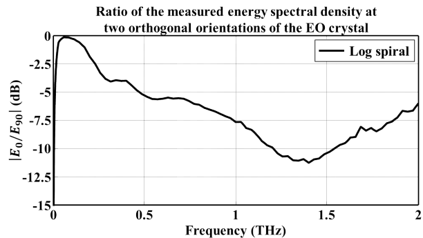
Figure 14. Ratio of two measured energy spectral densities amplitudes obtained by two orthogonal orientations of the EO crystal.
