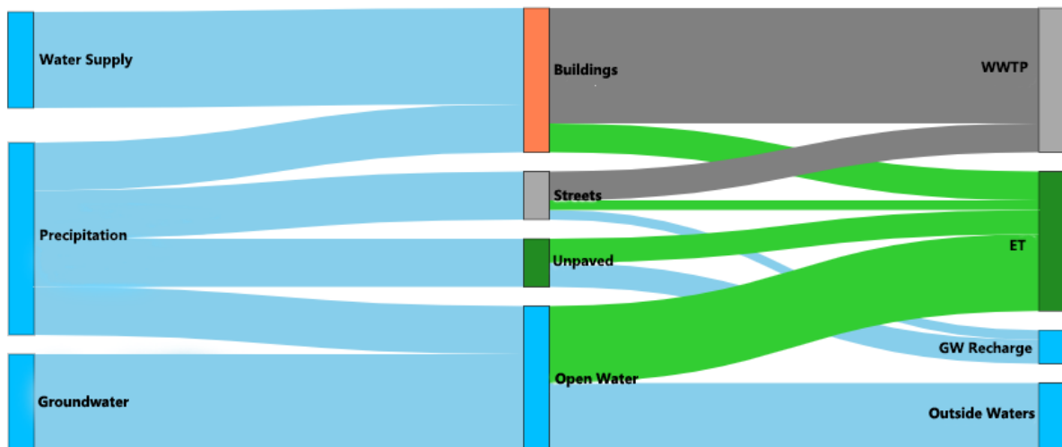
Figure 3.3: Sankey diagram of water balance
