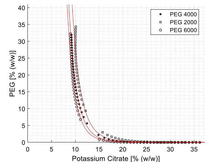
Fig. 14. FH model predicts the trend of decrease in monophasic region with increasing the polymer size. The w_{ij} ( w_j ) were fitted considering the system composed by PEG 4000 and according to the reconciliation approach (Method B, Table 1). The simulations were performed by varying the component size ( M and Mw ) of the polymer. R and T have the values of 8.3144 J/K/mol and 313.12 K, respectively.
