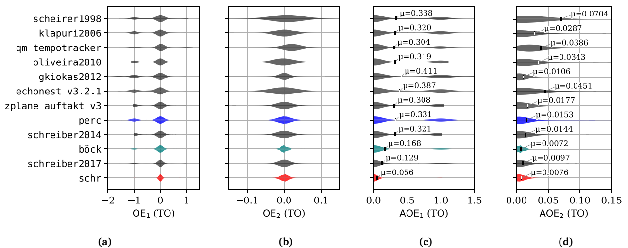
Figure 3: Empirical distributions of (a) OE_1 , (b) OE_2 , (c) AOE_1 , and (d) AOE_2 using kernel density estimation (KDE). Based on values measured for Ballroom using a median ICBI-derived ground truth created from beat annotations by Krebs et al. (2013). Ordered by year of publication (Scheirer, 1998; Klapuri et al., 2006; Davies et al., 2009; Oliveira et al., 2010; Gkiokas et al., 2012; Percival and Tzanetakis, 2014; Schreiber and Müller, 2014; Böck et al., 2015; Schreiber and Müller, 2017, 2018b). Estimates for zplane and echonest stem from Percival and Tzanetakis (2014).
