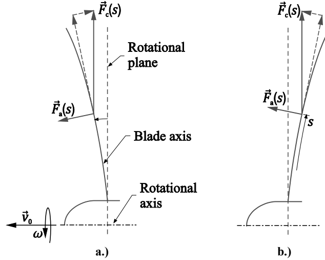
Figure 23: Leverage to centrifugal loads due to a.) positive coning, and b.) negative coning
