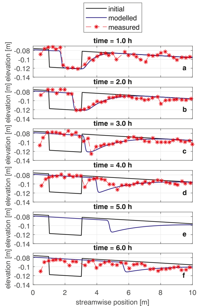
Fig. 7. Measured data and modelled results of the reference experiment (i.e., without a fixed layer) by Struiksmma (1999). No measurements where available at 5 h.
