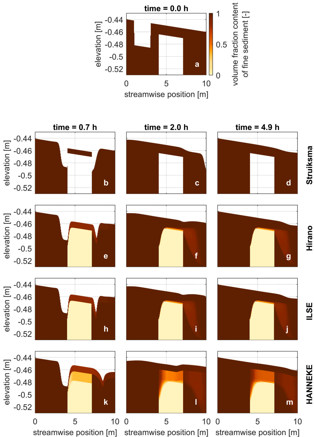
Fig. 11. Initial condition (a) and model results at different times (in columns) applying the model by Struikasma (top row), the model by Hirano (second row from above), the ILSE model (third row from above) and the HANNEKE model (fourth row from above) to a case in which all sediment is mobile.
