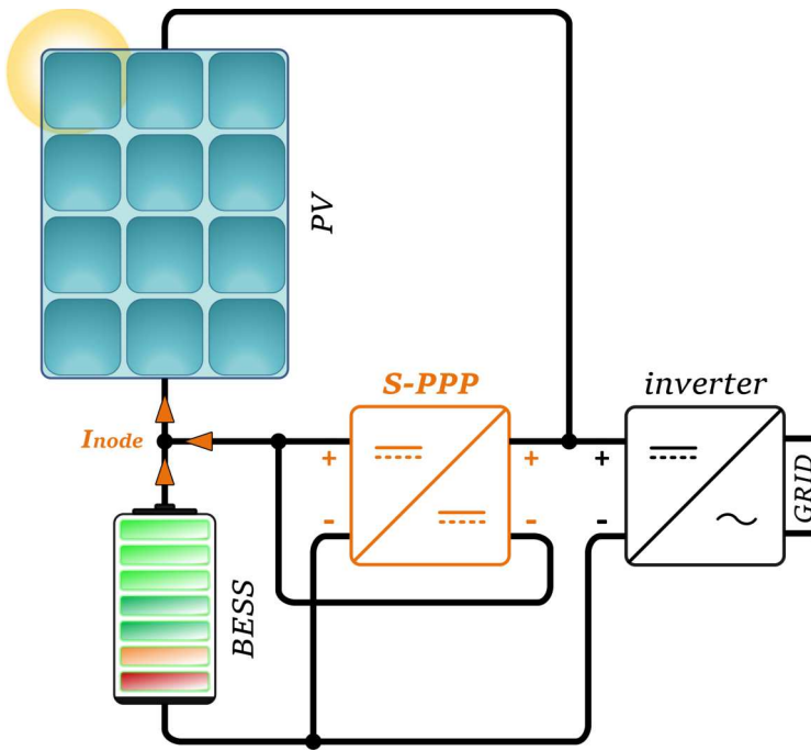
Fig. 1a): S-PPP converted applied to the PV-BESS series connection
