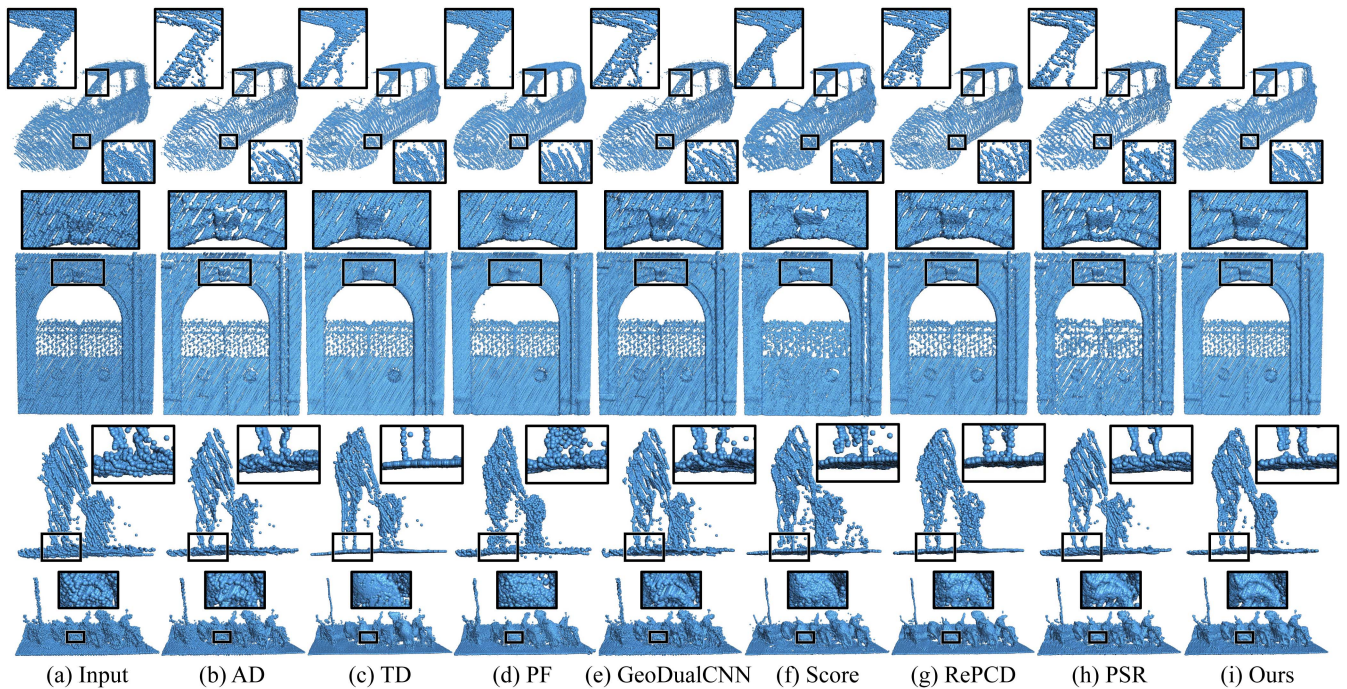
Fig. 7. Denoising real-scanned LiDAR data in Real-B . PathNet removes heavy noise and preserves geometry better (see the magnified parts) than its competitors.
