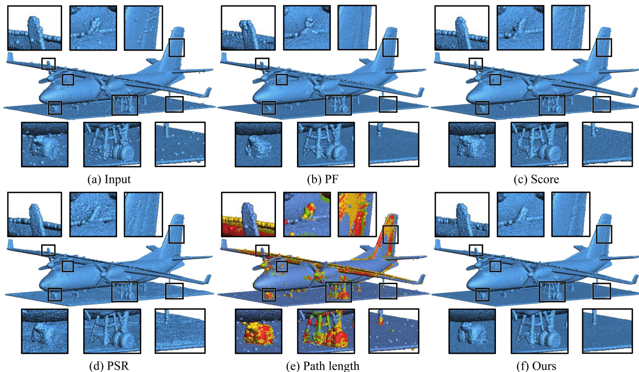
Fig. 9. Visualization of the real-scanned airplane data (246 K points) in Real-B and its denoising results. The airplane is scanned from multiple stations by a Leica RTC360. PathNet removes noise and preserves geometry better (see the magnified parts) than three state-of-the-art methods, namely PF [2], Score [7], and PSR [8].
