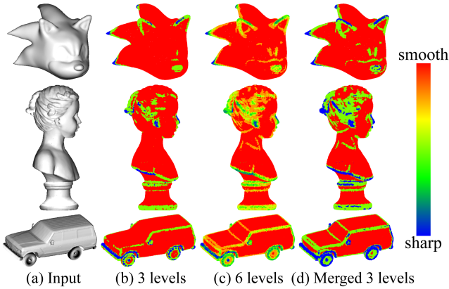
Fig. 6. Geometric feature levels (3 levels and 6 levels) of three 3 point clouds in the training dataset. (b) classifies all points into 3 levels directly, while (c) classifies all points into 6 levels. (d) merges 6 levels into 3 levels to balance the proportion of each level by merging the levels with low proportion but high similarity. The lower geometric feature levels (in blue) represent sharper regions. Compared with (b), (d) gives a higher level to the geometric feature area in the smooth region compared with (b), which avoids geometric smoothing in the smooth region while denoising.
