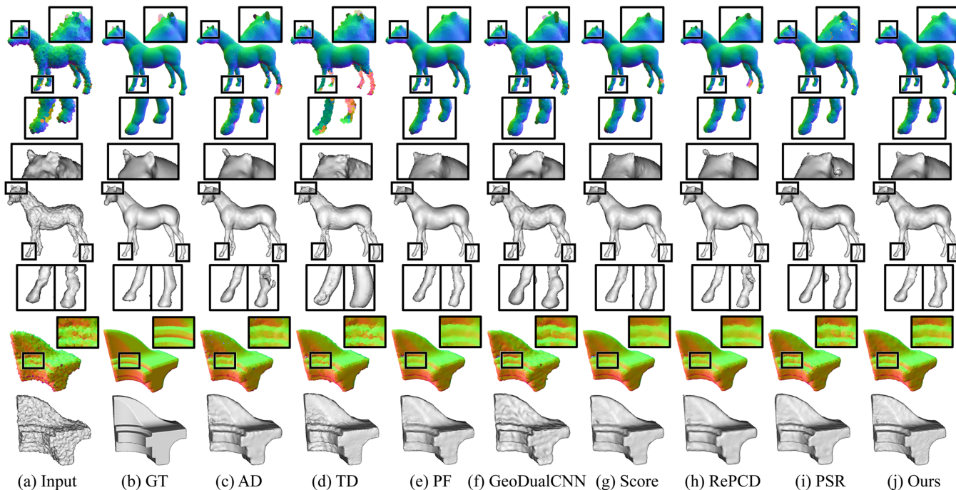
Fig. 10. Denoising synthetic point clouds in Synth-A . The noisy models are an animal and a CAD model corrupted by 1.0% and 1.5% Gaussian noise, respectively. PathNet outperforms the others in terms of both noise removal and feature preservation (see the close-up views). The colorful points are colored by their normals. The discontinuity in color indicates noise residuals (horse legs) that cause errors in the normals. The gray models are the meshes reconstructed by Poisson surface reconstruction.
