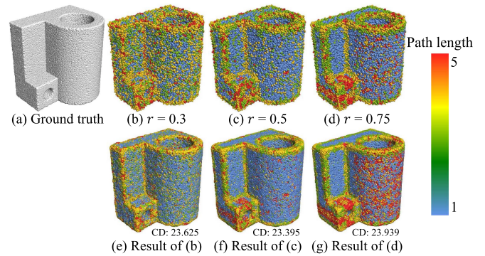
Fig. 13. Path selection visualization for a point cloud (1% noise and 50 K points) with different receptive fields. The two rows respectively demonstrate the input and output colored by the path length. The receptive fields from (b) to (d) are 0.3, 0.5, and 0.75, respectively. PathNet operates smoothly with these different receptive fields.
