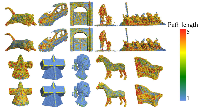
Fig. 11. Visualization of path lengths of ten models from Synth-A , Real-A , and Real-B datasets. The 1st and 3rd rows demonstrate the path lengths on the inputs. The 2nd and 4th rows are on the denoised outputs.
