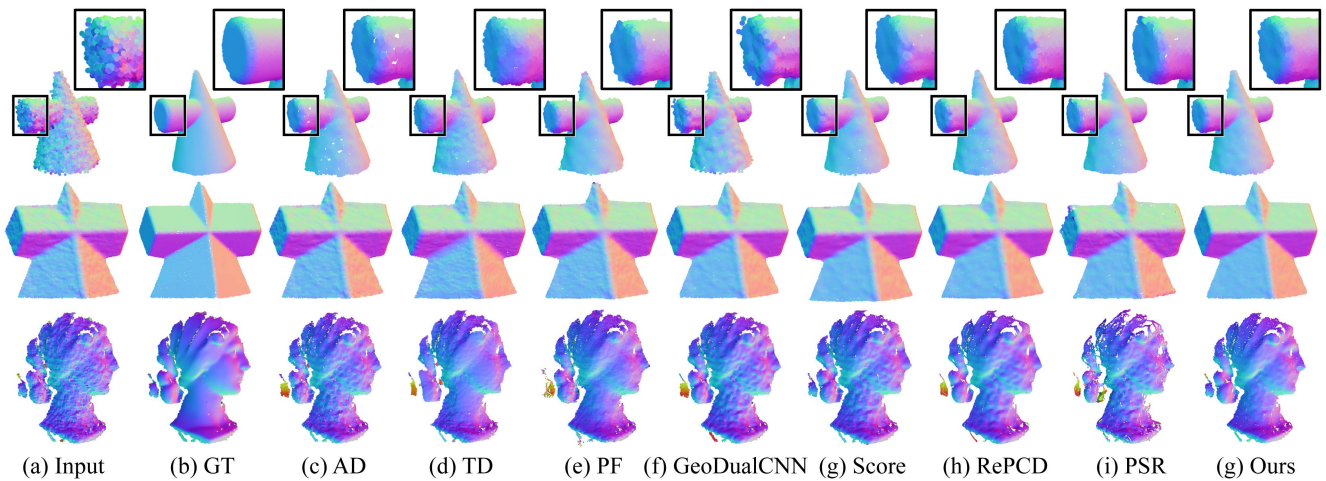
Fig. 8. Denoising real-scanned Kinect data in Real-A . The models in the first two rows are obtained by fusing scans from multiple views, and the one in the bottom row is a single-view point cloud. PathNet outperforms the others in terms of both noise removal and feature preservation. The points are colored by their normals calculated using the same algorithm.
