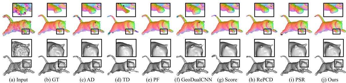
Fig. 2. Visual comparisons of the denoising results of our method (j) against state-of-the-art methods (c-i) including AD [4], TD [5], PF [2], GeoDualCNN [6], Score [7], RePCD [3] and PSR [8]. The input data is corrupted by 1.0% Gaussian noise. Our method outperforms the others in terms of both noise removal and feature preservation (see particularly the close-up views). The colorful points are colored by their normals calculated using the same algorithm. The discontinuity in color indicates noise residuals (legs) that cause errors in the normals. The gray models are the meshes reconstructed by Poisson surface reconstruction.
