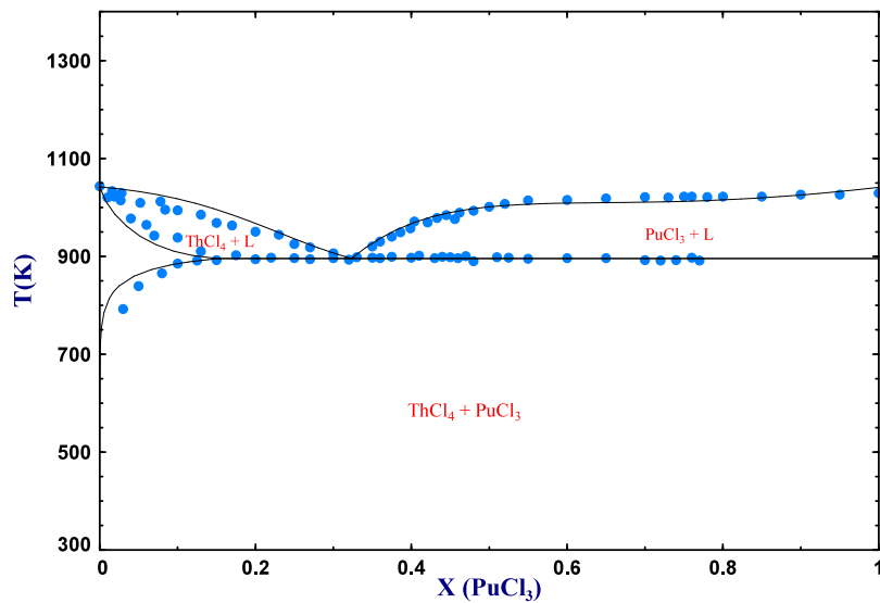
Fig. 3. Phase diagram of the ThCl 4 -PuCl 3 system modeled in this work. (●) Data from Vorobei et al. [8].
