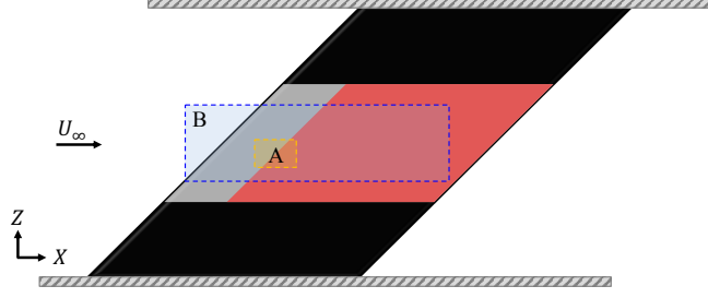
Fig. 7 Schematic of IR imaging, showing a side view of the M3J model indicating the locaiton of the final analysis region for camera (A) and camera (B).
