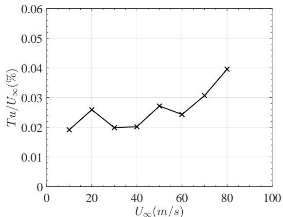
Fig. 5 Low Turbulence Tunnel (LTT) measured turbulence intensity with M3J model installed in the test-section.
