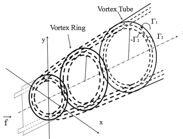
Figure 1. Scheme of the vortex model. The wake consists of vortex rings for the near wake and semi-infinite vortex tubes for the far wake. Vortex shed at the edge and positions where there is a pressure jump.
