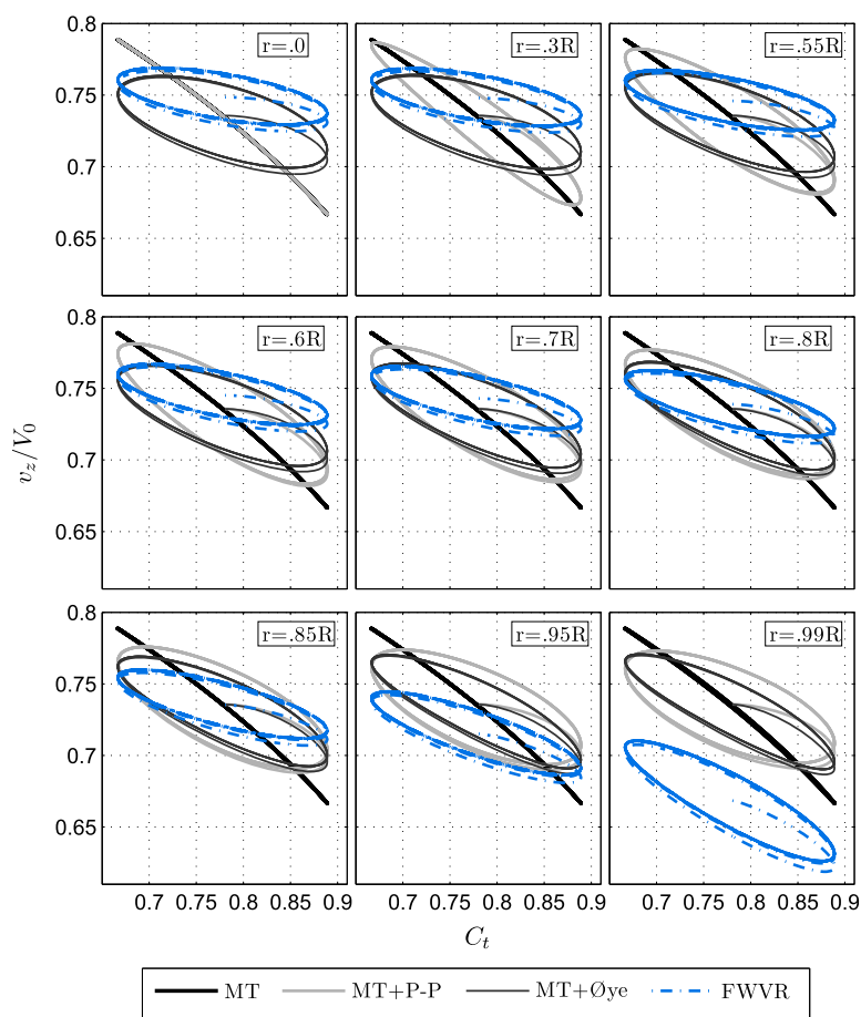
Figure 9. Comparison of hysteresis loops of the axial velocity at different radii between the FWVR model, Momentum Theory and the \text{\O} ye and Pitt-Peters model for Case II (2) for k = 0.2 .
