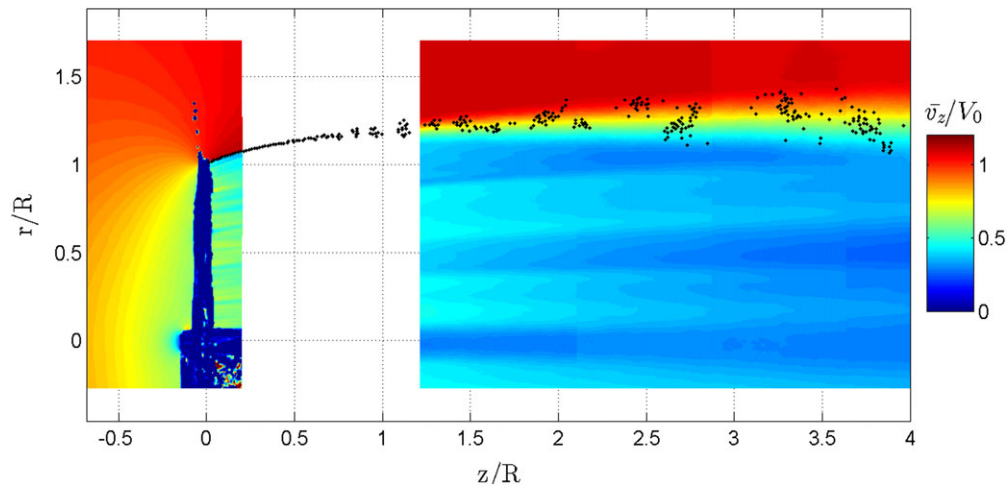
Figure B1. Comparison between positions of vortex rings from the FWVR model and time averaged velocity field from the wind tunnel measurements of an actuator disc for C_t = 0.93 . Black points represent intersections of the vortex rings with the symmetry plane
