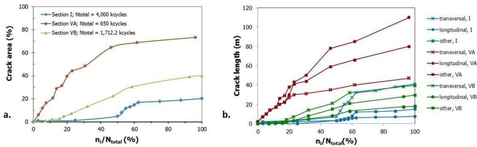
Fig. 2. (a) Development of the percentage cracked area on Lintrack sections I, VA, VB based on 100x100 grid size area (b) Development of crack length observed on Lintrack sections I, VA and VB (Pramesti [7] based on Groenendijk[1, 4] data)
