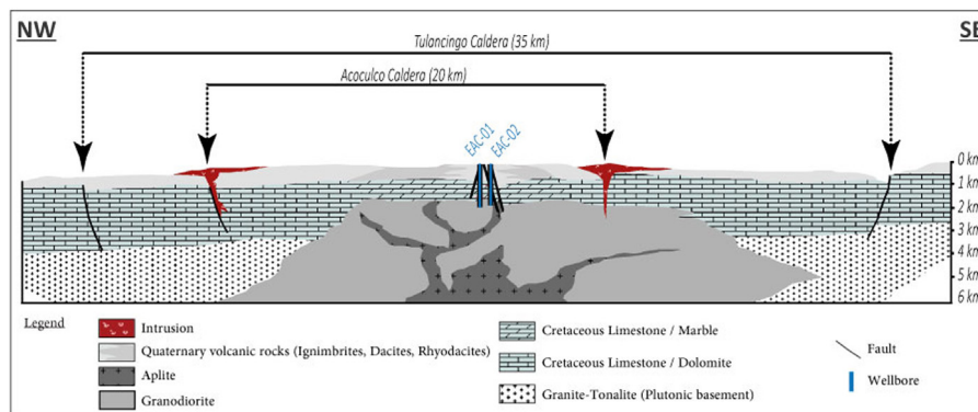
Fig. 7. Schematic geological section of the Tulancingo–Acoculco caldera Complex, modified from López-Hernández et al. (2009).
