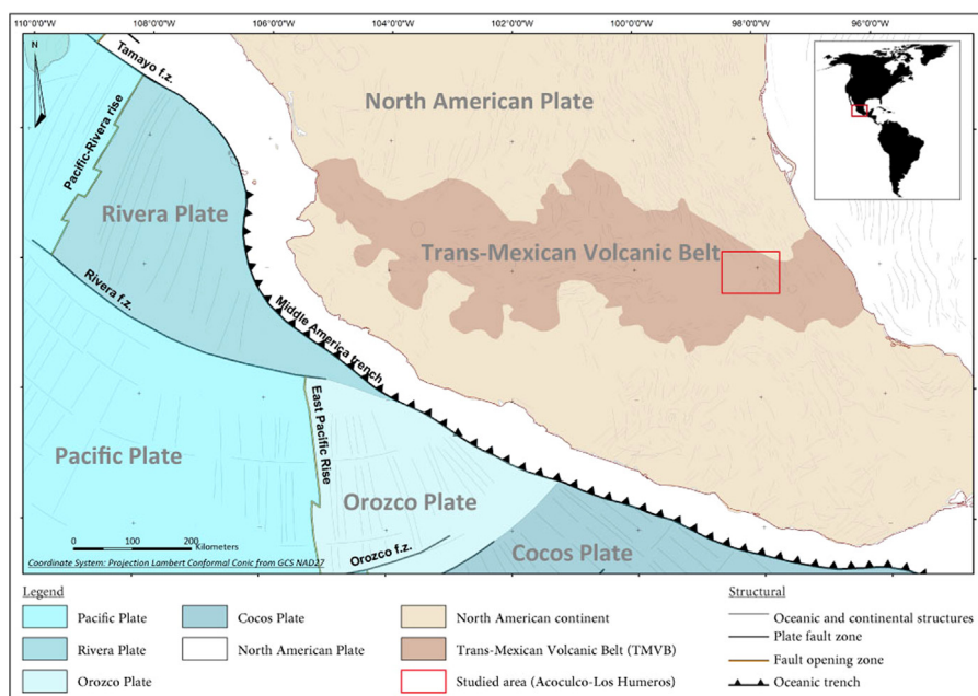
Fig. 6. Simplified tectonic map of Mexico, indicating Acoculco site location, modified from Padilla (2013).
