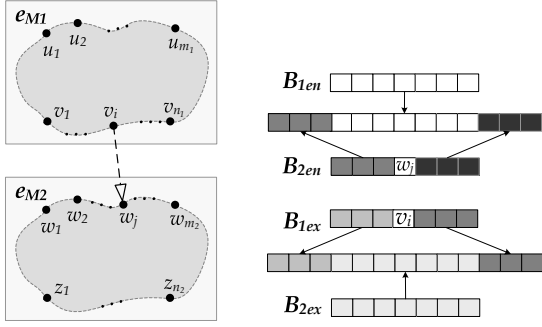
Figure 17: Merge two misc composites e_{M1} and e_{M1} connected by a path (v_i, w_j)
