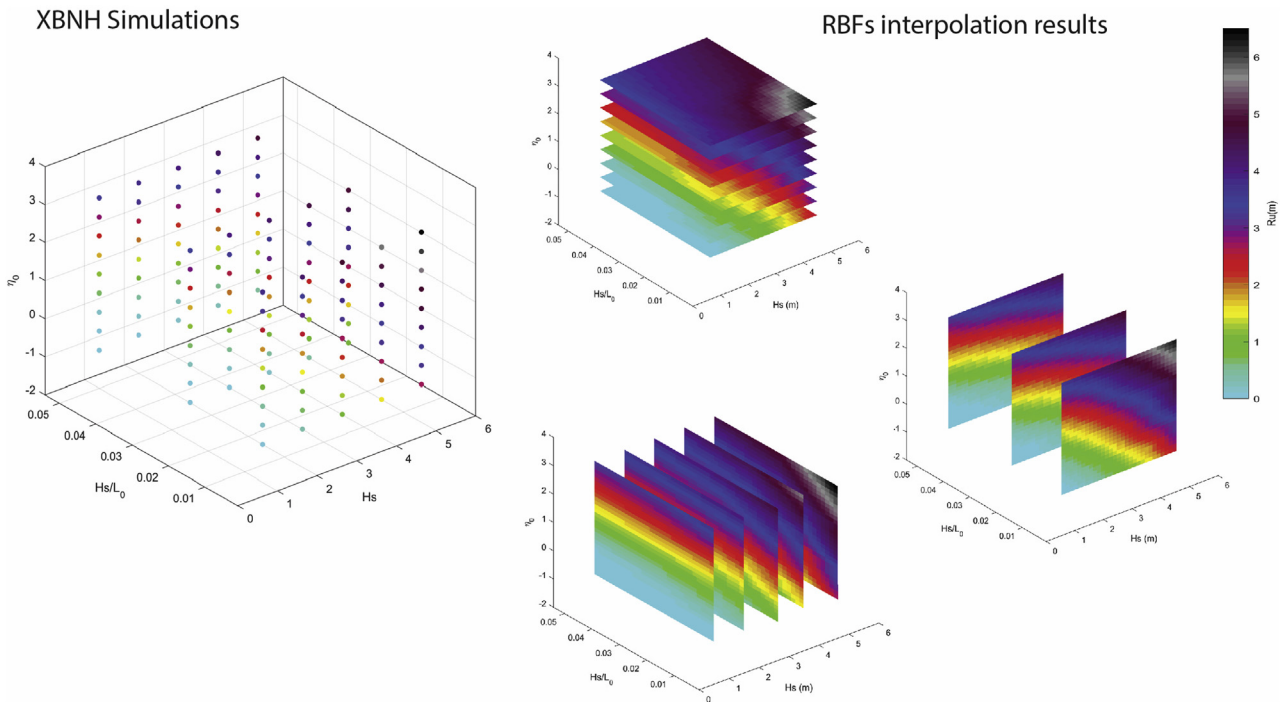
Fig. 2. Example fixing four of the parameters ( \beta_f = 0.1 , W_{reef} = 300 m, \beta_b = 0.1 , and c_f = 0.05 ). The left panel shows the represents the three-dimensional matrix of XBNH simulations and the right panel shows three different slices of the response function fixing one of the variables in each plot ( R_{2\%} = f(H_s, H_s/L_0 | \eta_0) , R_{2\%} = f(H_s, \eta_0 | H_s/L_0) , and R_{2\%} = f(H_s/L_0, \eta_0 | H_s) ).
