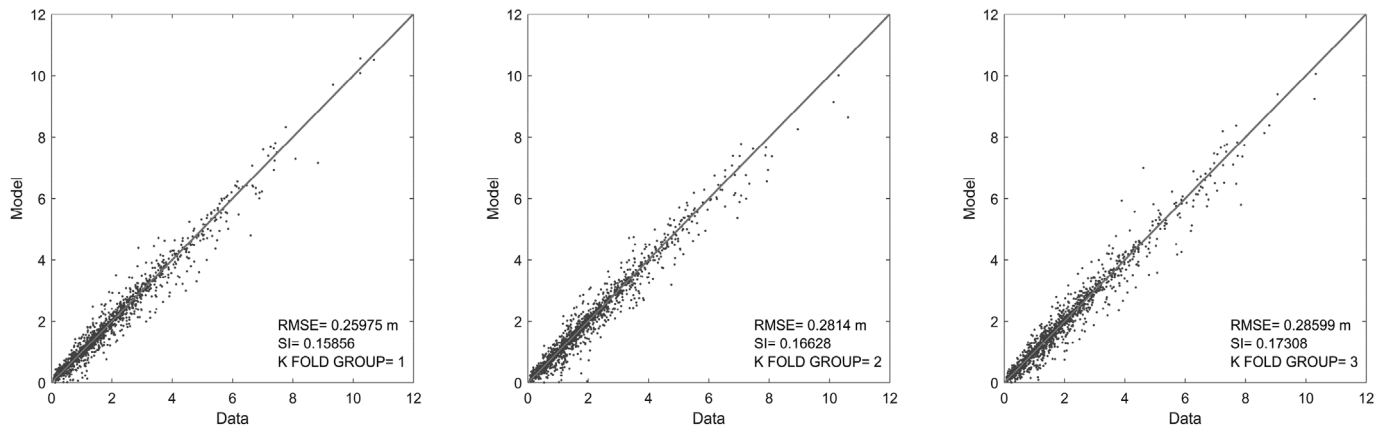
Fig. 3. Example k -fold model-data validation for the first three sub-datasets. Comparison between run-up values ( R_{2\%} , in meters) from XBNH simulations (x-axis) and meta-model (y-axis).
