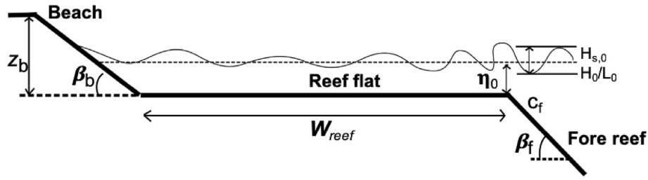
Fig. 1. Idealized reef profile and defined hydrodynamic and morphologic parameters, adapted from Pearson et al. (2017).
