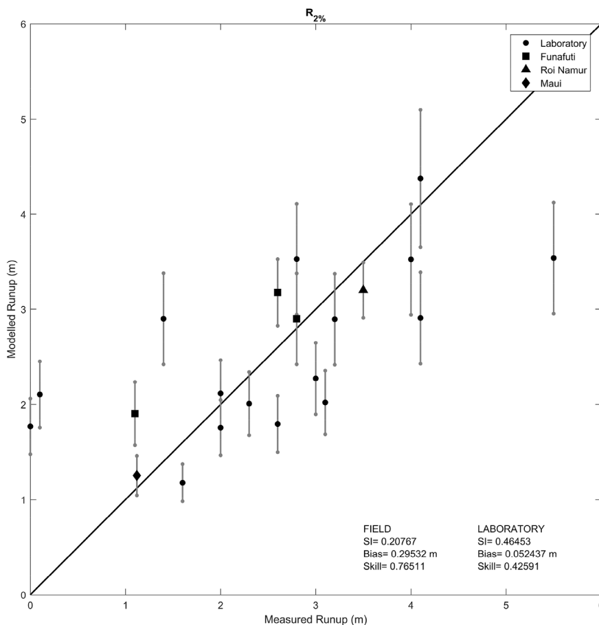
Fig. 4. Validation of HyCReWW model.
