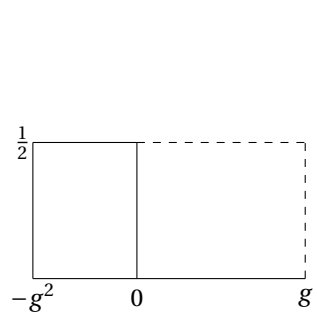
Figure 3.3: \Omega_g
