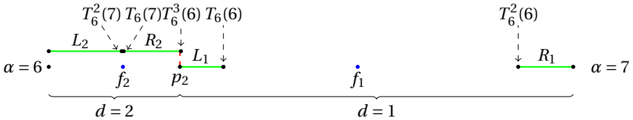
Figure 4.4: N = 50, \alpha = 6
