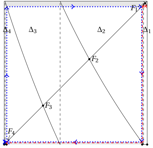
N = 11, \alpha = 1.8687 \dots (k = 2, i = 1) T_\alpha^3(\alpha) = T_\alpha(\alpha)
