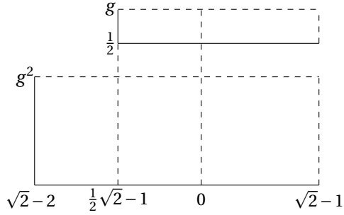
Figure 3.10: \Omega_{\sqrt{2}-1}
