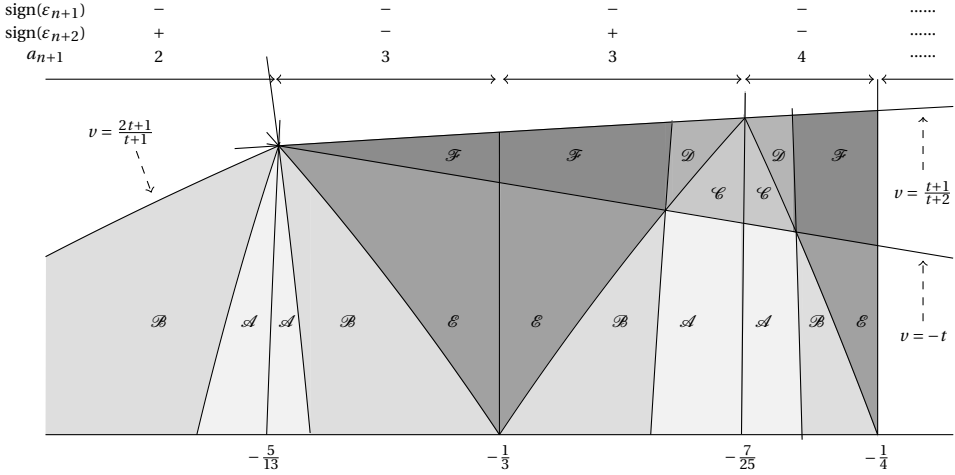
Figure 2.8: The six patterns for \varepsilon_{n+1} = -1
