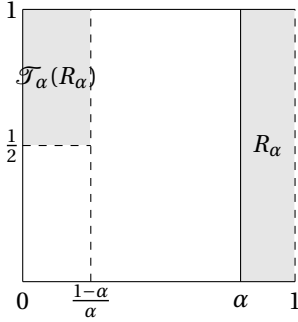
Figure 3.1: \Omega_1, \alpha = 0.8
