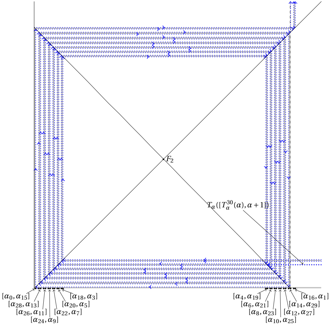
Figure 4.28: N = 10,000 ; \alpha = 98.9995 bottom left. The notation \alpha_i is short for T_\alpha^i(\alpha) . The small gaps and the large gap in \Delta_2 are visible as well as the leftmost, small gap of \Delta_1 and part of the large gap containing f_1 . Not visible is the one gap remaining, the one between T_\alpha^{17}(\alpha) and T_\alpha^{30}(\alpha) .
