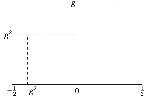
Figure 3.8: \Omega_{\frac{1}{2}}
