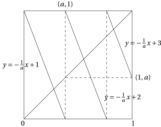
Figure 4.16: The ‘limit graph’ of T_\alpha , translated over (-\alpha, -\alpha) , under the conditions I_\alpha = \Delta_d \cup \Delta_{d-1} \Delta_{d-2} and N/(\alpha + 1) - (d - 2) = p_d for N \rightarrow \infty (and \alpha, d \rightarrow \infty accordingly)
