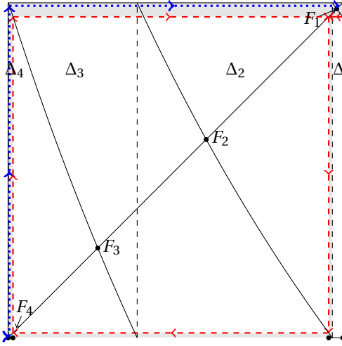
N = 11, \alpha = 1.8719 \dots (k = 2, i = 1) T_\alpha^3(\alpha + 1) = T_\alpha(\alpha + 1)
