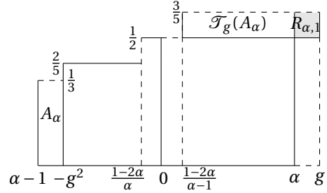
Figure 3.5: \Omega_{\alpha,1}^+ , \alpha = 0.52
