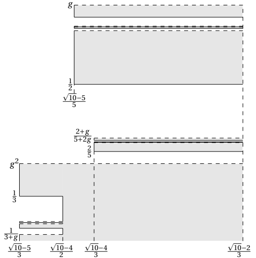
Figure 3.17: \Omega_{\frac{\sqrt{10}-2}{3}} , 'rough sketch'.
