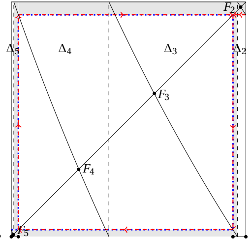
N = 21, \alpha = 2.7123 \alpha_l = 2.7122 \dots and \alpha_u = 2.7123 \dots
