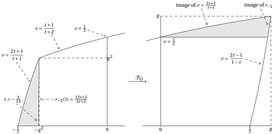
Figure 2.5: The map of the leftmost corner applying \mathcal{F}_O
