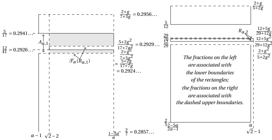
Figure 3.14: The leftmost corner of \Omega_{\alpha,2}, \alpha = 0.405 .
