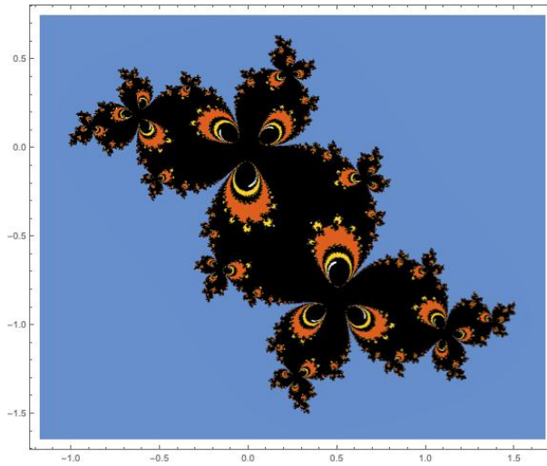
Figure 5.1: Julia Set
