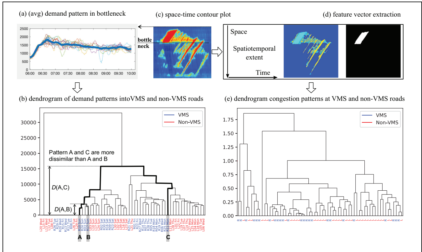
Figure 4. Methods and clustering results for hypothesis 1. (For an explanation of the subfigures see running text.) Note: VMS = variable message signs.
