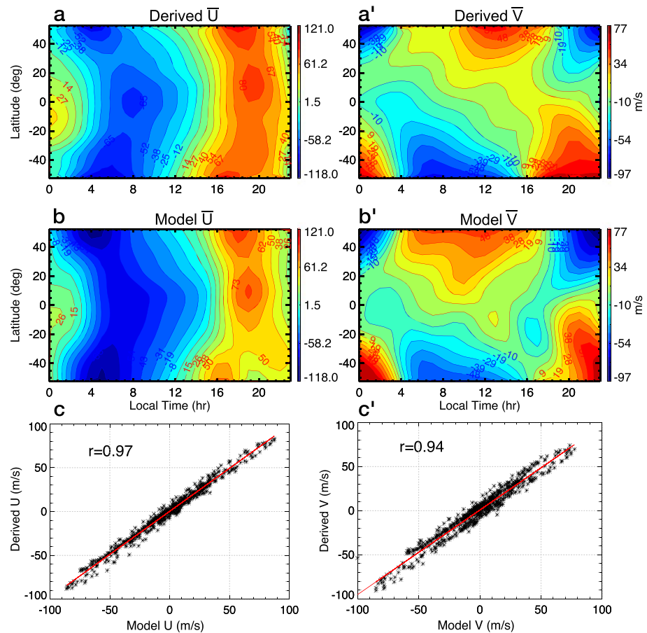
Figure 3. Latitude versus local time comparison between (a) synthetic and (b) model zonal winds (longitudinal mean, \bar{U} ), and a' derived and b' model meridional wind (longitudinal mean, \bar{V} ). (c (c')) The scatter plot between synthetic zonal (meridional) winds and model zonal (meridional) winds. The TIME-GCM run used is the same as in Figures 1 and 2. Note correlation coefficients of \sim 0.97 ( \sim 0.94 ) for zonal (meridional) winds. The minimum in model meridional winds at 10\text{--}30^\circ\text{S} around 16–18 LT not captured by the derived winds is likely due to increased pressure gradient and/or ion drag retrieval errors around sunset for relatively low wind speeds ( \pm 15 m/s).
