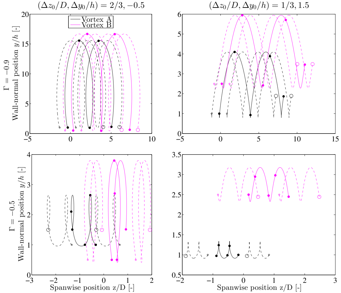
Figure 6: Trajectories for \Gamma = -0.9 ( top ) and \Gamma = -0.5 ( bottom ). Different initial conditions (\Delta z_0/D, \Delta y_0/h) are prescribed: 2/3, -0.5 ( left ) and 1/3, 1.5 ( right ). Filled markers and solid lines represent the base vortices; empty markers and dashed lines represent their periodic images. Markers are spaced at 0.25\mathcal{T} . Trajectories for \Gamma = -0.9 and -0.5 are shown for a total time 20L/U and 5L/U .
