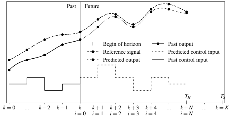
Fig. 4 Schematic representation of the offline MPC algorithm.
