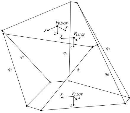
Fig. 3 Schematic hexapod system.
