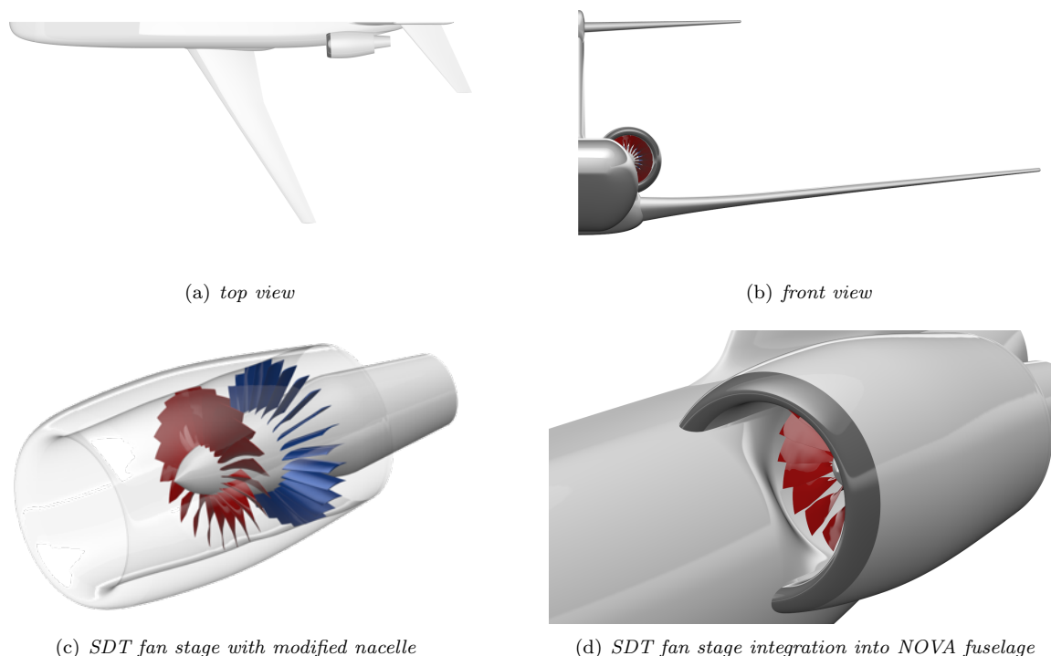
Figure 1. NOVA aircraft configuration equipped with the redesigned BLI engine nacelle.
