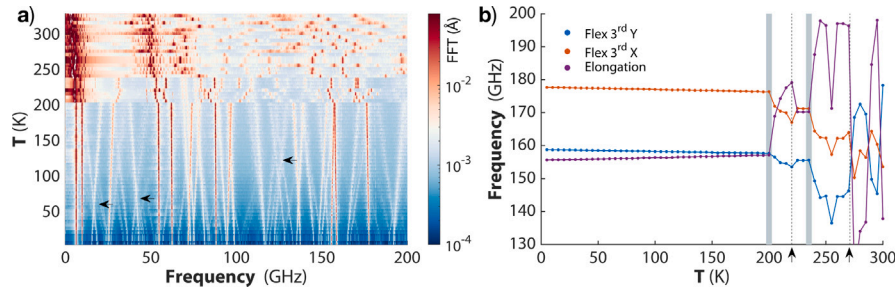
Fig. 4. Internal resonance of higher modes. (a) Density plot of the spectrum showing the thermal shift of the eigenfrequencies. (b) Detailed evolution of the two third flexural and the first longitudinal mode. Region of coinciding eigenfrequencies are highlighted with a grey background. The arrows indicate sudden variation of the flexural modes. (For interpretation of the references to color in this figure legend, the reader is referred to the web version of this article.)
