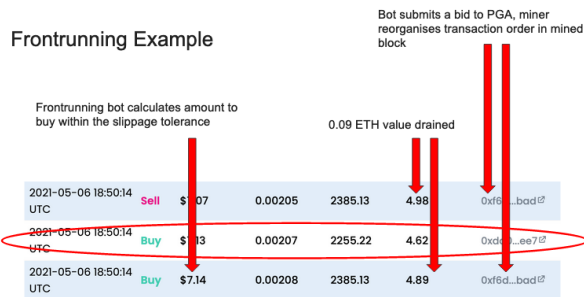
Figure 6: Sandwich attack that drained 0.09 ETH, shown on ChartEx
