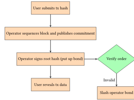
Figure 9: Commit-reveal scheme to prevent transaction-reordering for optimistic rollups. [26]
