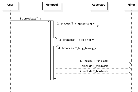
Figure 7: A sequence diagram illustrating how adversaries guarantee transaction order by exploiting Geth’s default transaction ordering algorithm.
