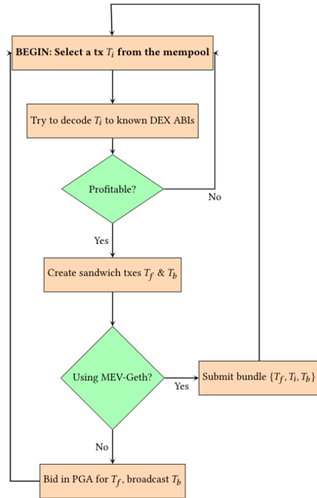
Figure 4: Flowchart of an example specialized frontrunner that targets DEX trades, which extracts profits by taking advantage of the victim’s slippage tolerance. Among them, ABIs and PGA are Solidity Contract Application Binary Interface: https://docs.soliditylang.org/en/v0.8.7/abi-spec.html and Priority Gas Auctions respectively
