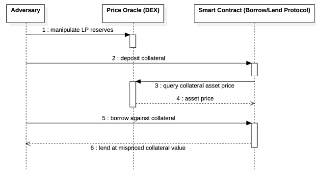
Figure 10: A sequence diagram depicting an example of an oracle manipulation exploit; involving an adversary, and a lending/borrowing smart contract to be arbitrated which queries an on-chain price oracle.
