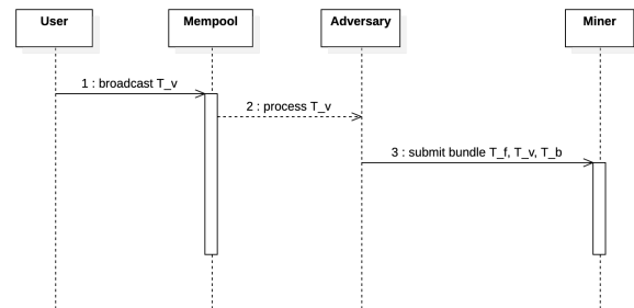
Figure 8: A sequence diagram illustrating how adversaries guarantee transaction order by participating in sealed-bid auctions to compete for block space.
