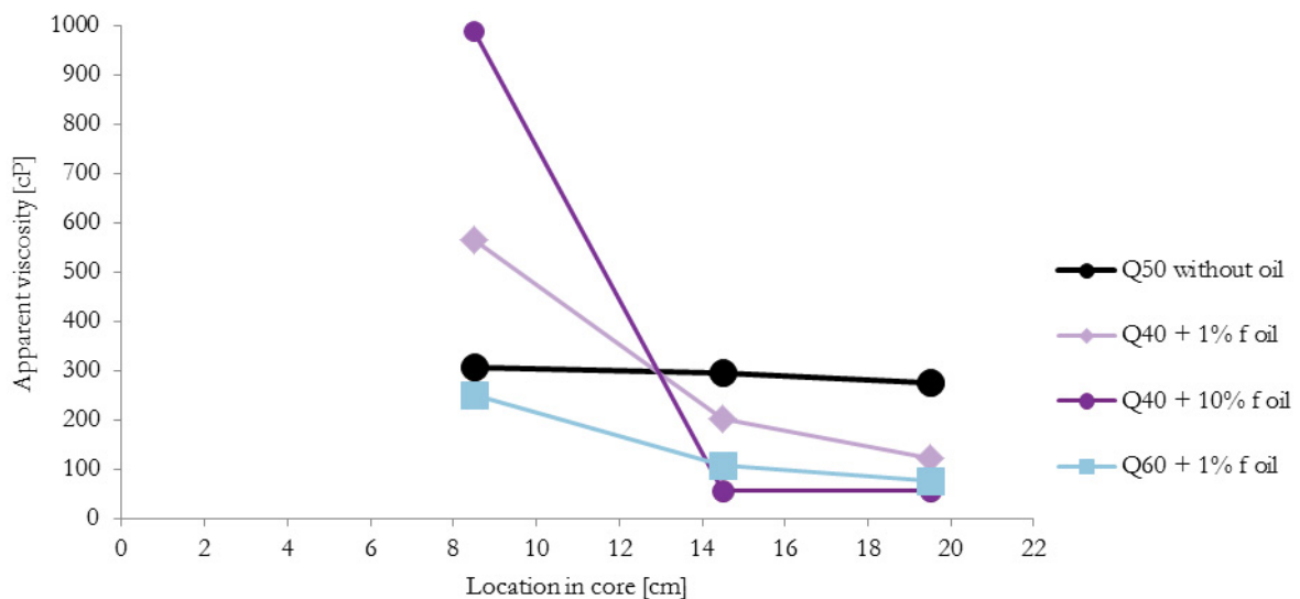
Figure 5 Apparent viscosity of pre-generated foam with surfactant A and oil over the length of the core. Q50: 50% foam quality, etc. f: fractional flow of oil in injected fluids.
