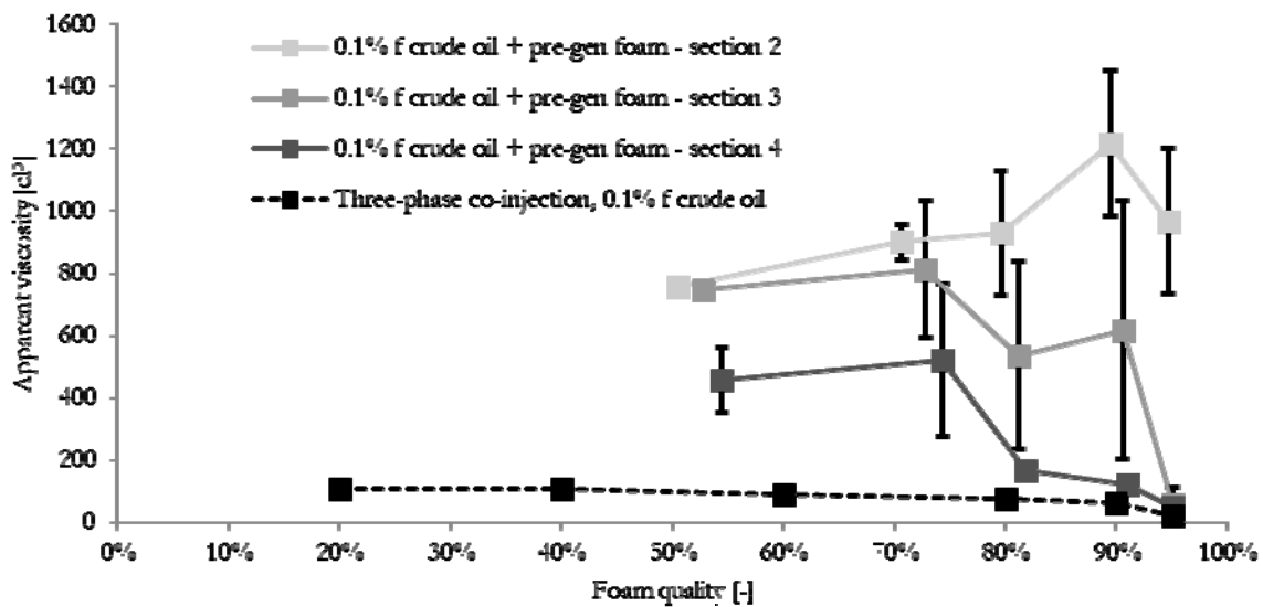
Figure 3 Apparent viscosity as a function of foam quality for pre-generated foam in contact with oil in different sections of the core, compared to three-phase co-injection. 0.1% f crude oil: 0.1% injected fractional flow of crude oil.
