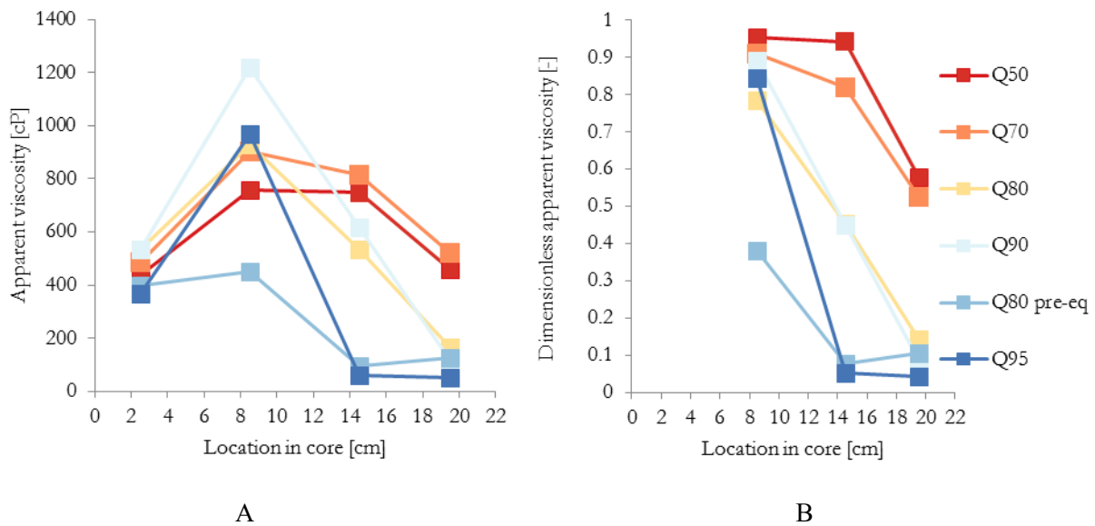
Figure 2 Left: apparent viscosity [cP] over the length of the core for different foam qualities with AOS. Right: dimensionless apparent viscosity [-] over the length of the core for the same experiments. All experiments were conducted with 0.1% oil fractional-flow. Q50: 50% foam quality, etc. Pre-eq: surfactant solution pre-equilibrated with oil.
