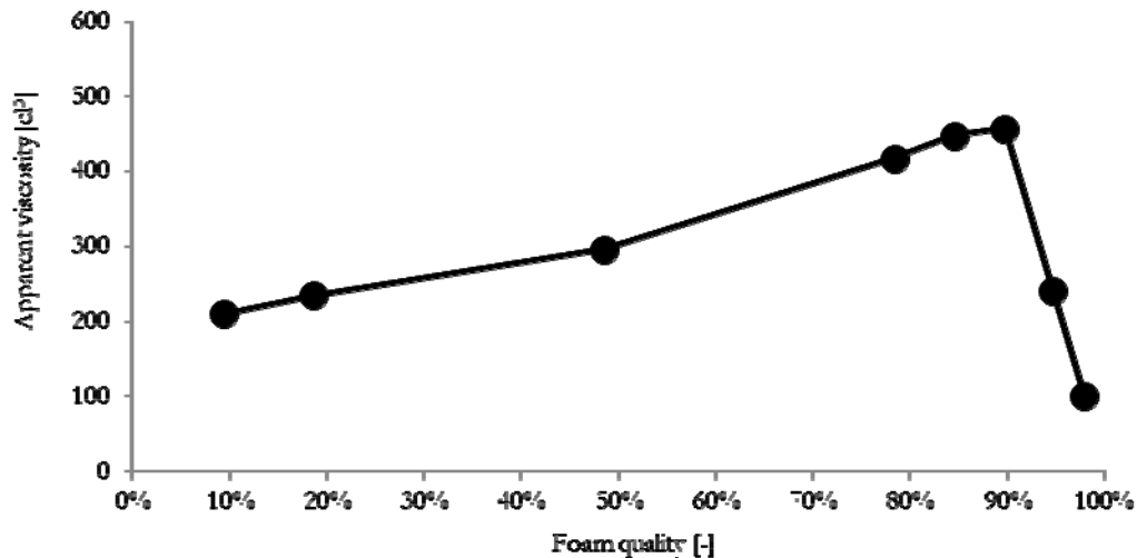
Figure 4 Surfactant-A foam apparent viscosity as a function of foam quality, in the absence of oil, in the third section of the core.
