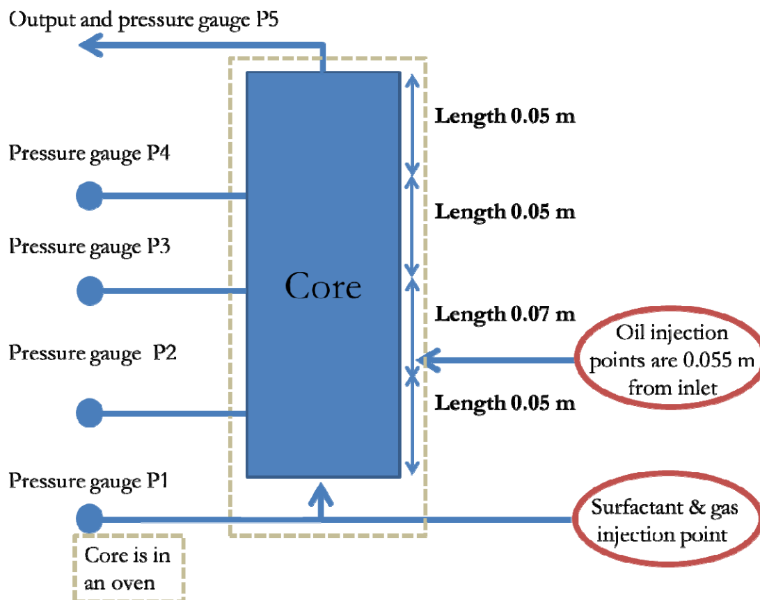
Figure 1 Schematic of the apparatus used for this experiment. Note that there are two oil-injection points 0.055 m from the main inlet on opposite sides of the core. (Only one is shown here to avoid clutter.)
