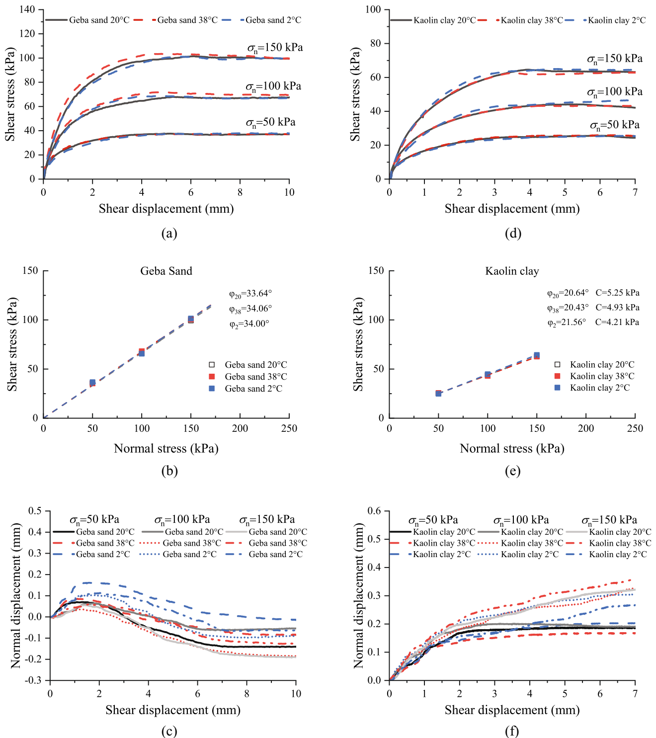
Fig. 8 CNL results for soil samples at T = 2, 20, 38 °C. Geba sand: a shear stress vs. shear displacement; b failure envelopes; c normal displacement vs. shear displacement; kaolin clay: d shear stress vs. shear displacement; e failure envelopes; f normal displacement vs. shear displacement
